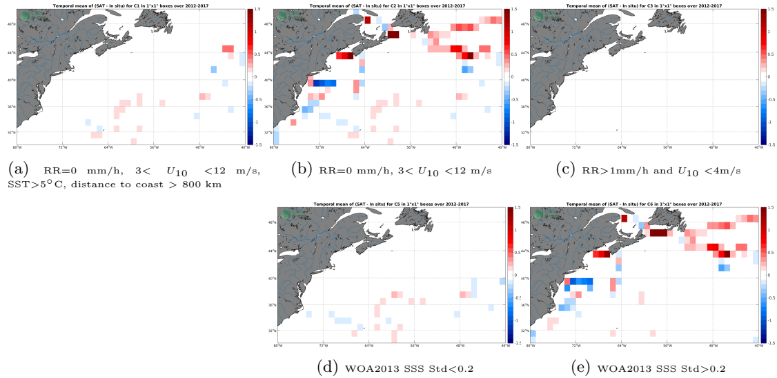
Figure 12: Temporal mean gridded over spatial boxes of size 1^\circ \times 1^\circ of \Delta SSS (CCI SSS L4 Merged-OI v2.31 - 30-day running (ESA) - TSG (GOSUD-Sailing-ship)) for 5 different subdatasets corresponding to:RR=0 mm/h, 3 < U_{10} < 12 m/s, SST >5^\circ\text{C} , distance to coast > 800 km (a), RR=0 mm/h, 3 < U_{10} < 12 m/s (b), RR >1 mm/h and U_{10} < 4 m/s (c), WOA2013 SSS Std <0.2 (d), WOA2013 SSS Std >0.2 (e).
