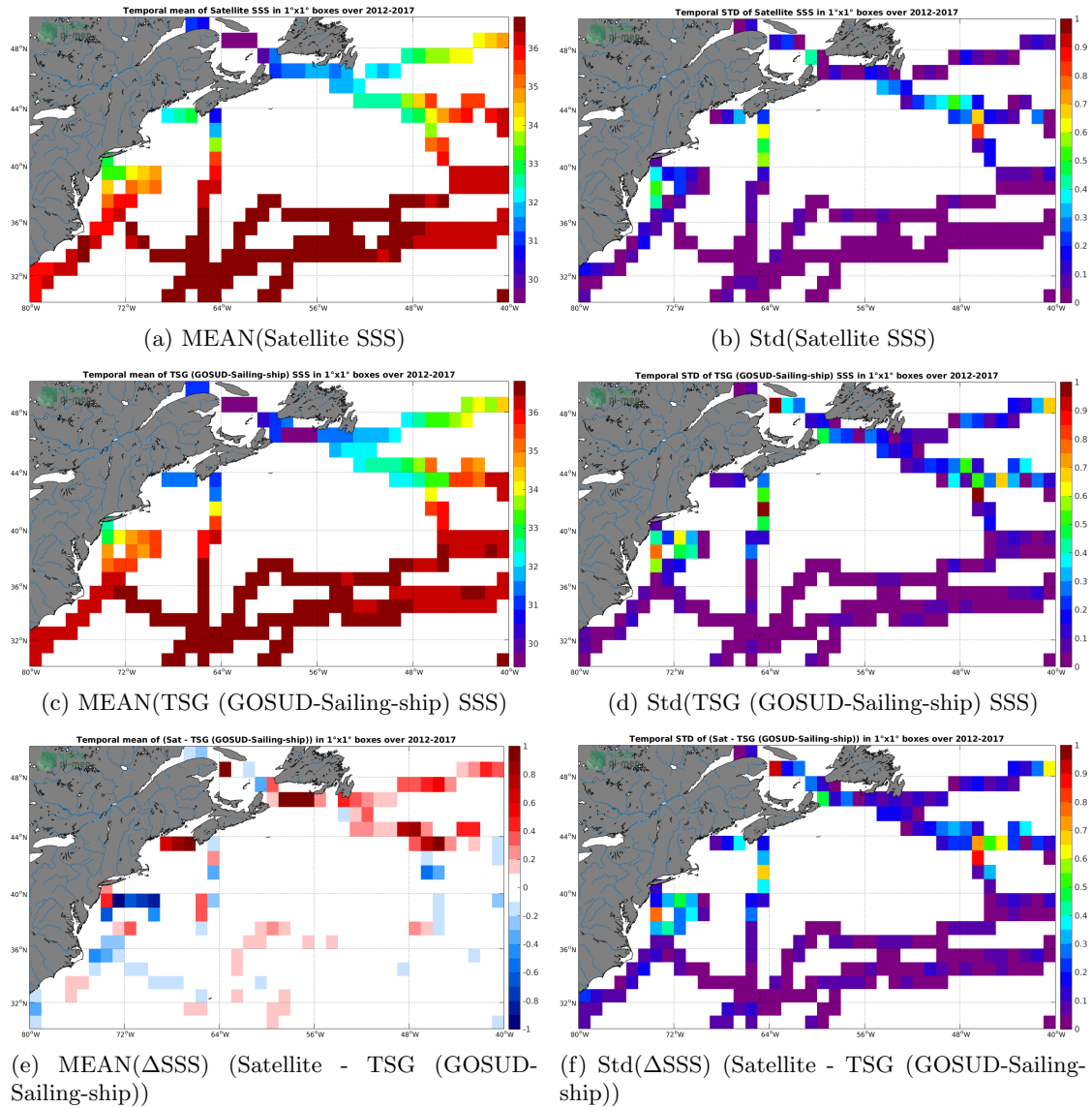
Figure 6: Temporal mean (left) and Std (right) of SSS from CCI SSS L4 Merged-OI v2.31 - 30-day running (ESA) (top), TSG (GOSUD-Sailing-ship) (middle), and of \Delta SSS (Satellite - TSG (GOSUD-Sailing-ship)). Only match-up pairs are used to generate these maps.
