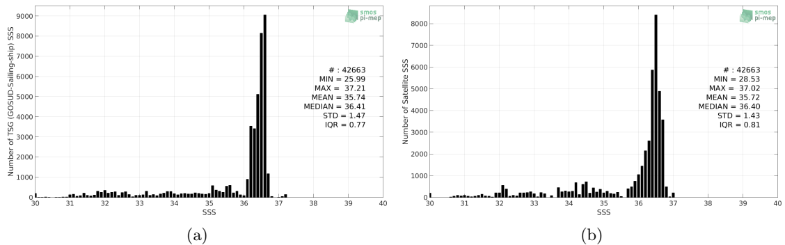
Figure 2: Histograms of SSS from TSG (GOSUD-Sailing-ship) (a) and CCI SSS L4 Merged-OI v2.31 - 30-day running (ESA) (b) considering all match-up pairs per bins of 0.1 over the Gulf Stream Pi-MEP region and for the full satellite product period.
