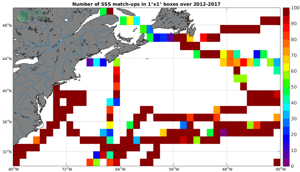
Figure 4: Number of SSS match-ups between TSG (GOSUD-Sailing-ship) SSS and the CCI SSS L4 Merged-OI v2.31 - 30-day running (ESA) SSS product for the Gulf Stream Pi-MEP region over 1^\circ \times 1^\circ boxes and for the full satellite product period.
