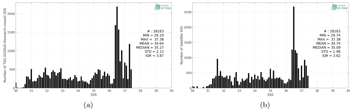
Figure 2: Histograms of SSS from TSG (GOSUD-Research-vessel) (a) and CCI SSS L4 Merged-OI v2.31 - 30-day running (ESA) (b) considering all match-up pairs per bins of 0.1 over the Gulf Stream Pi-MEP region and for the full satellite product period.
