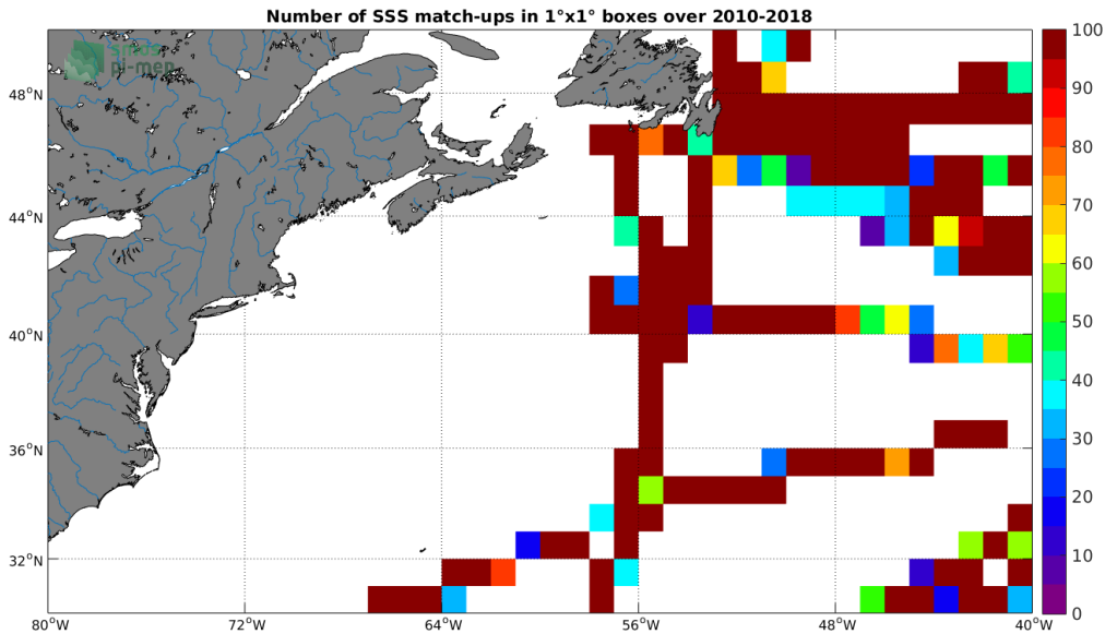
Figure 4: Number of SSS match-ups between TSG (GOSUD-Research-vessel) SSS and the CCI SSS L4 Merged-OI v2.31 - 30-day running (ESA) SSS product for the Gulf Stream Pi-MEP region over 1^\circ \times 1^\circ boxes and for the full satellite product period.
