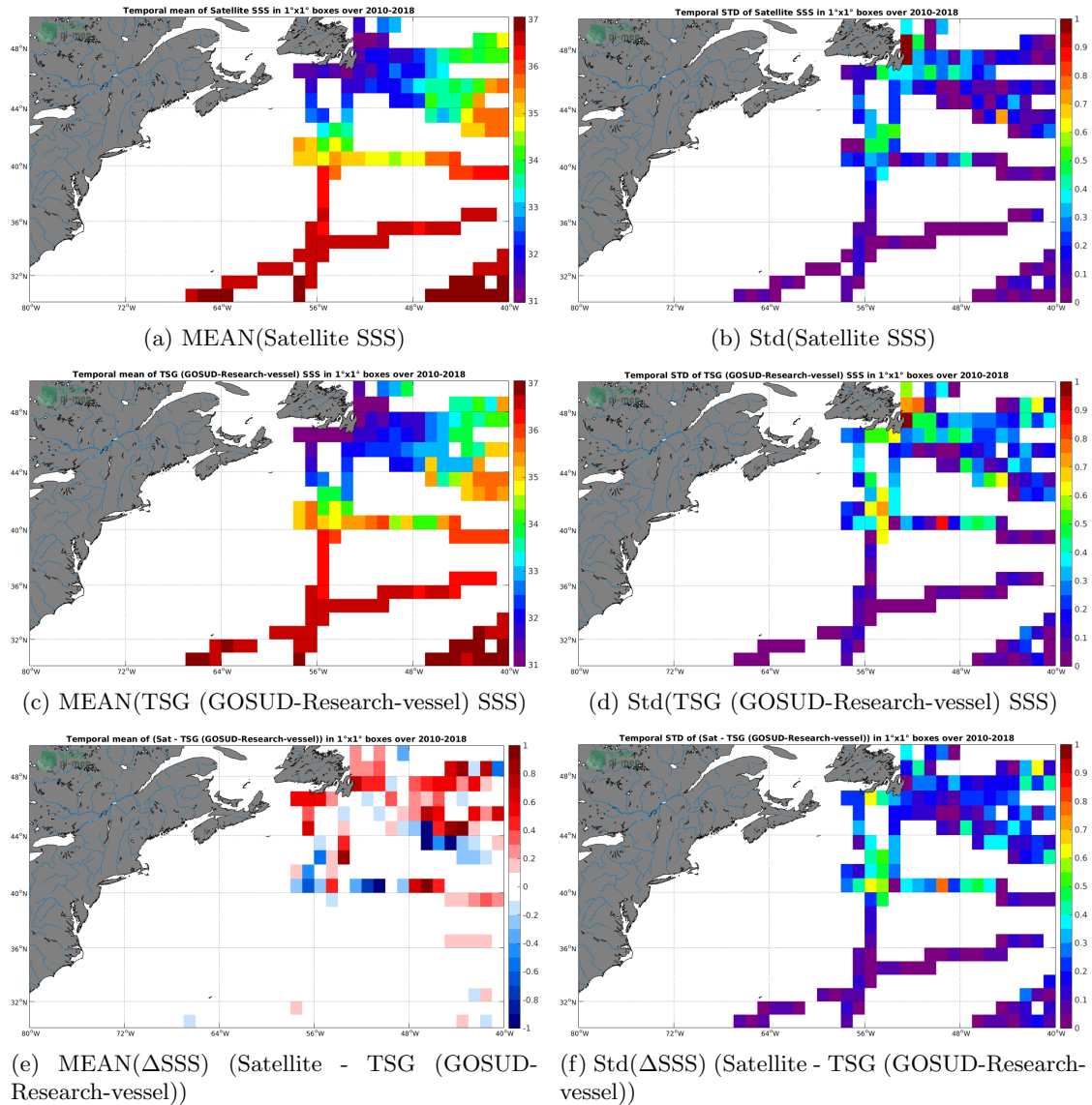
Figure 6: Temporal mean (left) and Std (right) of SSS from CCI SSS L4 Merged-OI v2.31 - 30-day running (ESA) (top), TSG (GOSUD-Research-vessel) (middle), and of \Delta SSS (Satellite - TSG (GOSUD-Research-vessel)). Only match-up pairs are used to generate these maps.
