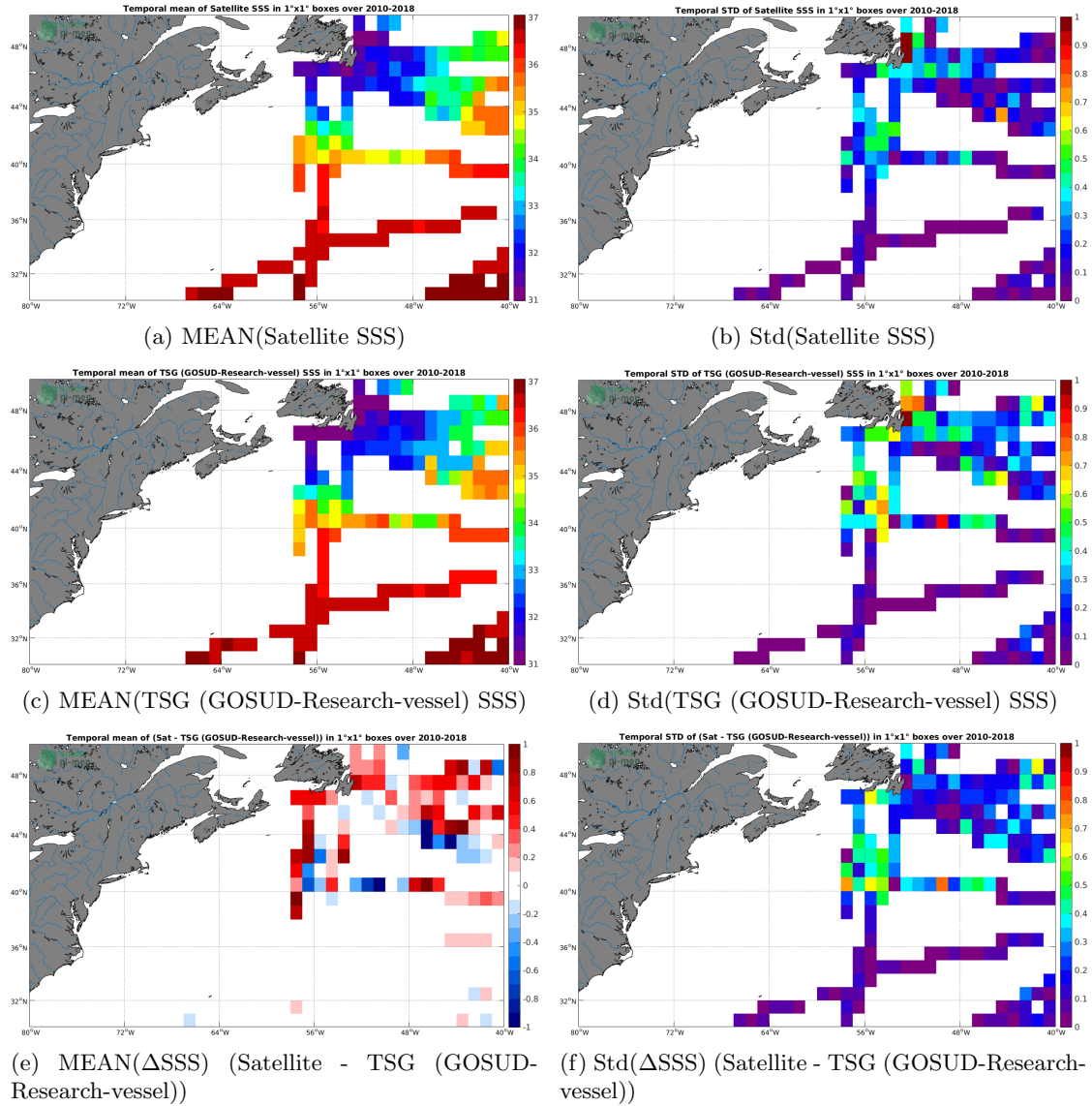
Figure 6: Temporal mean (left) and Std (right) of SSS from CCI L4 Merged-OI v2.31 - 30-day running (ESA) (top), TSG (GOSUD-Research-vessel) (middle), and of \Delta SSS (Satellite - TSG (GOSUD-Research-vessel)). Only match-up pairs are used to generate these maps.
