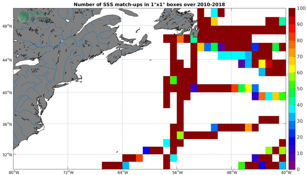
Figure 4: Number of SSS match-ups between TSG (GOSUD-Research-vessel) SSS and the CCI L4 Merged-OI v2.31 - 30-day running (ESA) SSS product for the Gulf Stream Pi-MEP region over 1^\circ \times 1^\circ boxes and for the full satellite product period.
