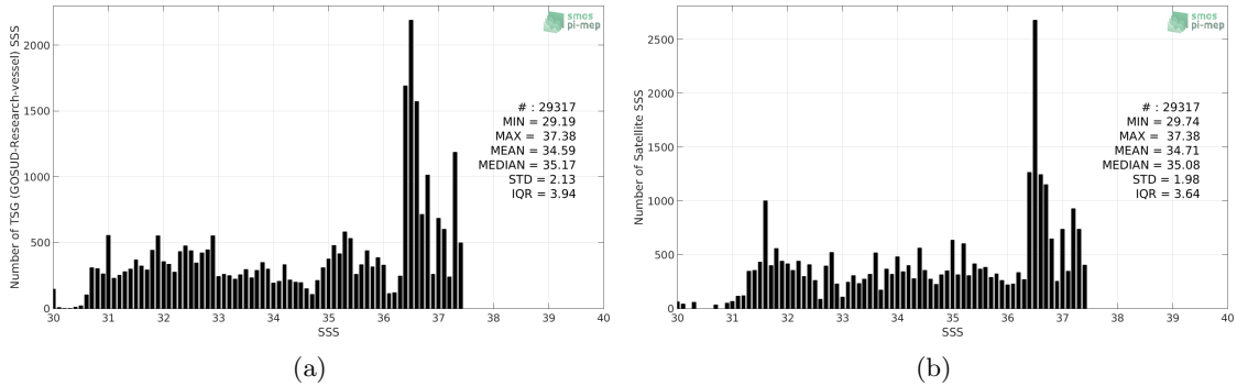
Figure 2: Histograms of SSS from TSG (GOSUD-Research-vessel) (a) and CCI L4 Merged-OI v2.31 - 30-day running (ESA) (b) considering all match-up pairs per bins of 0.1 over the Gulf Stream Pi-MEP region and for the full satellite product period.
