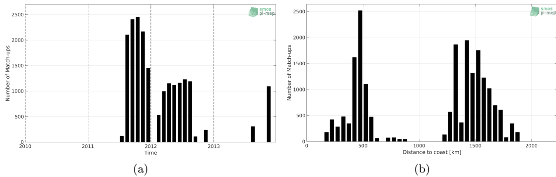
Figure 1: Number of match-ups between Surface drifters and CCI SSS L4 Merged-OI v2.31 - 30-day running (ESA) SSS as a function of time (a) and as function of the distance to coast (b) over the Gulf Stream Pi-MEP region and for the full satellite product period.
