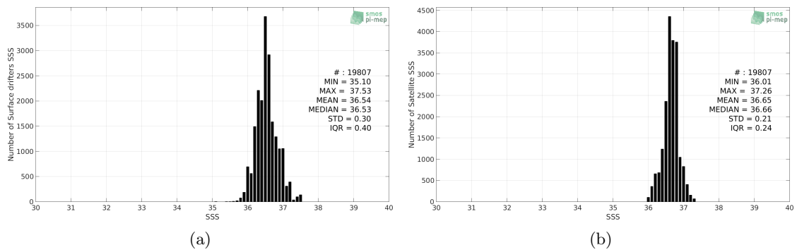
Figure 2: Histograms of SSS from Surface drifters (a) and CCI SSS L4 Merged-OI v2.31 - 30-day running (ESA) (b) considering all match-up pairs per bins of 0.1 over the Gulf Stream Pi-MEP region and for the full satellite product period.
