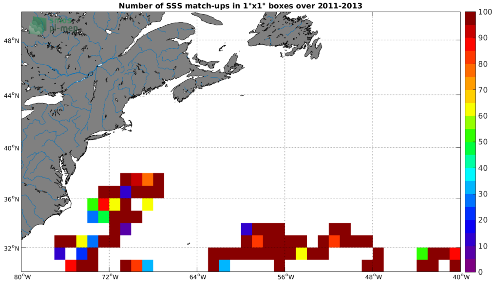
Figure 3: Number of SSS match-ups between Surface drifters SSS and the CCI SSS L4 Merged-OI v2.31 - 30-day running (ESA) SSS product for the Gulf Stream Pi-MEP region over 1°x1° boxes and for the full satellite product period.
