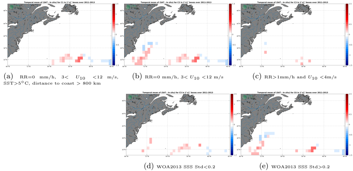
Figure 11: Temporal mean gridded over spatial boxes of size 1^{\circ}\times 1^{\circ} of \Delta\text{SSS} (CCI SSS L4 Merged-OI v2.31 - 30-day running (ESA) - Surface drifters) for 5 different subdatasets corresponding to:RR=0 mm/h, 3 < U_{10} < 12 m/s, SST >5^{\circ}\text{C} , distance to coast > 800 km (a), RR=0 mm/h, 3 < U_{10} < 12 m/s (b), RR >1 mm/h and U_{10} < 4 m/s (c), WOA2013 SSS Std <0.2 (d), WOA2013 SSS Std >0.2 (e).
