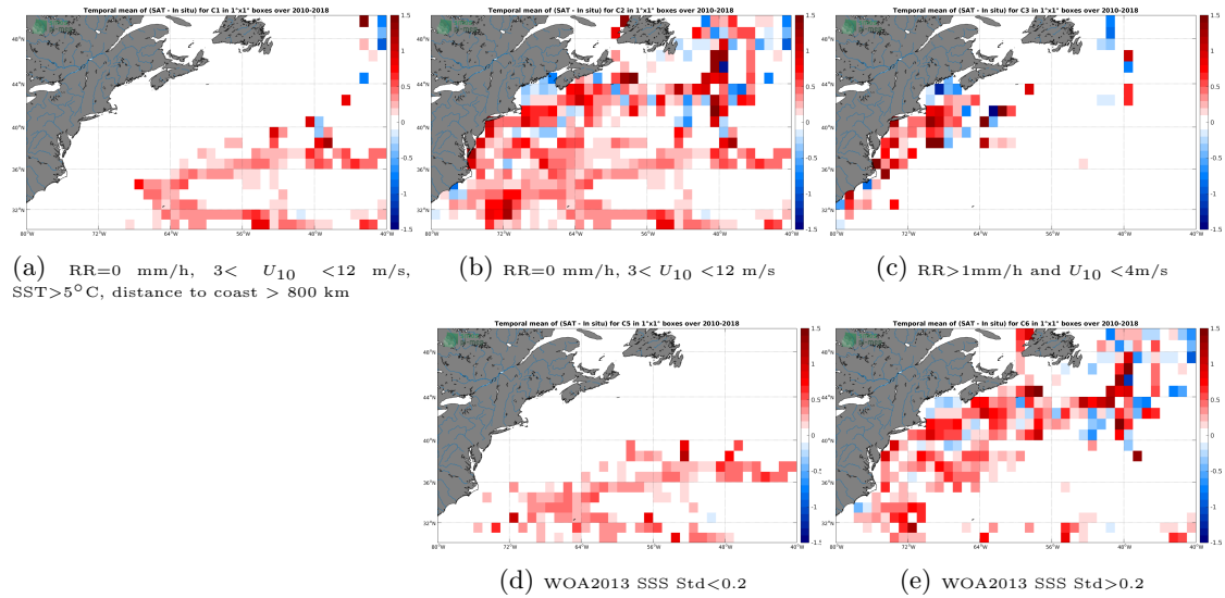
Figure 12: Temporal mean gridded over spatial boxes of size 1^\circ \times 1^\circ of \Delta SSS (CCI-L4-ESAMERGED-OI-V1.8-30DAY-RUNNING - TSG-SAMOS) for 5 different subdatasets corresponding to:RR=0 mm/h, 3 < U_{10} < 12 m/s, SST >5^\circ C, distance to coast > 800 km (a), RR=0 mm/h, 3 < U_{10} < 12 m/s (b), RR >1 mm/h and U_{10} < 4 m/s (c), WOA2013 SSS Std <0.2 (d), WOA2013 SSS Std >0.2 (e).
