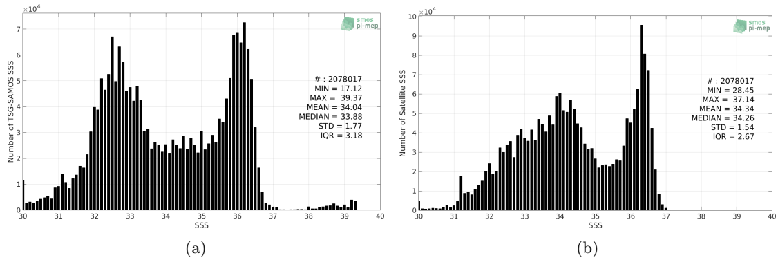
Figure 2: Histograms of SSS from TSG-SAMOS (a) and CCI-L4-ESA-MERGED-OI-V1.8-30DAY-RUNNING (b) considering all match-up pairs per bins of 0.1 over the Gulf Stream Pi-MEP region and for the full satellite product period.
