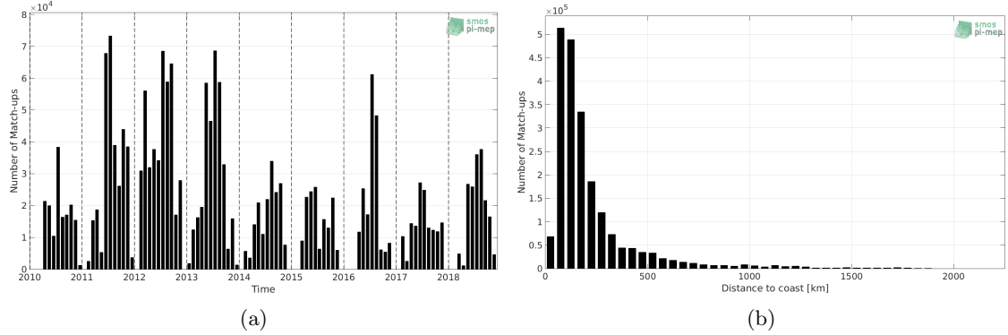
Figure 1: Number of match-ups between TSG-SAMOS and CCI-L4-ESA-MERGED-OI-V1.8-30DAY-RUNNING SSS as a function of time (a) and as function of the distance to coast (b) over the Gulf Stream Pi-MEP region and for the full satellite product period.
