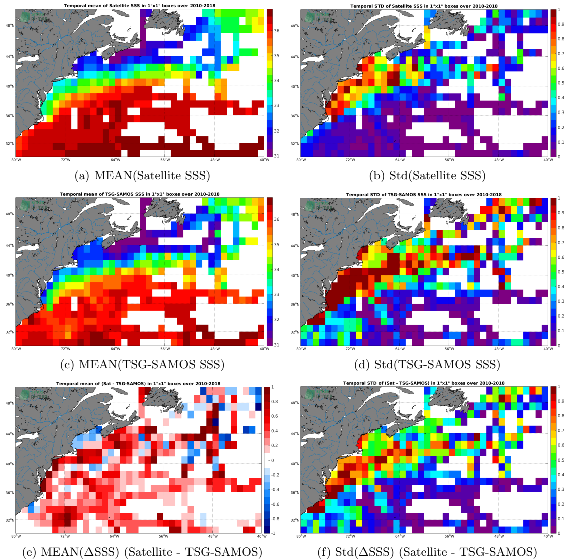
Figure 6: Temporal mean (left) and Std (right) of SSS from CCI-L4-ESA-MERGED-OI-V1.8-30DAY-RUNNING (top), TSG-SAMOS (middle), and of \Delta SSS (Satellite - TSG-SAMOS). Only match-up pairs are used to generate these maps.
