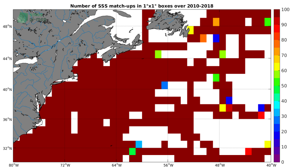
Figure 4: Number of SSS match-ups between TSG-SAMOS SSS and the CCI-L4-ESA-MERGED-OI-V1.8-30DAY-RUNNING SSS product for the Gulf Stream Pi-MEP region over 1^\circ \times 1^\circ boxes and for the full satellite product period.
