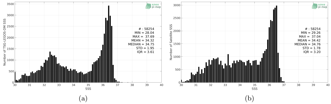
Figure 2: Histograms of SSS from TSG-LEGOS-DM (a) and CCI-L4-ESA-MERGED-OI-V1.8-30DAY-RUNNING (b) considering all match-up pairs per bins of 0.1 over the Gulf Stream Pi-MEP region and for the full satellite product period.
