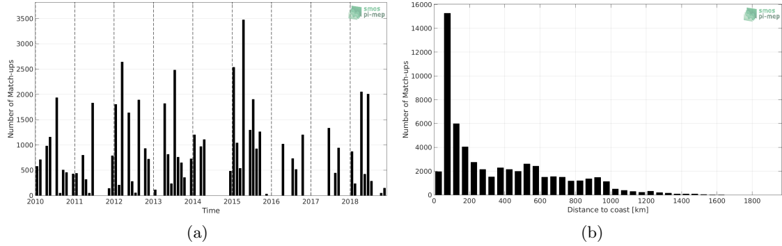
Figure 1: Number of match-ups between TSG-LEGOS-DM and CCI-L4-ESA-MERGED-OI-V1.8-30DAY-RUNNING SSS as a function of time (a) and as function of the distance to coast (b) over the Gulf Stream Pi-MEP region and for the full satellite product period.
