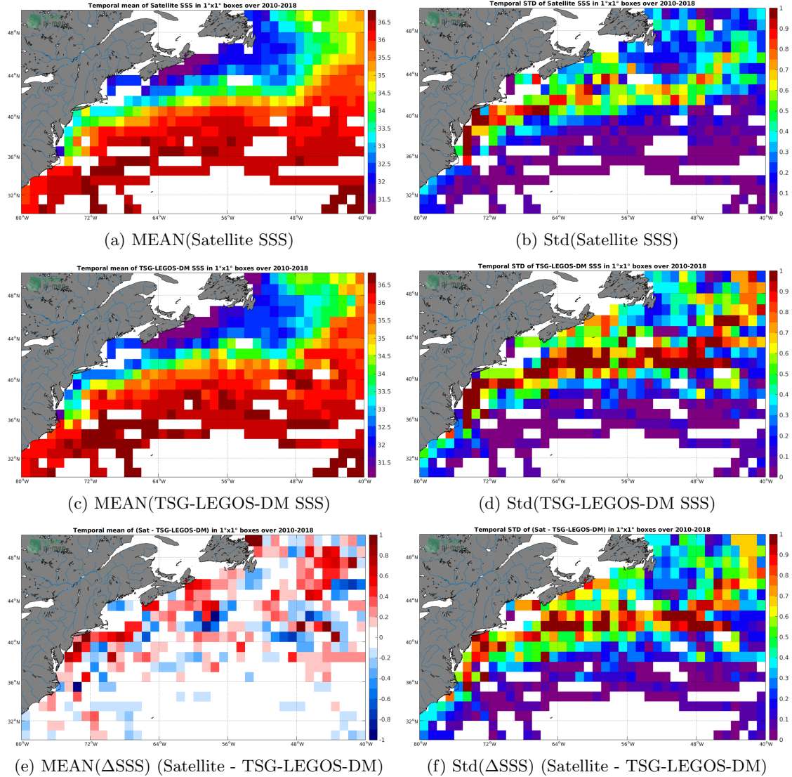
Figure 6: Temporal mean (left) and Std (right) of SSS from CCI-L4-ESA-MERGED-OI-V1.8-30DAY-RUNNING (top), TSG-LEGOS-DM (middle), and of \Delta SSS (Satellite - TSG-LEGOS-DM). Only match-up pairs are used to generate these maps.
