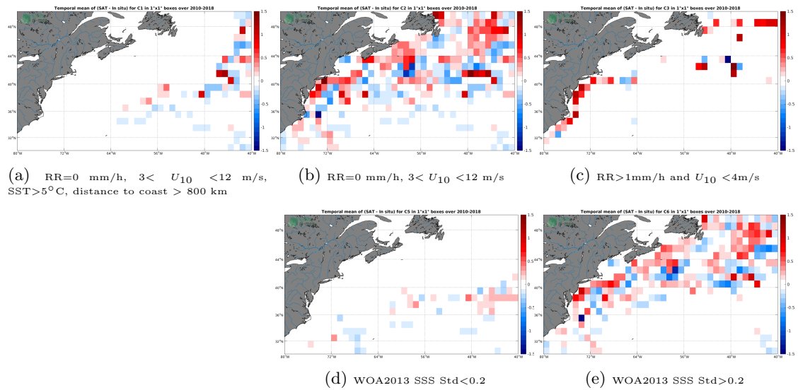
Figure 12: Temporal mean gridded over spatial boxes of size 1^\circ \times 1^\circ of \Delta SSS (CCI-L4-ESAMERGED-OI-V1.8-30DAY-RUNNING - TSG-LEGOS-DM) for 5 different subdatasets corresponding to:RR=0 mm/h, 3 < U_{10} < 12 m/s, SST >5^\circ C, distance to coast > 800 km (a), RR=0 mm/h, 3 < U_{10} < 12 m/s (b), RR >1 mm/h and U_{10} < 4 m/s (c), WOA2013 SSS Std <0.2 (d), WOA2013 SSS Std >0.2 (e).
