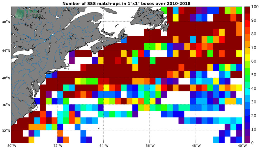
Figure 4: Number of SSS match-ups between TSG-LEGOS-DM SSS and the CCI-L4-ESA-MERGED-OI-V1.8-30DAY-RUNNING SSS product for the Gulf Stream Pi-MEP region over 1^\circ \times 1^\circ boxes and for the full satellite product period.
