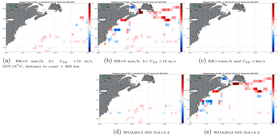
Figure 12: Temporal mean gridded over spatial boxes of size 1^{\circ}\times 1^{\circ} of \Delta SSS (CCI L4 Merged-OI v1.8 - 30-day running (ESA) - TSG-GOSUD-Sailing-ship) for 5 different subdatasets corresponding to: RR=0 mm/h, 3 < U_{10} < 12 m/s, SST > 5^{\circ}\text{C} , distance to coast > 800 km (a), RR=0 mm/h, 3 < U_{10} < 12 m/s (b), RR > 1 mm/h and U_{10} < 4 m/s (c), WOA2013 SSS Std < 0.2 (d), WOA2013 SSS Std > 0.2 (e).
