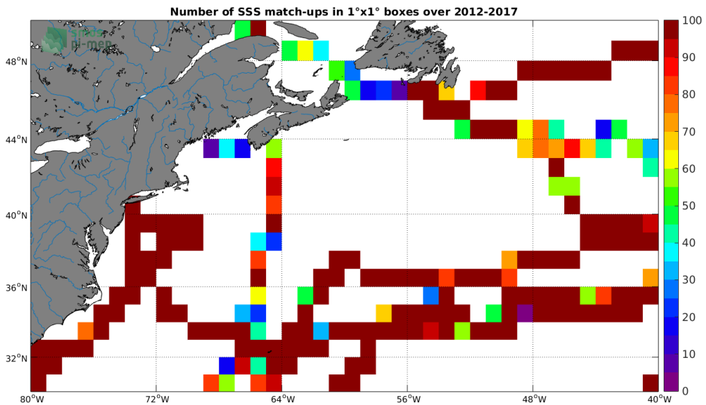
Figure 4: Number of SSS match-ups between TSG-GOSUD-Sailing-ship SSS and the CCI L4 Merged-OI v1.8 - 30-day running (ESA) SSS product for the Gulf Stream Pi-MEP region over 1^\circ \times 1^\circ boxes and for the full satellite product period.
