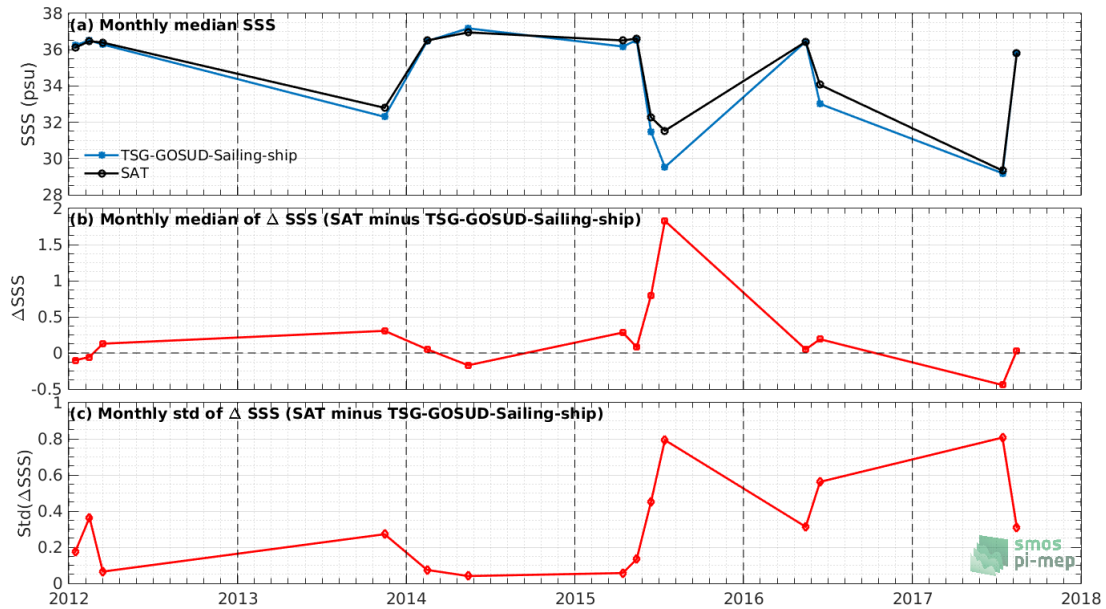
Figure 7: Time series of the monthly median SSS (top), median of \Delta\text{SSS} (Satellite - TSG-GOSUD-Sailing-ship) and Std of \Delta\text{SSS} (Satellite - TSG-GOSUD-Sailing-ship) over the Gulf Stream Pi-MEP region considering all match-ups collected by the Pi-MEP.
