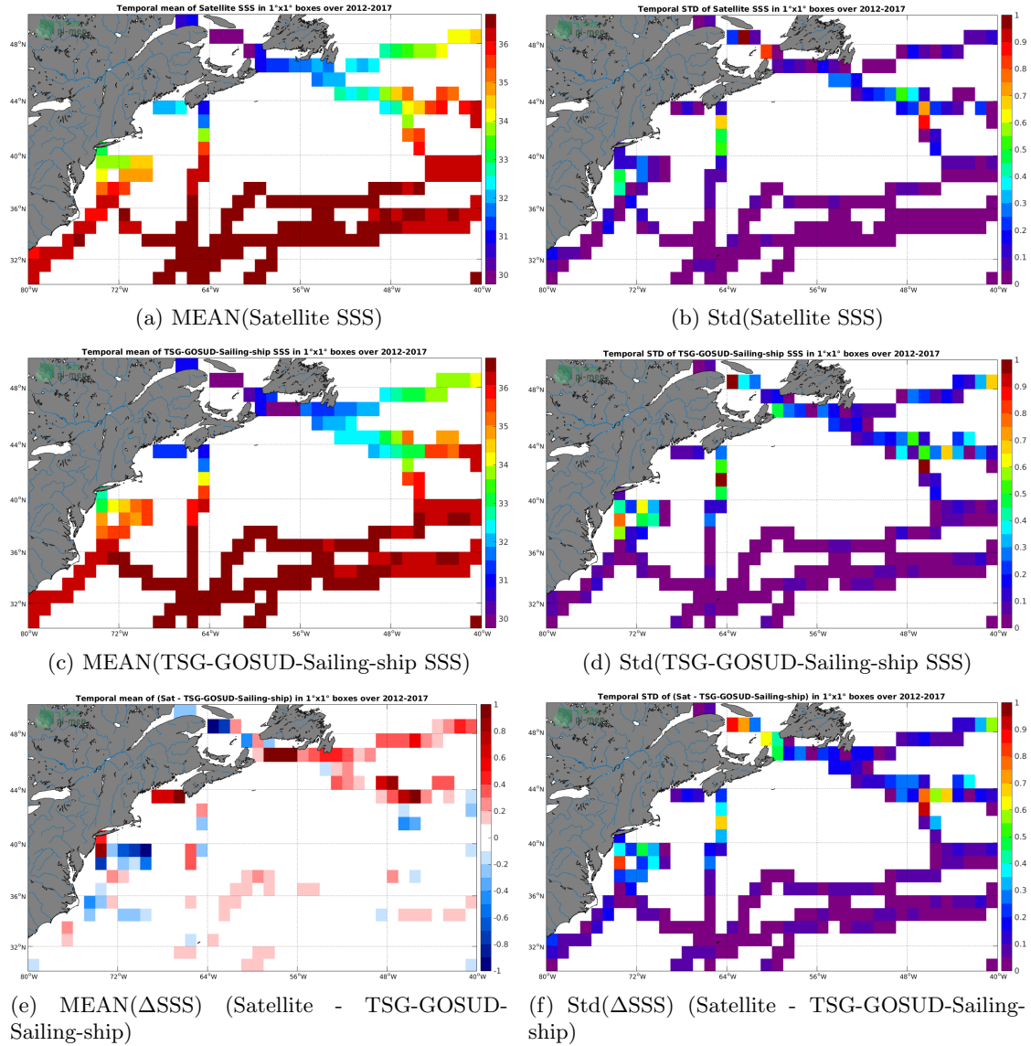
Figure 6: Temporal mean (left) and Std (right) of SSS from CCI L4 Merged-OI v1.8 - 30-day running (ESA) (top), TSG-GOSUD-Sailing-ship (middle), and of \Delta SSS (Satellite - TSG-GOSUD-Sailing-ship). Only match-up pairs are used to generate these maps.
