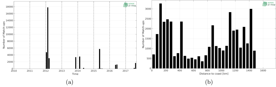
Figure 1: Number of match-ups between TSG-GOSUD-Sailing-ship and CCI L4 Merged-OI v1.8 - 30-day running (ESA) SSS as a function of time (a) and as function of the distance to coast (b) over the Gulf Stream Pi-MEP region and for the full satellite product period.
