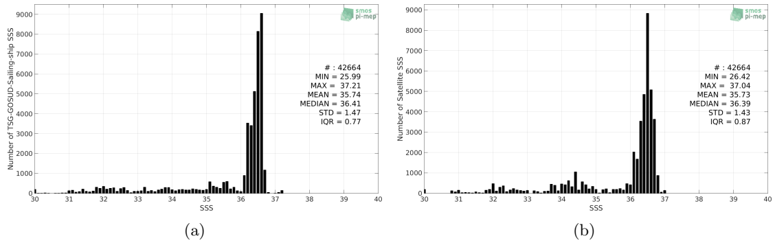
Figure 2: Histograms of SSS from TSG-GOSUD-Sailing-ship (a) and CCI L4 Merged-OI v1.8 - 30-day running (ESA) (b) considering all match-up pairs per bins of 0.1 over the Gulf Stream Pi-MEP region and for the full satellite product period.
