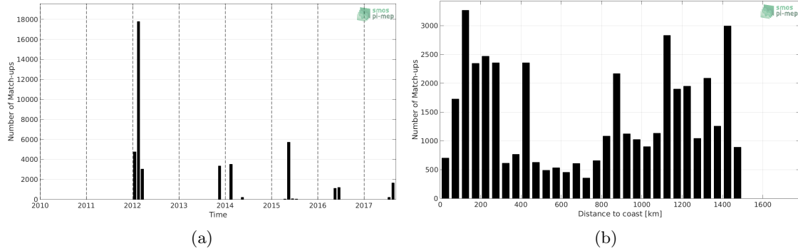
Figure 1: Number of match-ups between TSG-GOSUD-Sailing-ship and CCI-L4-ESA-MERGED-OI-V1.8-30DAY-RUNNING SSS as a function of time (a) and as function of the distance to coast (b) over the Gulf Stream Pi-MEP region and for the full satellite product period.
