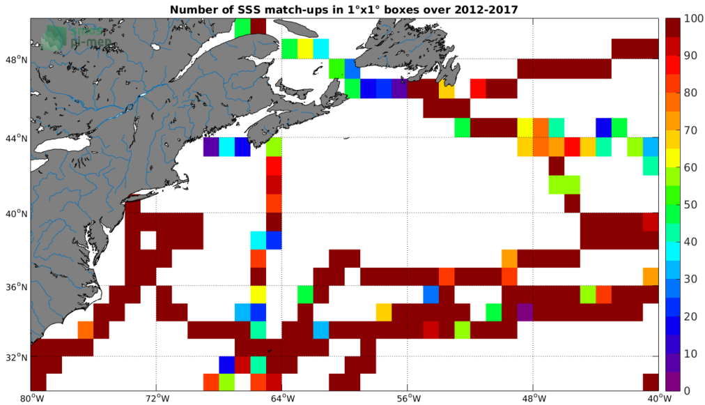
Figure 4: Number of SSS match-ups between TSG-GOSUD-Sailing-ship SSS and the CCI-L4-ESA-MERGED-OI-V1.8-30DAY-RUNNING SSS product for the Gulf Stream Pi-MEP region over 1^\circ \times 1^\circ boxes and for the full satellite product period.
