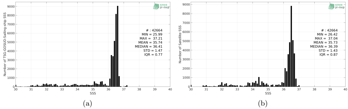
Figure 2: Histograms of SSS from TSG-GOSUD-Sailing-ship (a) and CCI-L4-ESA-MERGED-OI-V1.8-30DAY-RUNNING (b) considering all match-up pairs per bins of 0.1 over the Gulf Stream Pi-MEP region and for the full satellite product period.
