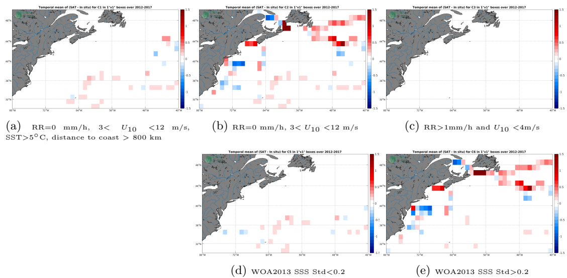
Figure 12: Temporal mean gridded over spatial boxes of size 1^\circ \times 1^\circ of \Delta SSS (CCI-L4-ESAMERGED-OI-V1.8-30DAY-RUNNING - TSG-GOSUD-Sailing-ship) for 5 different subdatasets corresponding to: RR=0 mm/h, 3 < U_{10} < 12 m/s, SST>5°C, distance to coast > 800 km (a), RR=0 mm/h, 3 < U_{10} < 12 m/s (b), RR>1mm/h and U_{10} < 4 m/s (c), WOA2013 SSS Std<0.2 (d), WOA2013 SSS Std>0.2 (e).
