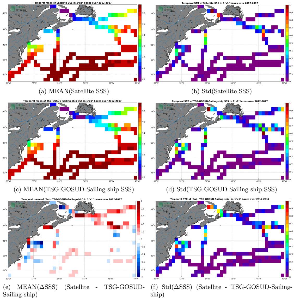
Figure 6: Temporal mean (left) and Std (right) of SSS from CCI-L4-ESA-MERGED-OI-V1.8-30DAY-RUNNING (top), TSG-GOSUD-Sailing-ship (middle), and of \Delta SSS (Satellite - TSG-GOSUD-Sailing-ship). Only match-up pairs are used to generate these maps.
