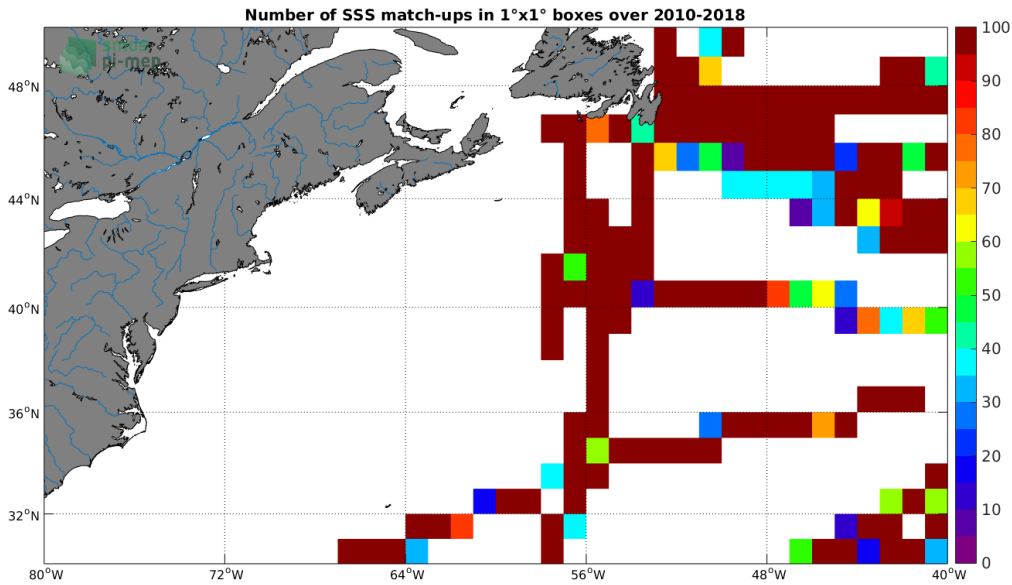
Figure 4: Number of SSS match-ups between TSG-GOSUD-Research-vessel SSS and the CCI L4 Merged-OI v1.8 - 30-day running (ESA) SSS product for the Gulf Stream Pi-MEP region over 1°x1° boxes and for the full satellite product period.
