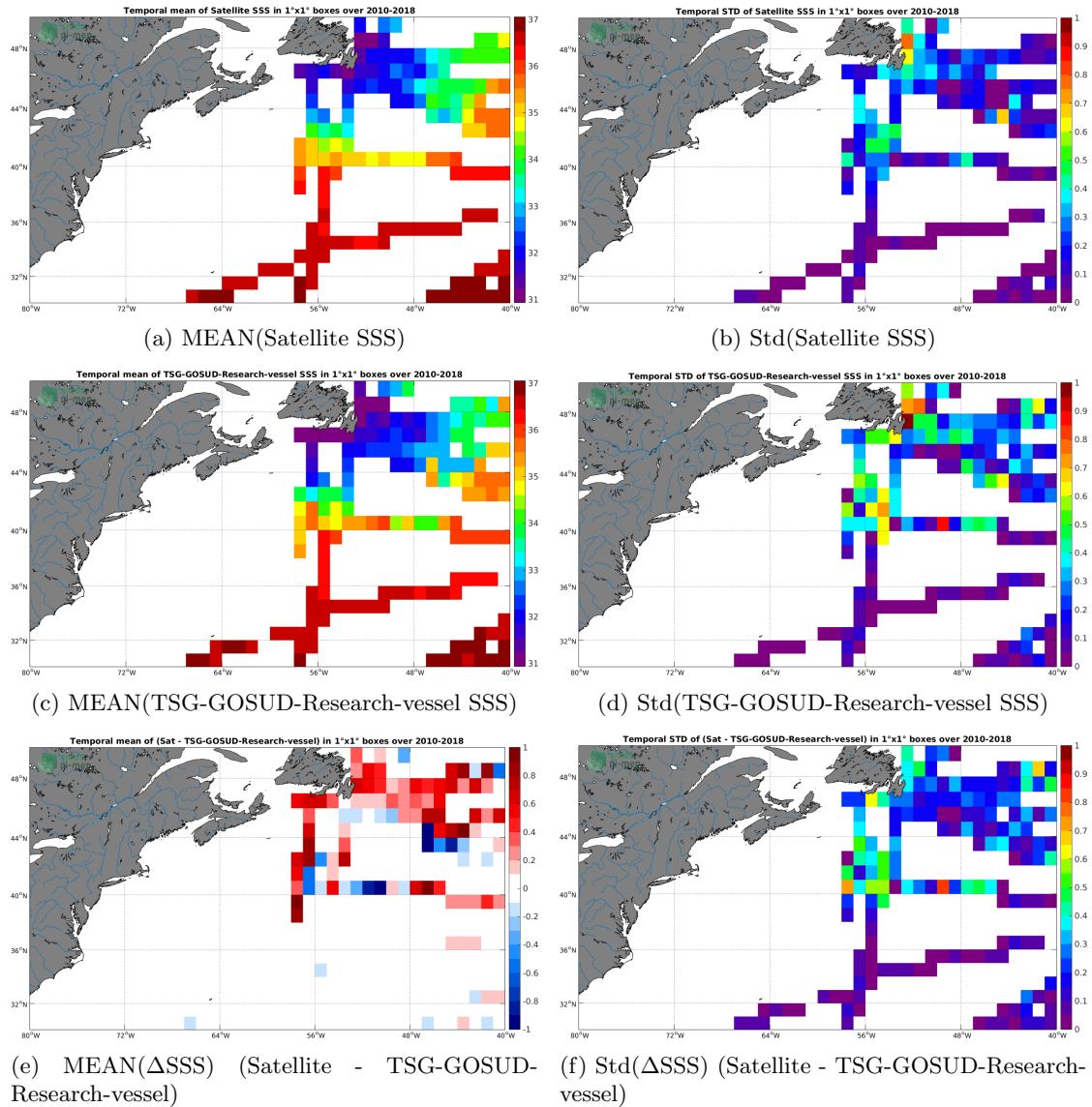
Figure 6: Temporal mean (left) and Std (right) of SSS from CCI L4 Merged-OI v1.8 - 30-day running (ESA) (top), TSG-GOSUD-Research-vessel (middle), and of \Delta SSS (Satellite - TSG-GOSUD-Research-vessel). Only match-up pairs are used to generate these maps.
