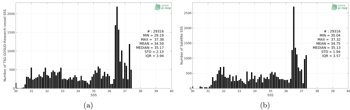
Figure 2: Histograms of SSS from TSG-GOSUD-Research-vessel (a) and CCI L4 Merged-OI v1.8 - 30-day running (ESA) (b) considering all match-up pairs per bins of 0.1 over the Gulf Stream Pi-MEP region and for the full satellite product period.
