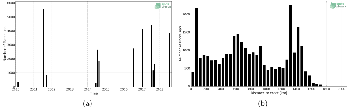
Figure 1: Number of match-ups between TSG-GOSUD-Research-vessel and CCI L4 Merged-OI v1.8 - 30-day running (ESA) SSS as a function of time (a) and as function of the distance to coast (b) over the Gulf Stream Pi-MEP region and for the full satellite product period.
