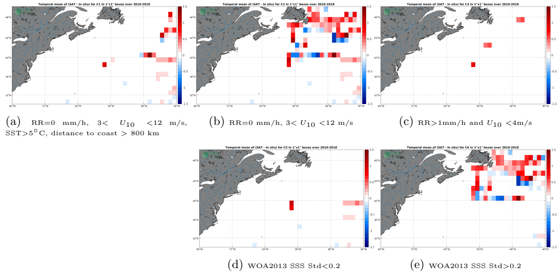
Figure 12: Temporal mean gridded over spatial boxes of size 1^\circ \times 1^\circ of \Delta SSS (CCI L4 Merged-OI v1.8 - 30-day running (ESA) - TSG-GOSUD-Research-vessel) for 5 different subdatasets corresponding to: RR=0 mm/h, 3 < U_{10} < 12 m/s, SST > 5^\circ\text{C} , distance to coast > 800 km (a), RR=0 mm/h, 3 < U_{10} < 12 m/s (b), RR > 1 mm/h and U_{10} < 4 m/s (c), WOA2013 SSS Std < 0.2 (d), WOA2013 SSS Std > 0.2 (e).
