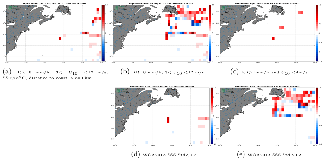
Figure 12: Temporal mean gridded over spatial boxes of size 1^\circ \times 1^\circ of \Delta SSS (CCI-L4-ESA-MERGED-OI-V1.8-30DAY-RUNNING - TSG-GOSUD-Research-vessel) for 5 different sub-datasets corresponding to:RR=0 mm/h, 3 < U_{10} < 12 m/s, SST>5°C, distance to coast > 800 km (a), RR=0 mm/h, 3 < U_{10} < 12 m/s (b), RR>1mm/h and U_{10} < 4 m/s (c), WOA2013 SSS Std<0.2 (d), WOA2013 SSS Std>0.2 (e).
