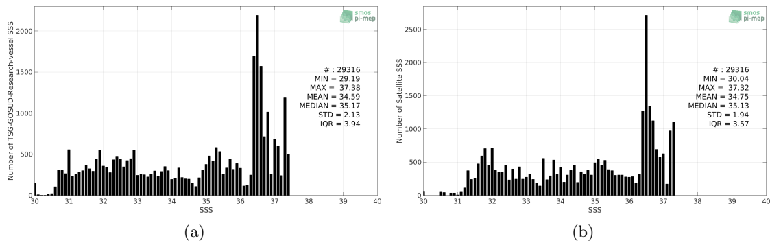
Figure 2: Histograms of SSS from TSG-GOSUD-Research-vessel (a) and CCI-L4-ESA-MERGED-OI-V1.8-30DAY-RUNNING (b) considering all match-up pairs per bins of 0.1 over the Gulf Stream Pi-MEP region and for the full satellite product period.
