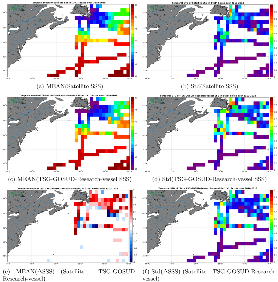
Figure 6: Temporal mean (left) and Std (right) of SSS from CCI-L4-ESA-MERGED-OI-V1.8-30DAY-RUNNING (top), TSG-GOSUD-Research-vessel (middle), and of \Delta SSS (Satellite - TSG-GOSUD-Research-vessel). Only match-up pairs are used to generate these maps.
