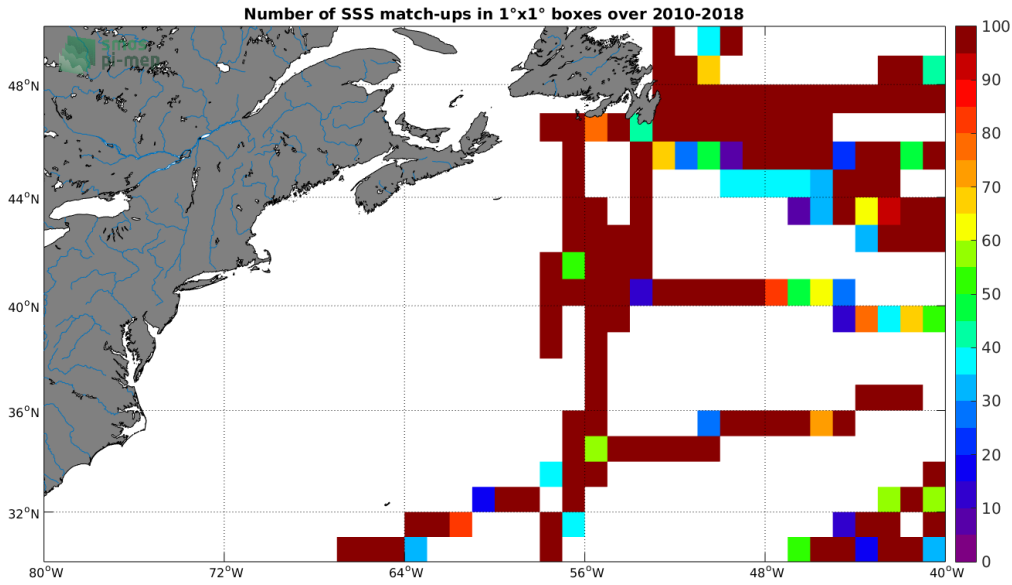
Figure 4: Number of SSS match-ups between TSG-GOSUD-Research-vessel SSS and the CCI-L4-ESA-MERGED-OI-V1.8-30DAY-RUNNING SSS product for the Gulf Stream Pi-MEP region over 1°x1° boxes and for the full satellite product period.
