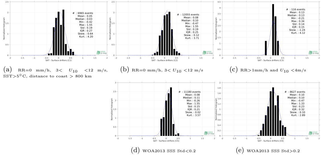
Figure 12: Normalized histogram of \Delta SSS (CCI-L4-ESA-MERGED-OI-V1.8-30DAY-RUNNING - Surface drifters) for 5 different subdatasets corresponding to: RR=0 mm/h, 3 < U_{10} < 12 m/s, SST>5°C, distance to coast > 800 km (a), RR=0 mm/h, 3 < U_{10} < 12 m/s (b), RR>1mm/h and U_{10} < 4 m/s (c), WOA2013 SSS Std<0.2 (d), WOA2013 SSS Std>0.2 (e).
