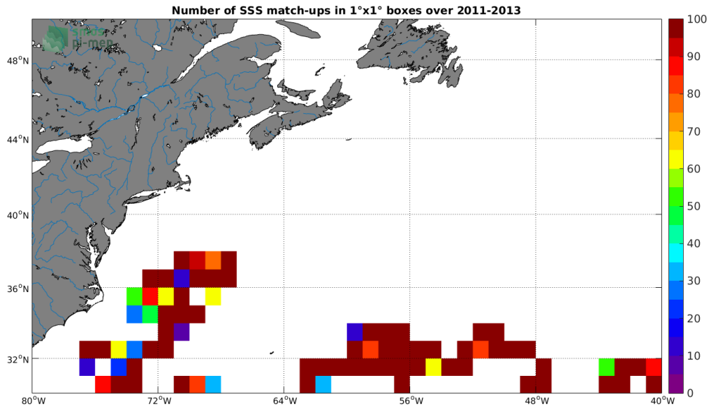
Figure 3: Number of SSS match-ups between Surface drifters SSS and the CCI-L4-ESA-MERGED-OI-V1.8-30DAY-RUNNING SSS product for the Gulf Stream Pi-MEP region over 1°x1° boxes and for the full satellite product period.
