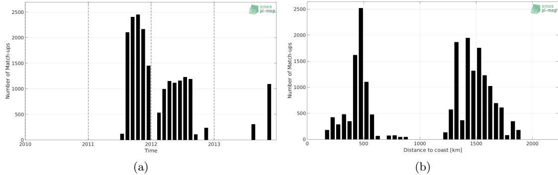
Figure 1: Number of match-ups between Surface drifters and CCI-L4-ESA-MERGED-OI-V1.8-30DAY-RUNNING SSS as a function of time (a) and as function of the distance to coast (b) over the Gulf Stream Pi-MEP region and for the full satellite product period.
