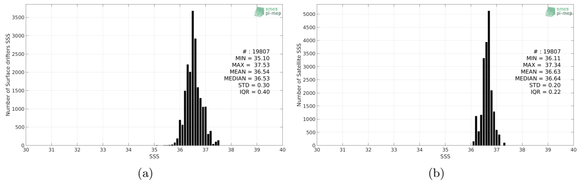
Figure 2: Histograms of SSS from Surface drifters (a) and CCI-L4-ESA-MERGED-OI-V1.8-30DAY-RUNNING (b) considering all match-up pairs per bins of 0.1 over the Gulf Stream Pi-MEP region and for the full satellite product period.
