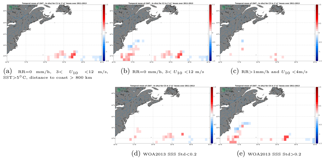
Figure 11: Temporal mean gridded over spatial boxes of size 1^\circ \times 1^\circ of \Delta SSS (CCI-L4-ESAMERGED-OI-V1.8-30DAY-RUNNING - Surface drifters) for 5 different subdatasets corresponding to:RR=0 mm/h, 3 < U_{10} < 12 m/s, SST >5^\circ C, distance to coast > 800 km (a), RR=0 mm/h, 3 < U_{10} < 12 m/s (b), RR >1 mm/h and U_{10} < 4 m/s (c), WOA2013 SSS Std <0.2 (d), WOA2013 SSS Std >0.2 (e).
