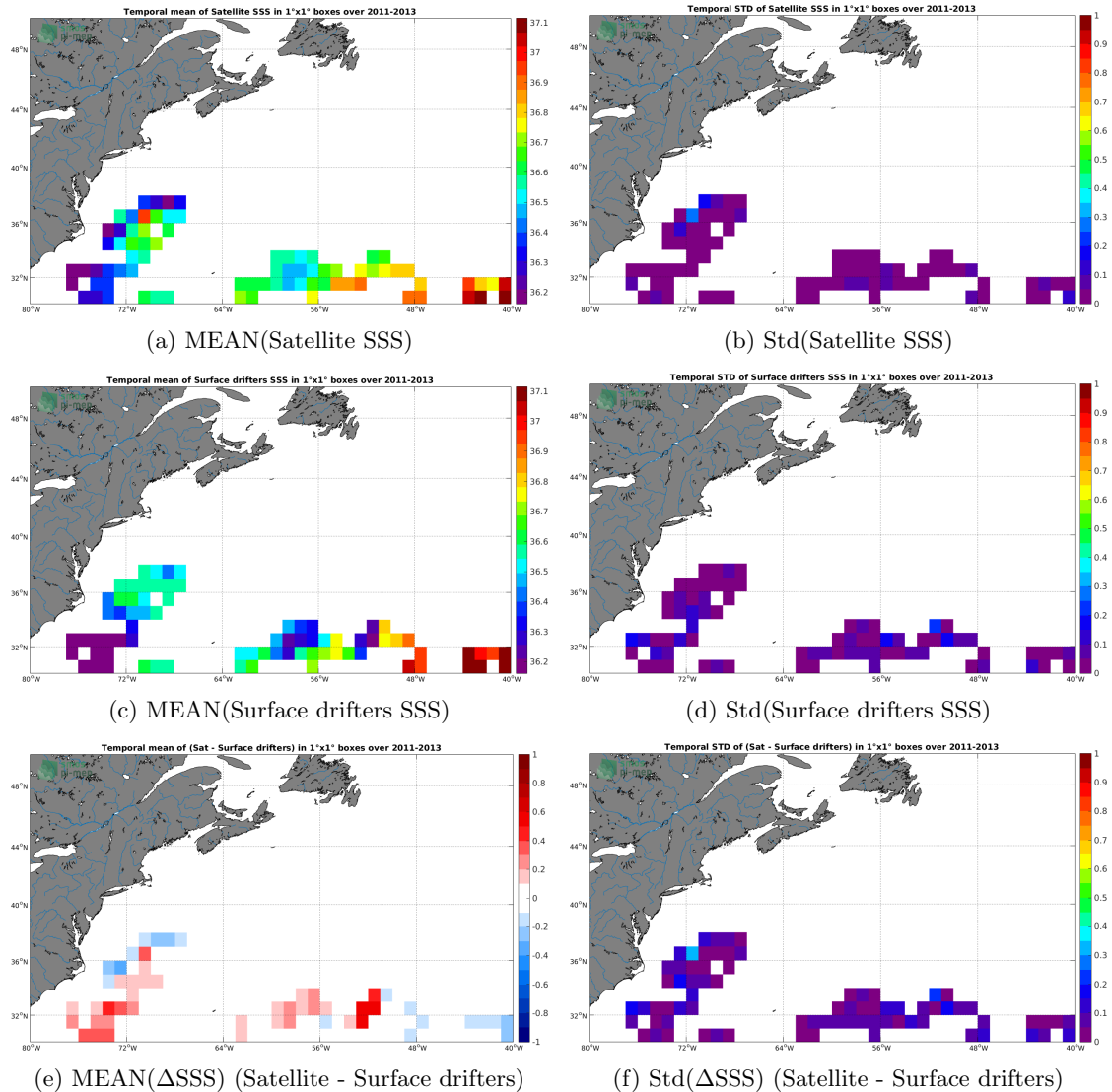
Figure 5: Temporal mean (left) and Std (right) of SSS from CCI-L4-ESA-MERGED-OI-V1.8-30DAY-RUNNING (top), Surface drifters (middle), and of \Delta SSS (Satellite - Surface drifters). Only match-up pairs are used to generate these maps.
