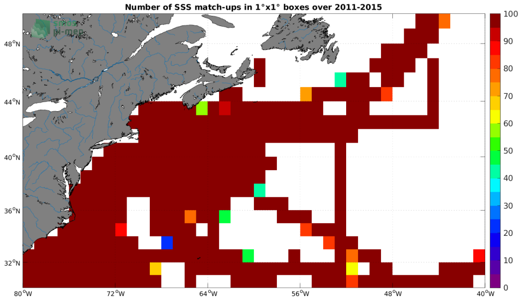
Figure 4: Number of SSS match-ups between TSG (SAMOS) SSS and the Aquarius SSS L4 OI v5 - Weekly (IPRC) SSS product for the Gulf Stream Pi-MEP region over 1^{\circ} \times 1^{\circ} boxes and for the full satellite product period.
