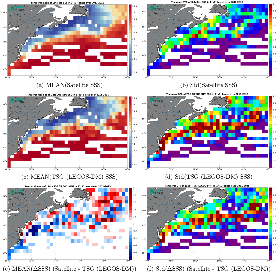
Figure 7: Temporal mean (left) and Std (right) of SSS from Aquarius SSS L4 OI v5 - Weekly (IPRC) (top), TSG (LEGOS-DM) (middle), and of \Delta SSS (Satellite - TSG (LEGOS-DM)). Only match-up pairs are used to generate these maps.
