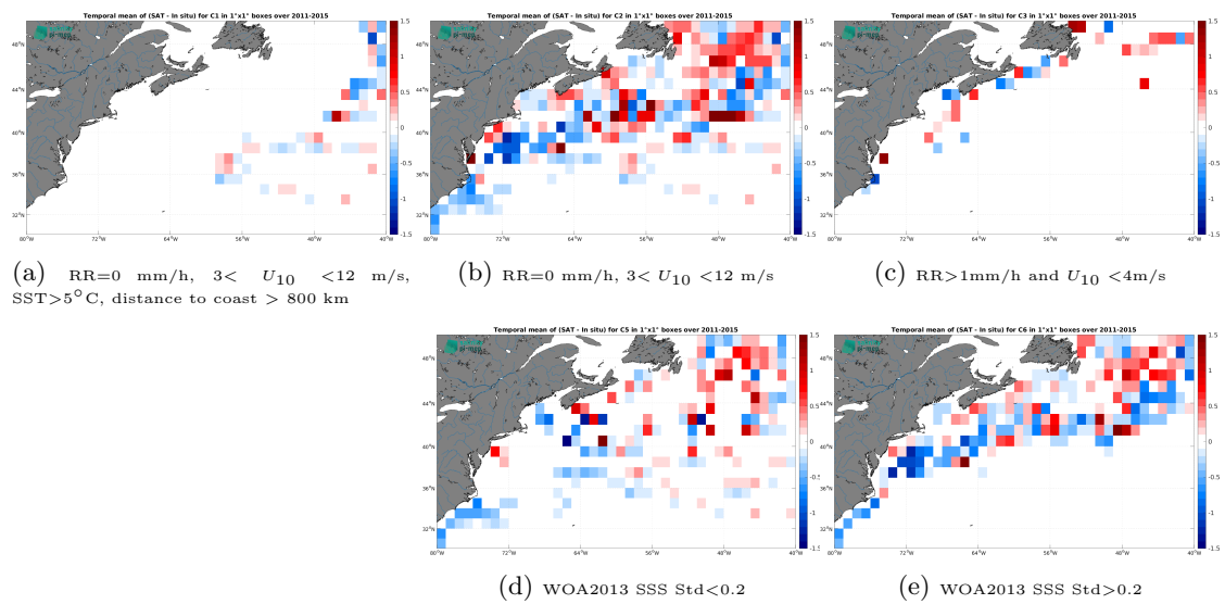
Figure 14: Temporal mean gridded over spatial boxes of size 1^\circ \times 1^\circ of \Delta SSS (Aquarius SSS L4 OI v5 - Weekly (IPRC) - TSG (LEGOS-DM)) for 5 different subdatasets corresponding to:RR=0 mm/h, 3 < U_{10} < 12 m/s, SST > 5°C, distance to coast > 800 km (a), RR=0 mm/h, 3 < U_{10} < 12 m/s (b), RR > 1mm/h and U_{10} < 4 m/s (c), WOA2013 SSS Std < 0.2 (d), WOA2013 SSS Std > 0.2 (e).
