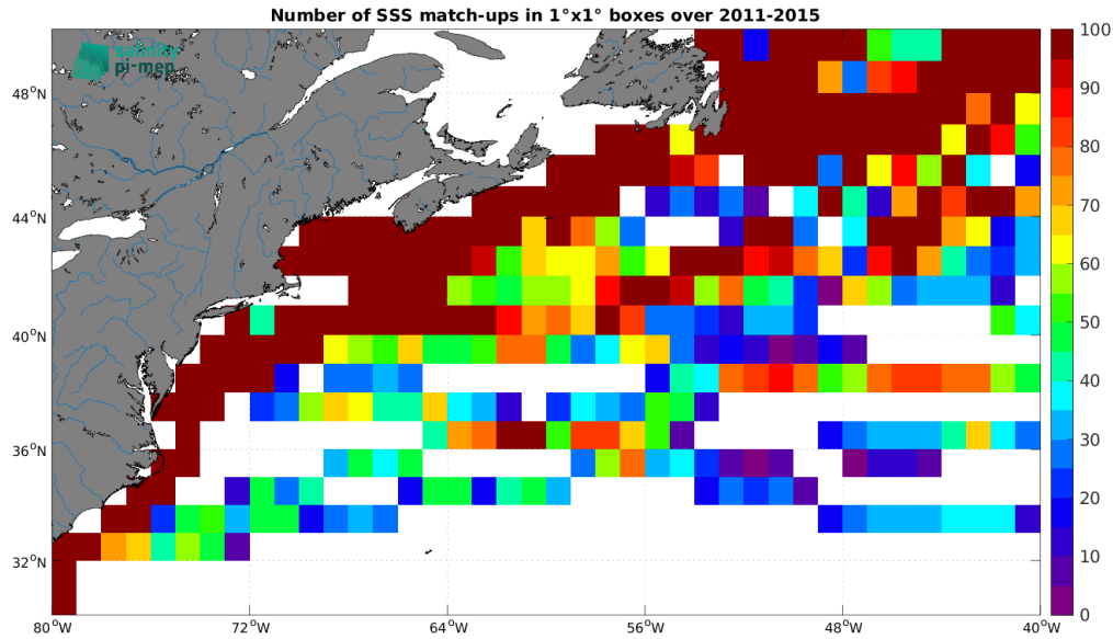
Figure 5: Number of SSS match-ups between TSG (LEGOS-DM) SSS and the Aquarius SSS L4 OI v5 - Weekly (IPRC) SSS product for the Gulf Stream Pi-MEP region over 1^\circ \times 1^\circ boxes and for the full satellite product period.
