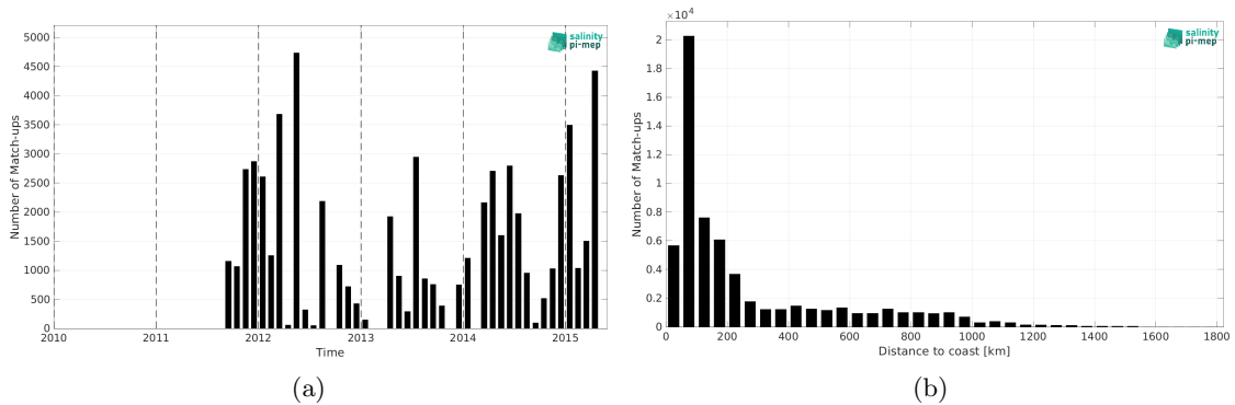
Figure 2: Number of match-ups between TSG (LEGOS-DM) and Aquarius SSS L4 OI v5 - Weekly (IPRC) SSS as a function of time (a) and as function of the distance to coast (b) over the Gulf Stream Pi-MEP region and for the full satellite product period.
