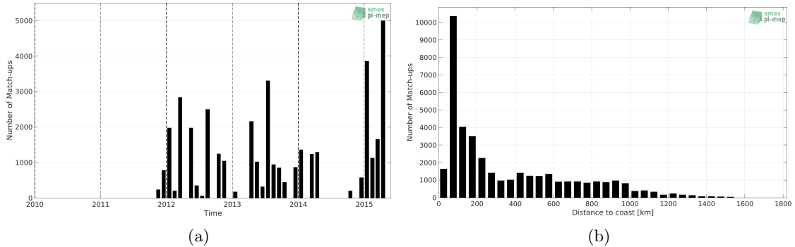
Figure 1: Number of match-ups between TSG (LEGOS-DM) and Aquarius SSS L4 OI v5 - Weekly (IPRC) SSS as a function of time (a) and as function of the distance to coast (b) over the Gulf Stream Pi-MEP region and for the full satellite product period.
