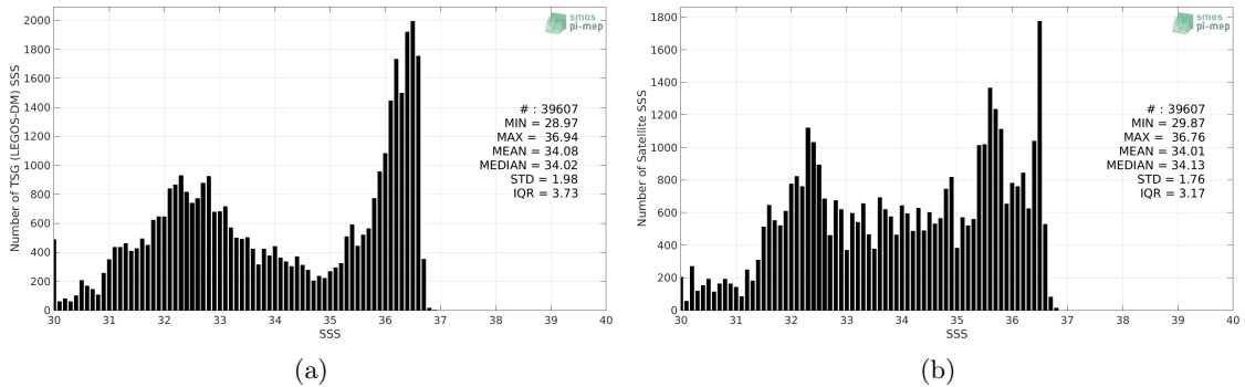
Figure 2: Histograms of SSS from TSG (LEGOS-DM) (a) and Aquarius SSS L4 OI v5 - Weekly (IPRC) (b) considering all match-up pairs per bins of 0.1 over the Gulf Stream Pi-MEP region and for the full satellite product period.
