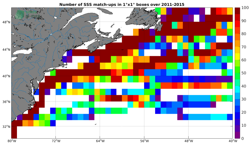
Figure 4: Number of SSS match-ups between TSG (LEGOS-DM) SSS and the Aquarius SSS L4 OI v5 - Weekly (IPRC) SSS product for the Gulf Stream Pi-MEP region over 1^\circ \times 1^\circ boxes and for the full satellite product period.
