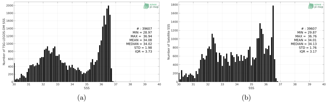
Figure 2: Histograms of SSS from TSG-LEGOS-DM (a) and Aquarius-L4-IPRC-V5-WEEKLY (b) considering all match-up pairs per bins of 0.1 over the Gulf Stream Pi-MEP region and for the full satellite product period.
