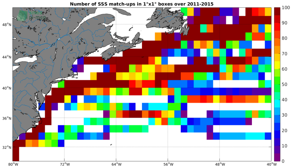
Figure 4: Number of SSS match-ups between TSG-LEGOS-DM SSS and the Aquarius-L4-IPRC-V5-WEEKLY SSS product for the Gulf Stream Pi-MEP region over 1^\circ \times 1^\circ boxes and for the full satellite product period.
