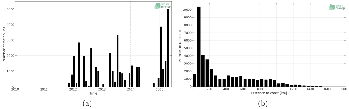
Figure 1: Number of match-ups between TSG-LEGOS-DM and Aquarius-L4-IPRC-V5-WEEKLY SSS as a function of time (a) and as function of the distance to coast (b) over the Gulf Stream Pi-MEP region and for the full satellite product period.
