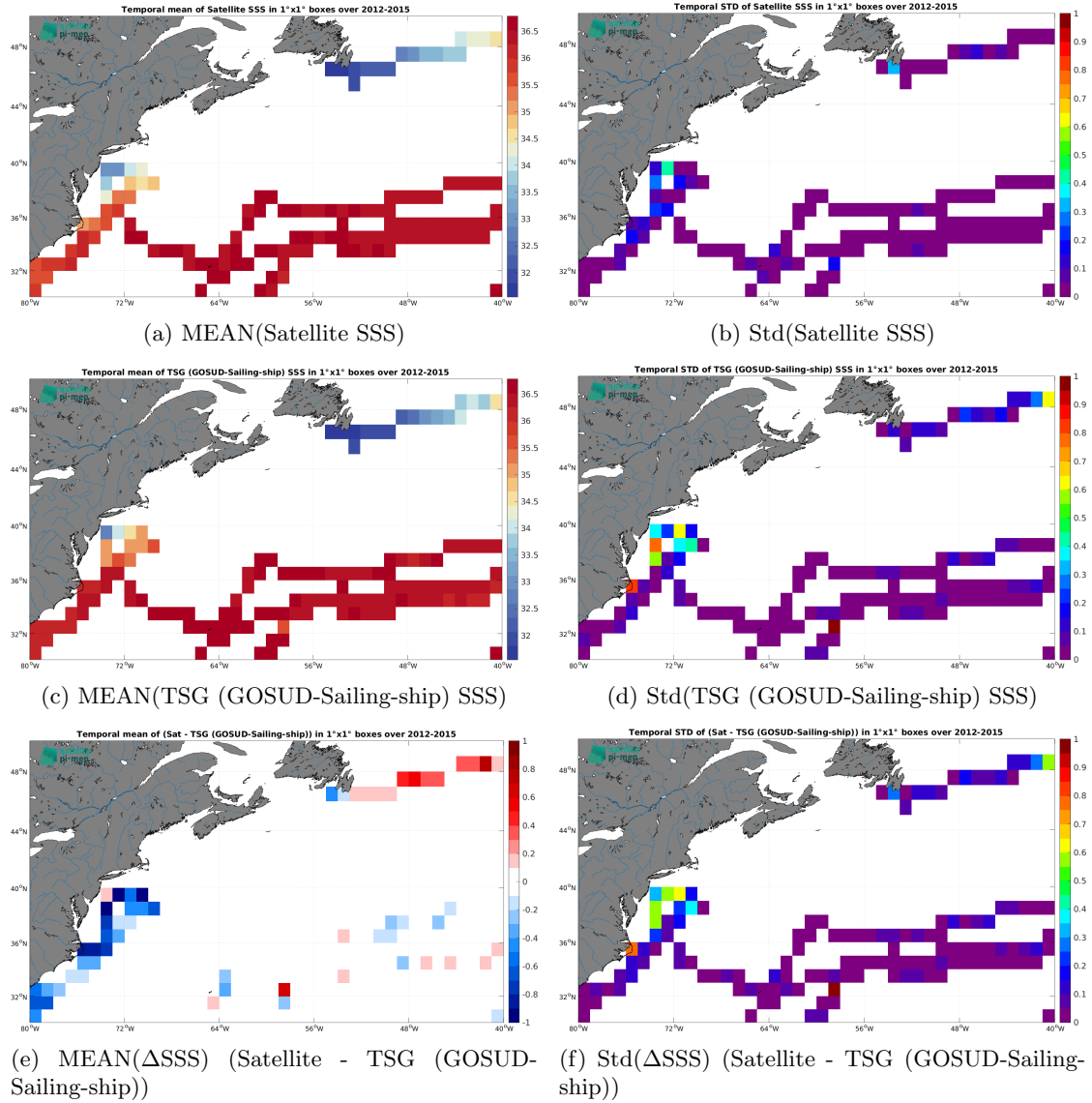
Figure 7: Temporal mean (left) and Std (right) of SSS from Aquarius SSS L4 OI v5 - Weekly (IPRC) (top), TSG (GOSUD-Sailing-ship) (middle), and of \Delta SSS (Satellite - TSG (GOSUD-Sailing-ship)). Only match-up pairs are used to generate these maps.
