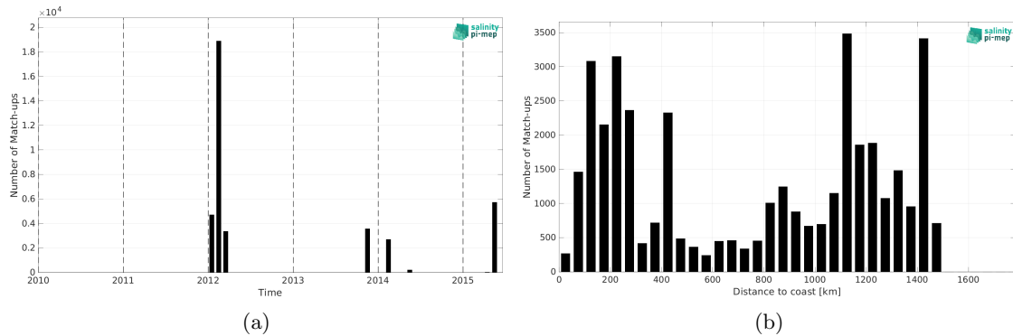
Figure 2: Number of match-ups between TSG (GOSUD-Sailing-ship) and Aquarius SSS L4 OI v5 - Weekly (IPRC) SSS as a function of time (a) and as function of the distance to coast (b) over the Gulf Stream Pi-MEP region and for the full satellite product period.
