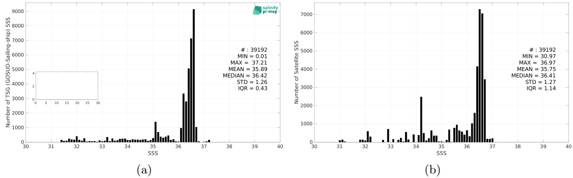
Figure 3: Histograms of SSS from TSG (GOSUD-Sailing-ship) (a) and Aquarius SSS L4 OI v5 - Weekly (IPRC) (b) considering all match-up pairs per bins of 0.1 over the Gulf Stream Pi-MEP region and for the full satellite product period.
