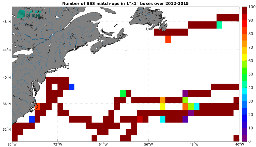
Figure 5: Number of SSS match-ups between TSG (GOSUD-Sailing-ship) SSS and the Aquarius SSS L4 OI v5 - Weekly (IPRC) SSS product for the Gulf Stream Pi-MEP region over 1^\circ \times 1^\circ boxes and for the full satellite product period.
