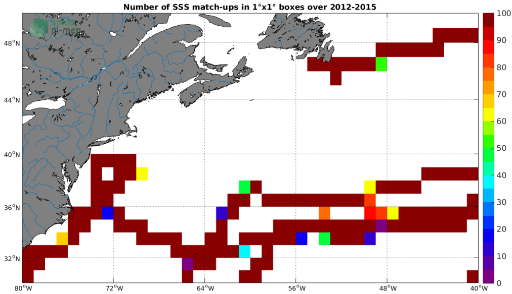
Figure 4: Number of SSS match-ups between TSG (GOSUD-Sailing-ship) SSS and the Aquarius SSS L4 OI v5 - Weekly (IPRC) SSS product for the Gulf Stream Pi-MEP region over 1^\circ \times 1^\circ boxes and for the full satellite product period.
