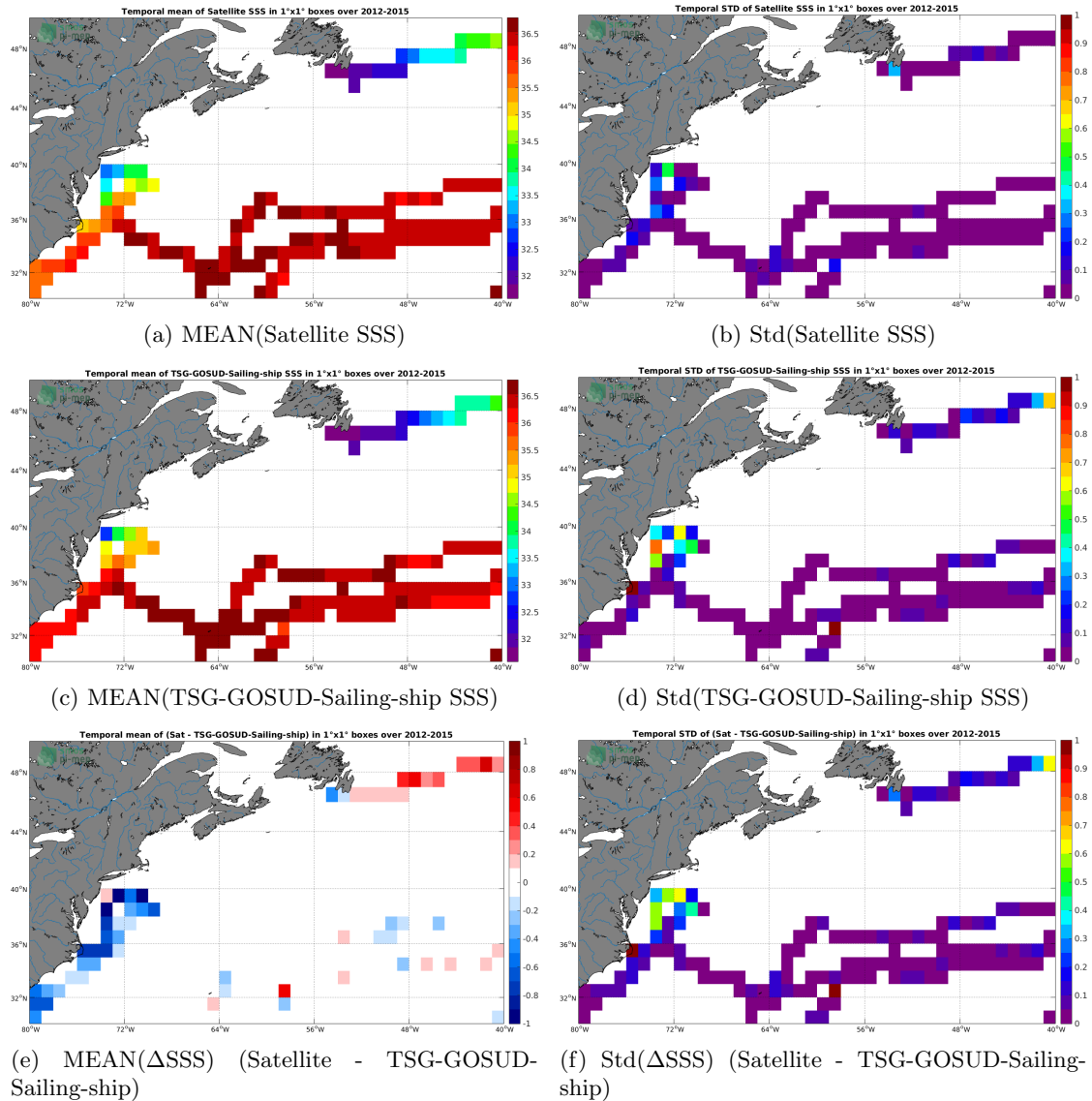
Figure 6: Temporal mean (left) and Std (right) of SSS from Aquarius-L4-IPRC-V5-WEEKLY (top), TSG-GOSUD-Sailing-ship (middle), and of \Delta SSS (Satellite - TSG-GOSUD-Sailing-ship). Only match-up pairs are used to generate these maps.
