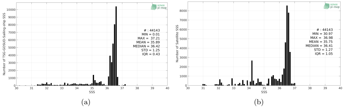
Figure 2: Histograms of SSS from TSG-GOSUD-Sailing-ship (a) and Aquarius-L4-IPRC-V5-WEEKLY (b) considering all match-up pairs per bins of 0.1 over the Gulf Stream Pi-MEP region and for the full satellite product period.
