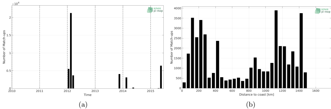
Figure 1: Number of match-ups between TSG-GOSUD-Sailing-ship and Aquarius-L4-IPRC-V5-WEEKLY SSS as a function of time (a) and as function of the distance to coast (b) over the Gulf Stream Pi-MEP region and for the full satellite product period.
