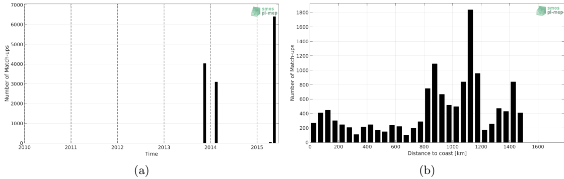
Figure 1: Number of match-ups between TSG-GOSUD-Sailing-ship and Aquarius-L4-IPRC-V5-WEEKLY SSS as a function of time (a) and as function of the distance to coast (b) over the Gulf Stream Pi-MEP region and for the full satellite product period.
