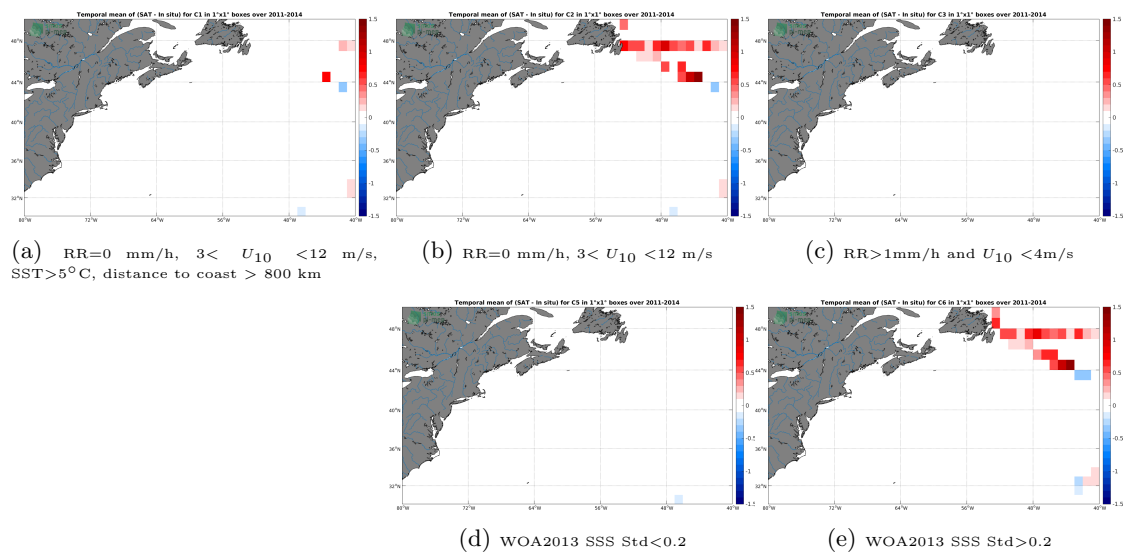
Figure 12: Temporal mean gridded over spatial boxes of size 1^\circ \times 1^\circ of \Delta SSS (Aquarius-L4-IPRC-V5-WEEKLY - TSG-GOSUD-Research-vessel) for 5 different subdatasets corresponding to: RR=0 mm/h, 3 < U_{10} < 12 m/s, SST > 5°C, distance to coast > 800 km (a), RR=0 mm/h, 3 < U_{10} < 12 m/s (b), RR > 1mm/h and U_{10} < 4 m/s (c), WOA2013 SSS Std < 0.2 (d), WOA2013 SSS Std > 0.2 (e).
