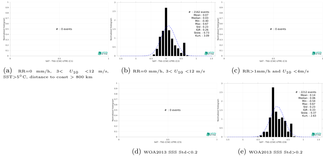
Figure 15: Normalized histogram of \Delta SSS (Aquarius SSS L4 OI v5 - Weekly (IPRC) - TSG (CSIC-UTM)) for 5 different subdatasets corresponding to: RR=0 mm/h, 3 < U_{10} < 12 m/s, SST >5^{\circ} C, distance to coast > 800 km (a), RR=0 mm/h, 3 < U_{10} < 12 m/s (b), RR >1 mm/h and U_{10} < 4 m/s (c), WOA2013 SSS Std <0.2 (d), WOA2013 SSS Std >0.2 (e).
