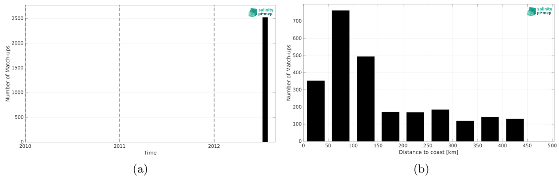
Figure 2: Number of match-ups between TSG (CSIC-UTM) and Aquarius SSS L4 OI v5 - Weekly (IPRC) SSS as a function of time (a) and as function of the distance to coast (b) over the Gulf Stream Pi-MEP region and for the full satellite product period.
