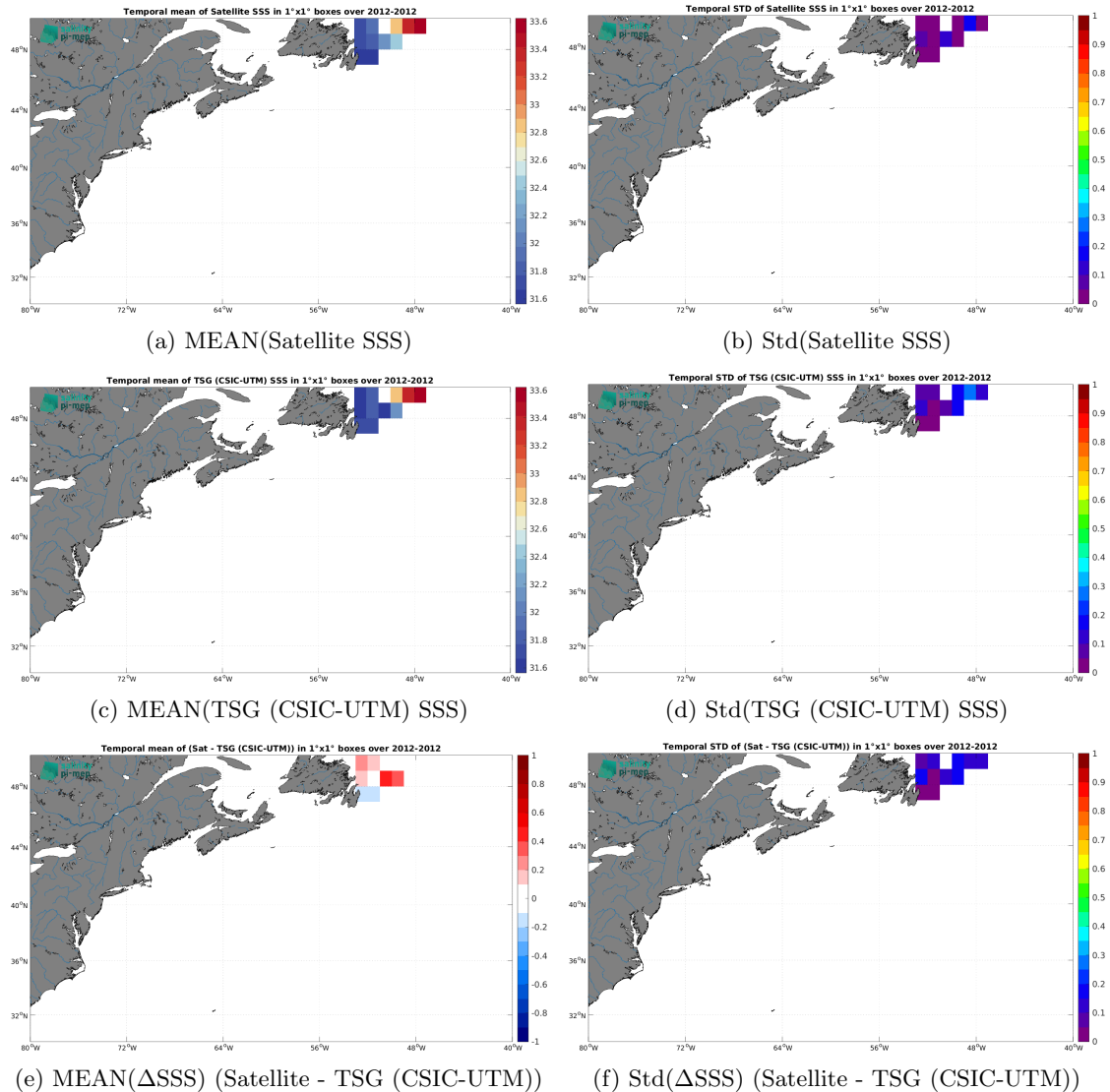
Figure 7: Temporal mean (left) and Std (right) of SSS from Aquarius SSS L4 OI v5 - Weekly (IPRC) (top), TSG (CSIC-UTM) (middle), and of \Delta SSS (Satellite - TSG (CSIC-UTM)). Only match-up pairs are used to generate these maps.
