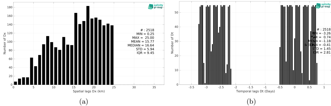
Figure 6: Histograms of the spatial (a) and temporal (b) lags between the location/time of the TSG (CSIC-UTM) measurement and the date of the corresponding Aquarius SSS L4 OI v5 - Weekly (IPRC) SSS pixel.
