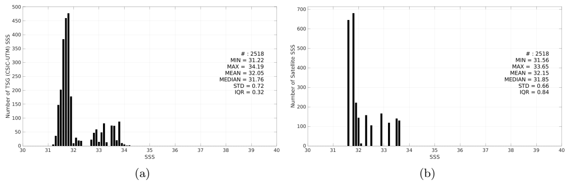
Figure 3: Histograms of SSS from TSG (CSIC-UTM) (a) and Aquarius SSS L4 OI v5 - Weekly (IPRC) (b) considering all match-up pairs per bins of 0.1 over the Gulf Stream Pi-MEP region and for the full satellite product period.
