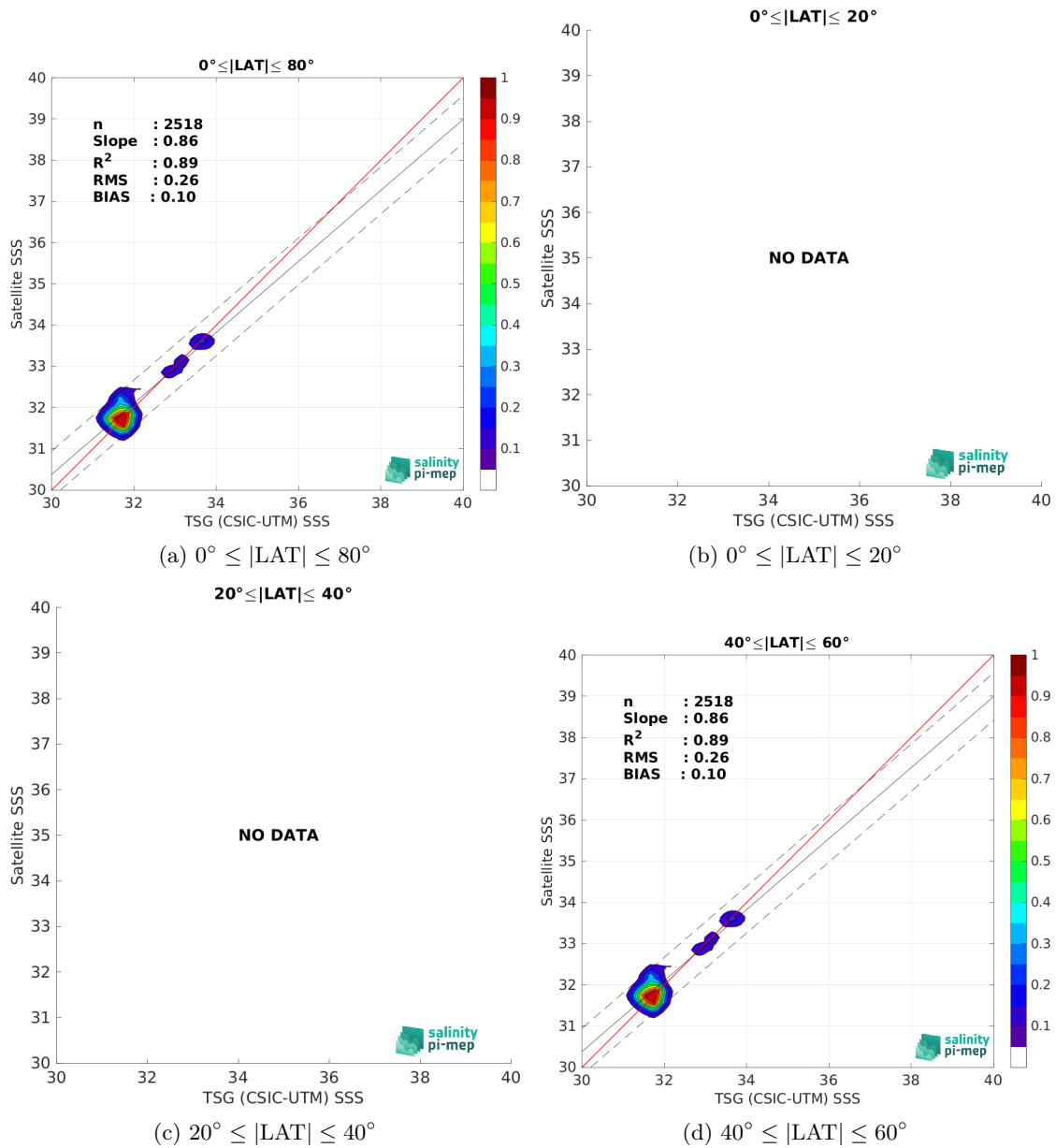
Figure 10: Contour maps of the concentration of Aquarius SSS L4 OI v5 - Weekly (IPRC) SSS (y-axis) versus TSG (CSIC-UTM) SSS (x-axis) at match-up pairs for different latitude bands. For each plot, the red line shows x=y . The black thin and dashed lines indicate a linear fit through the data cloud and the \pm 95\% confidence levels, respectively. The number match-up pairs n , the slope and R^2 coefficient of the linear fit, the root mean square (RMS) and the mean bias between satellite and in situ data are indicated for each latitude band in each plots.
