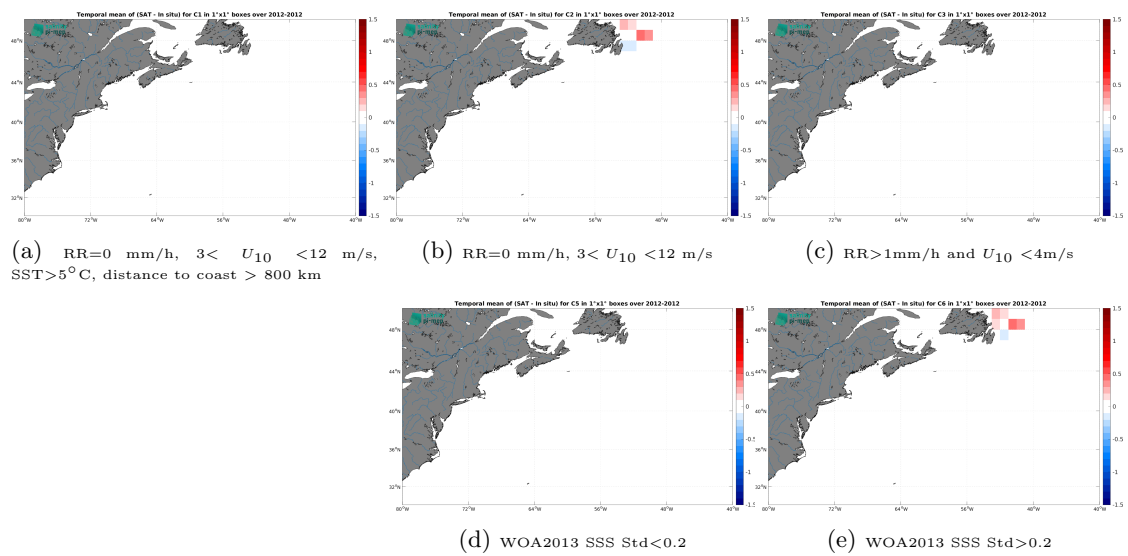
Figure 14: Temporal mean gridded over spatial boxes of size 1^\circ \times 1^\circ of \Delta SSS (Aquarius SSS L4 OI v5 - Weekly (IPRC) - TSG (CSIC-UTM)) for 5 different subdatasets corresponding to:RR=0 mm/h, 3 < U_{10} < 12 m/s, SST > 5°C, distance to coast > 800 km (a), RR=0 mm/h, 3 < U_{10} < 12 m/s (b), RR > 1mm/h and U_{10} < 4 m/s (c), WOA2013 SSS Std < 0.2 (d), WOA2013 SSS Std > 0.2 (e).
