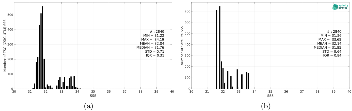
Figure 2: Histograms of SSS from TSG (CSIC-UTM) (a) and Aquarius SSS L4 OI v5 - Weekly (IPRC) (b) considering all match-up pairs per bins of 0.1 over the Gulf Stream Pi-MEP region and for the full satellite product period.
