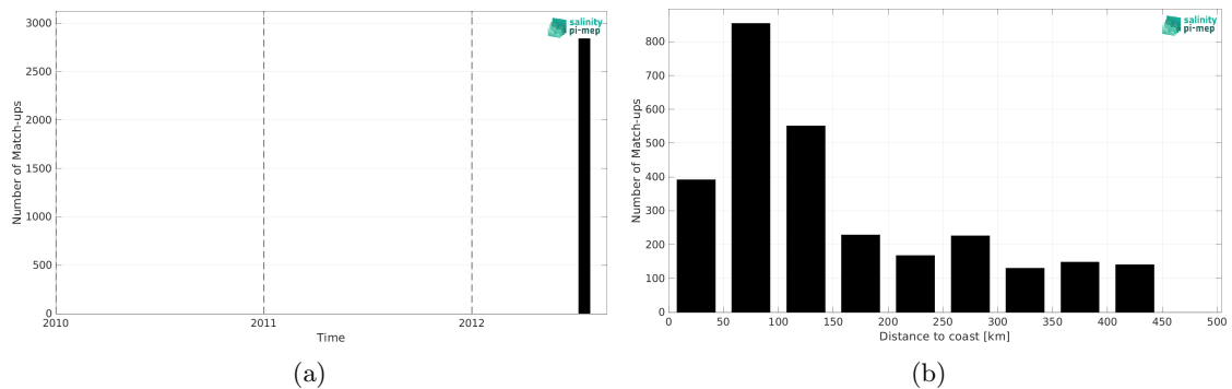
Figure 1: Number of match-ups between TSG (CSIC-UTM) and Aquarius SSS L4 OI v5 - Weekly (IPRC) SSS as a function of time (a) and as function of the distance to coast (b) over the Gulf Stream Pi-MEP region and for the full satellite product period.
