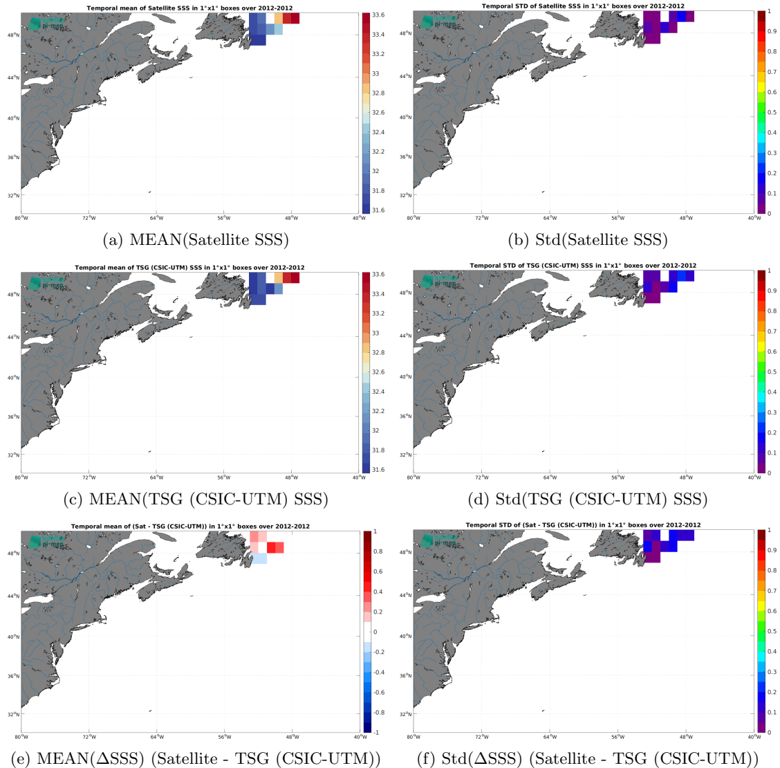
Figure 6: Temporal mean (left) and Std (right) of SSS from Aquarius SSS L4 OI v5 - Weekly (IPRC) (top), TSG (CSIC-UTM) (middle), and of \Delta SSS (Satellite - TSG (CSIC-UTM)). Only match-up pairs are used to generate these maps.
