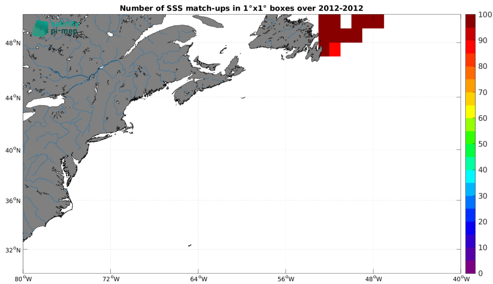
Figure 4: Number of SSS match-ups between TSG (CSIC-UTM) SSS and the Aquarius SSS L4 OI v5 - Weekly (IPRC) SSS product for the Gulf Stream Pi-MEP region over 1^\circ \times 1^\circ boxes and for the full satellite product period.
