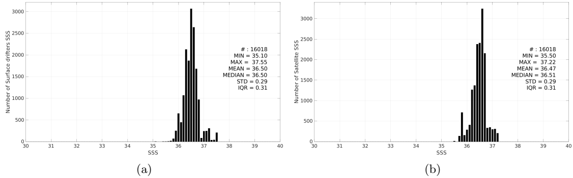
Figure 3: Histograms of SSS from Surface drifters (a) and Aquarius SSS L4 OI v5 - Weekly (IPRC) (b) considering all match-up pairs per bins of 0.1 over the Gulf Stream Pi-MEP region and for the full satellite product period.
