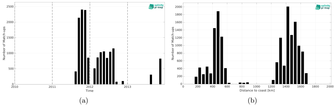
Figure 2: Number of match-ups between Surface drifters and Aquarius SSS L4 OI v5 - Weekly (IPRC) SSS as a function of time (a) and as function of the distance to coast (b) over the Gulf Stream Pi-MEP region and for the full satellite product period.
