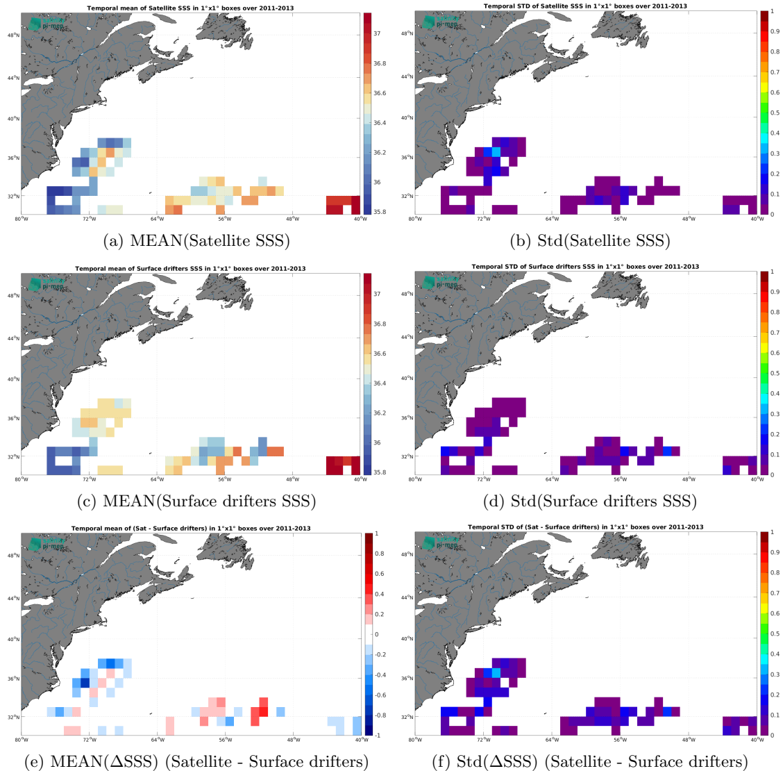
Figure 6: Temporal mean (left) and Std (right) of SSS from Aquarius SSS L4 OI v5 - Weekly (IPRC) (top), Surface drifters (middle), and of \Delta SSS (Satellite - Surface drifters). Only match-up pairs are used to generate these maps.
