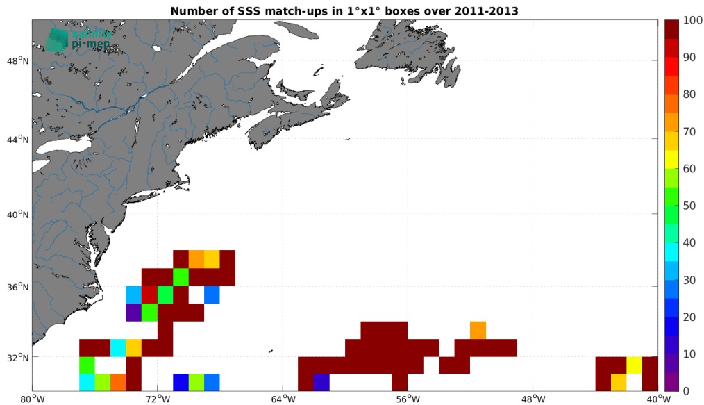
Figure 4: Number of SSS match-ups between Surface drifters SSS and the Aquarius SSS L4 OI v5 - Weekly (IPRC) SSS product for the Gulf Stream Pi-MEP region over 1^\circ \times 1^\circ boxes and for the full satellite product period.
