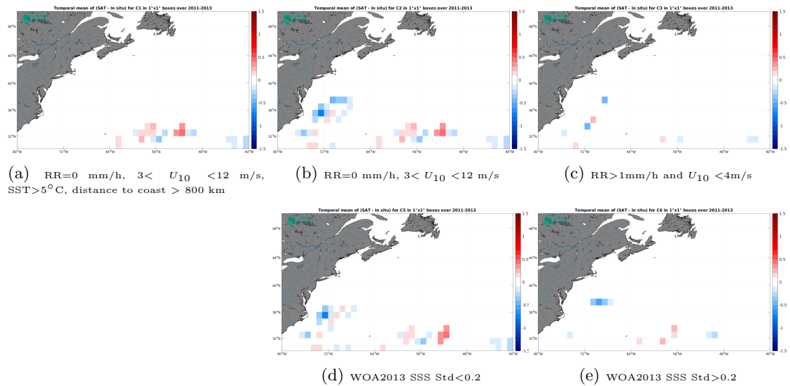
Figure 13: Temporal mean gridded over spatial boxes of size 1^\circ \times 1^\circ of \Delta SSS (Aquarius SSS L4 OI v5 - Weekly (IPRC) - Surface drifters) for 5 different subdatasets corresponding to:RR=0 mm/h, 3 < U_{10} < 12 m/s, SST >5^\circ C, distance to coast > 800 km (a), RR=0 mm/h, 3 < U_{10} < 12 m/s (b), RR >1 mm/h and U_{10} < 4 m/s (c), WOA2013 SSS Std <0.2 (d), WOA2013 SSS Std >0.2 (e).
