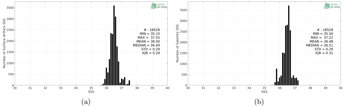
Figure 2: Histograms of SSS from Surface drifters (a) and Aquarius SSS L4 OI v5 - Weekly (IPRC) (b) considering all match-up pairs per bins of 0.1 over the Gulf Stream Pi-MEP region and for the full satellite product period.
