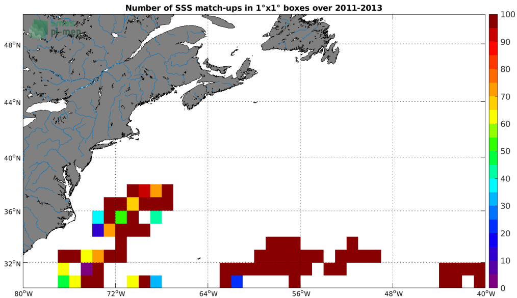
Figure 3: Number of SSS match-ups between Surface drifters SSS and the Aquarius SSS L4 OI v5 - Weekly (IPRC) SSS product for the Gulf Stream Pi-MEP region over 1^\circ \times 1^\circ boxes and for the full satellite product period.
