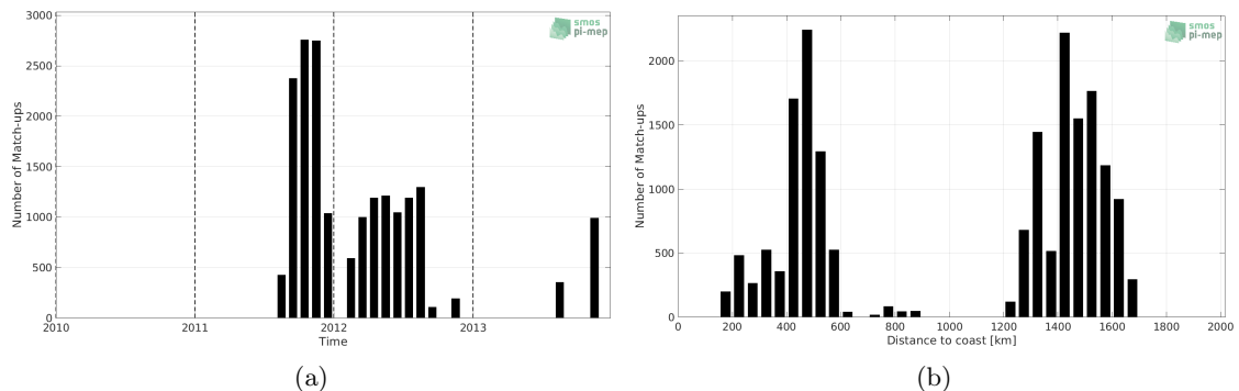
Figure 1: Number of match-ups between Surface drifters and Aquarius SSS L4 OI v5 - Weekly (IPRC) SSS as a function of time (a) and as function of the distance to coast (b) over the Gulf Stream Pi-MEP region and for the full satellite product period.
