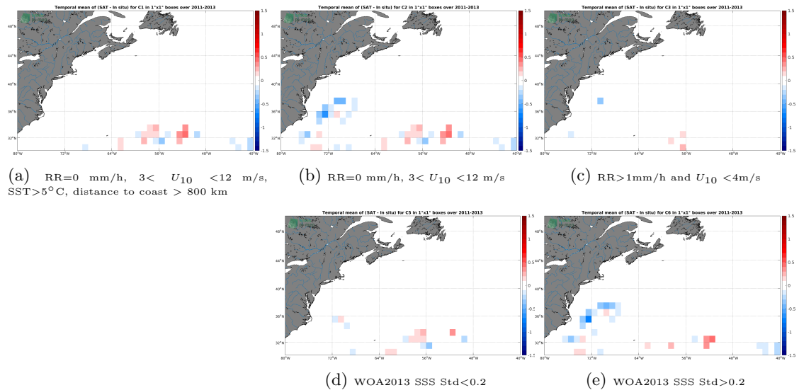
Figure 11: Temporal mean gridded over spatial boxes of size 1^{\circ}\times 1^{\circ} of \Delta\text{SSS} (Aquarius SSS L4 OI v5 - Weekly (IPRC) - Surface drifters) for 5 different subdatasets corresponding to:RR=0 mm/h, 3 < U_{10} < 12 m/s, SST >5^{\circ}\text{C} , distance to coast > 800 km (a), RR=0 mm/h, 3 < U_{10} < 12 m/s (b), RR >1 mm/h and U_{10} < 4 m/s (c), WOA2013 SSS Std <0.2 (d), WOA2013 SSS Std >0.2 (e).
