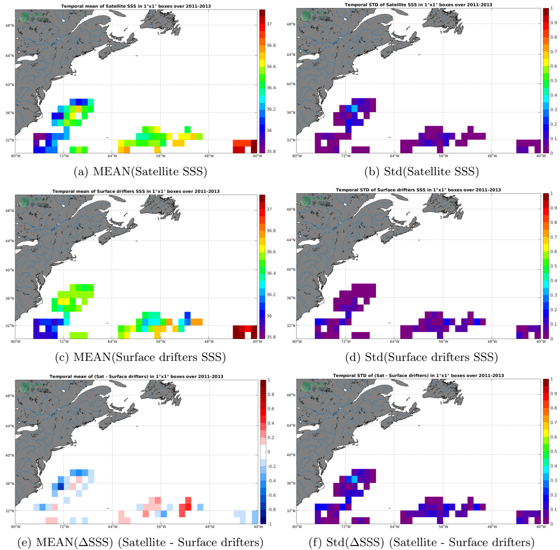
Figure 5: Temporal mean (left) and Std (right) of SSS from Aquarius SSS L4 OI v5 - Weekly (IPRC) (top), Surface drifters (middle), and of \Delta\text{SSS} (Satellite - Surface drifters). Only match-up pairs are used to generate these maps.
