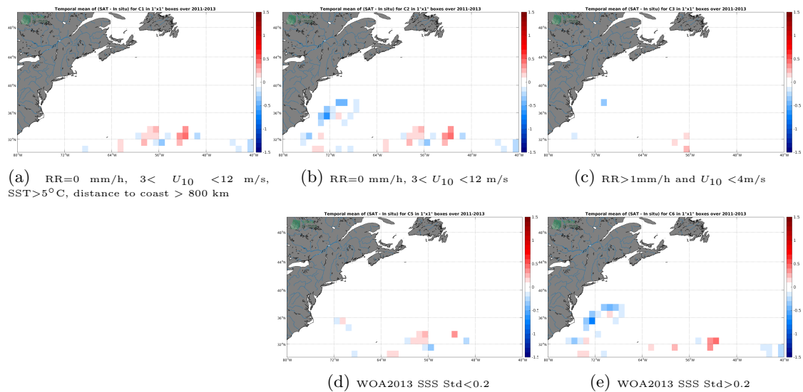
Figure 11: Temporal mean gridded over spatial boxes of size 1^{\circ}\times 1^{\circ} of \Delta\text{SSS} (Aquarius-L4-IPRC-V5-WEEKLY - Surface drifters) for 5 different subdatasets corresponding to:RR=0 mm/h, 3 < U_{10} < 12 m/s, SST >5^{\circ}\text{C} , distance to coast > 800 km (a), RR=0 mm/h, 3 < U_{10} < 12 m/s (b), RR >1 mm/h and U_{10} < 4 m/s (c), WOA2013 SSS Std <0.2 (d), WOA2013 SSS Std >0.2 (e).
