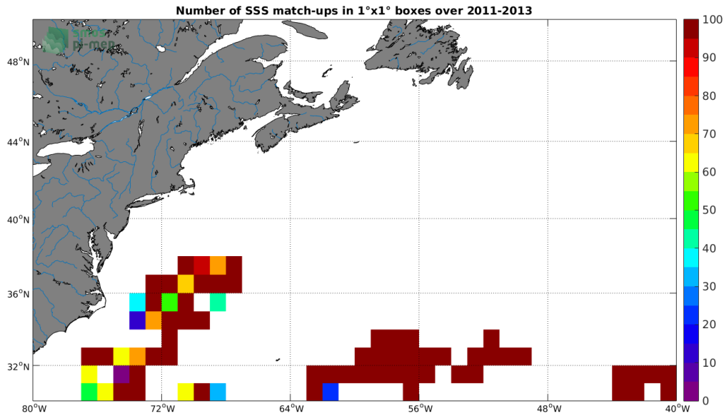
Figure 3: Number of SSS match-ups between Surface drifters SSS and the Aquarius-L4-IPRC-V5-WEEKLY SSS product for the Gulf Stream Pi-MEP region over 1^\circ \times 1^\circ boxes and for the full satellite product period.
