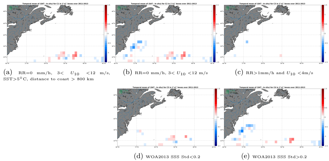
Figure 11: Temporal mean gridded over spatial boxes of size 1^\circ \times 1^\circ of \Delta SSS (Aquarius-L4-IPRC-V5-WEEKLY - Surface drifters) for 5 different subdatasets corresponding to:RR=0 mm/h, 3 < U_{10} < 12 m/s, SST >5^\circ\text{C} , distance to coast > 800 km (a), RR=0 mm/h, 3 < U_{10} < 12 m/s (b), RR >1 mm/h and U_{10} < 4 m/s (c), WOA2013 SSS Std <0.2 (d), WOA2013 SSS Std >0.2 (e).
