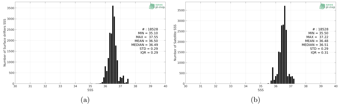
Figure 2: Histograms of SSS from Surface drifters (a) and Aquarius-L4-IPRC-V5-WEEKLY (b) considering all match-up pairs per bins of 0.1 over the Gulf Stream Pi-MEP region and for the full satellite product period.
