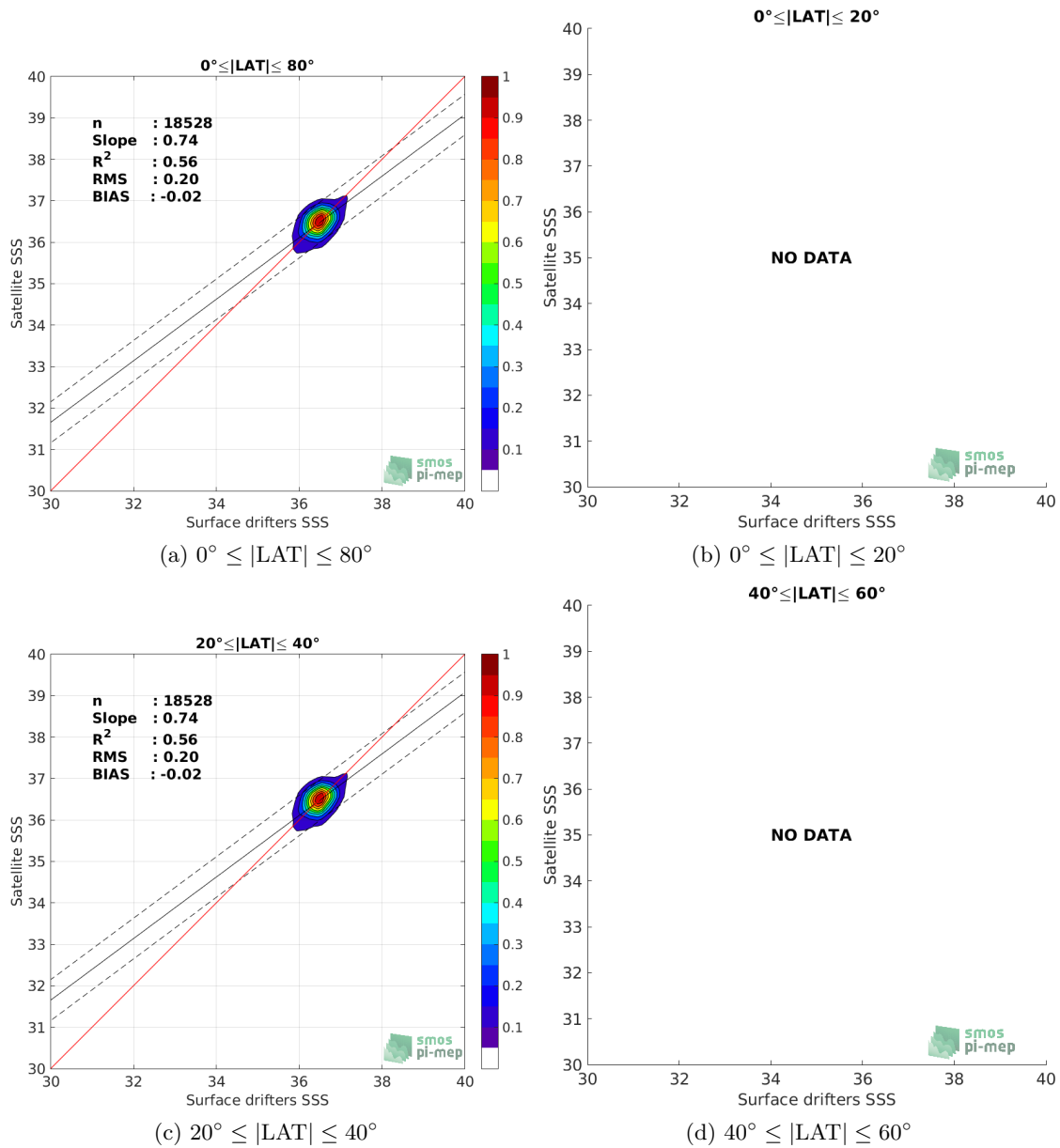
Figure 8: Contour maps of the concentration of Aquarius-L4-IPRC-V5-WEEKLY SSS (y-axis) versus Surface drifters SSS (x-axis) at match-up pairs for different latitude bands. For each plot, the red line shows x=y . The black thin and dashed lines indicate a linear fit through the data cloud and the \pm 95\% confidence levels, respectively. The number match-up pairs n , the slope and R^2 coefficient of the linear fit, the root mean square (RMS) and the mean bias between satellite and in situ data are indicated for each latitude band in each plots.
