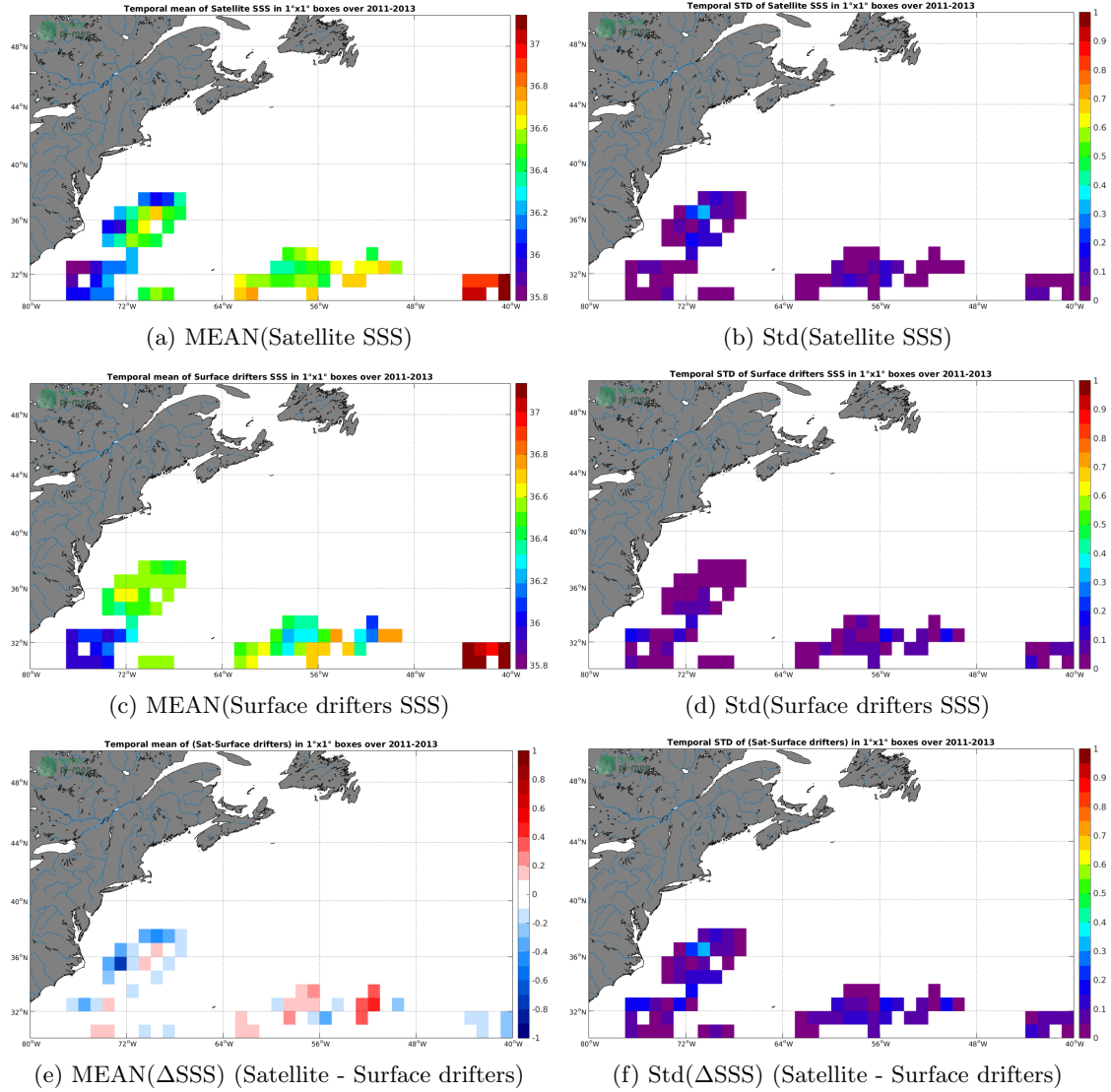
Figure 5: Temporal mean (left) and Std (right) of SSS from Aquarius-L4-IPRC-V5-WEEKLY (top), Surface drifters (middle), and of \Delta\text{SSS} (Satellite - Surface drifters). Only match-up pairs are used to generate these maps.
