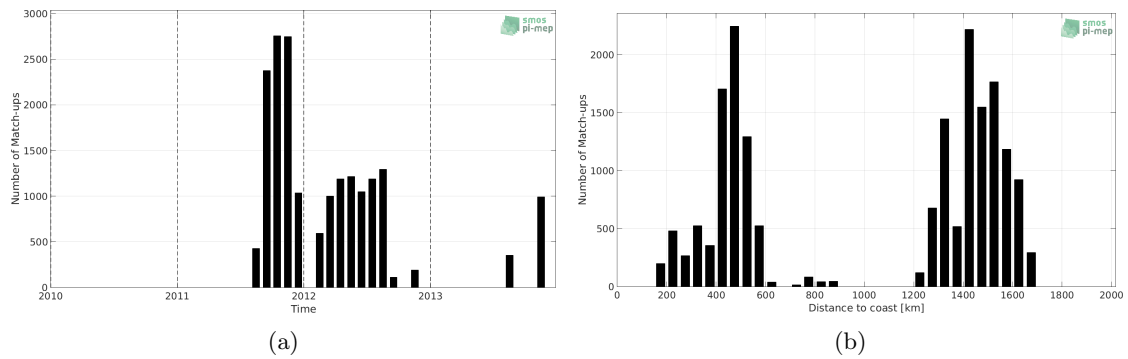
Figure 1: Number of match-ups between Surface drifters and Aquarius-L4-IPRC-V5-WEEKLY SSS as a function of time (a) and as function of the distance to coast (b) over the Gulf Stream Pi-MEP region and for the full satellite product period.
