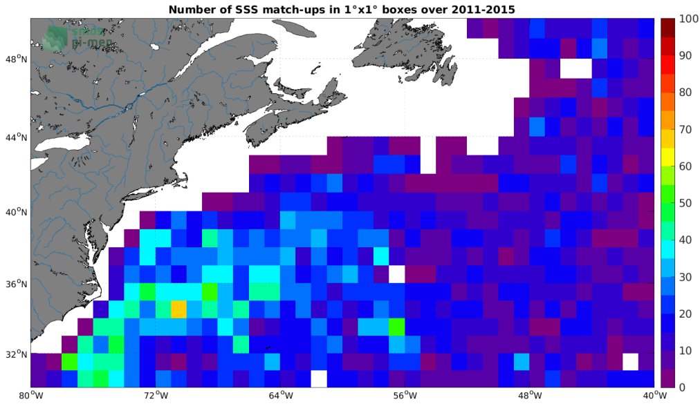
Figure 4: Number of SSS match-ups between Argo SSS and the Aquarius SSS L4 OI v5 - Weekly (IPRC) SSS product for the Gulf Stream Pi-MEP region over 1^{\circ} \times 1^{\circ} boxes and for the full satellite product period.
