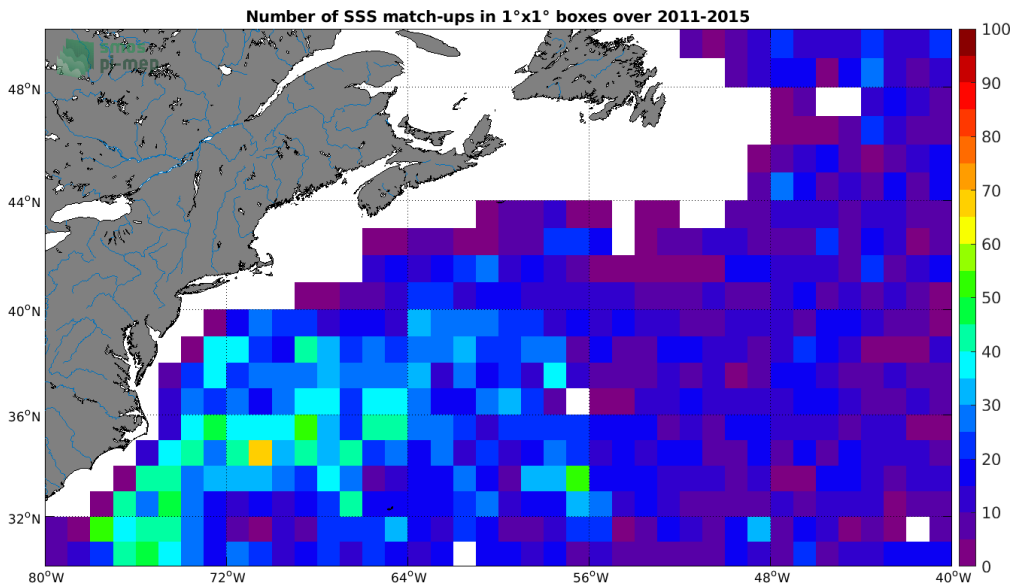
Figure 4: Number of SSS match-ups between Argo SSS and the Aquarius SSS L4 OI v5 - Weekly (IPRC) SSS product for the Gulf Stream Pi-MEP region over 1°x1° boxes and for the full satellite product period.
