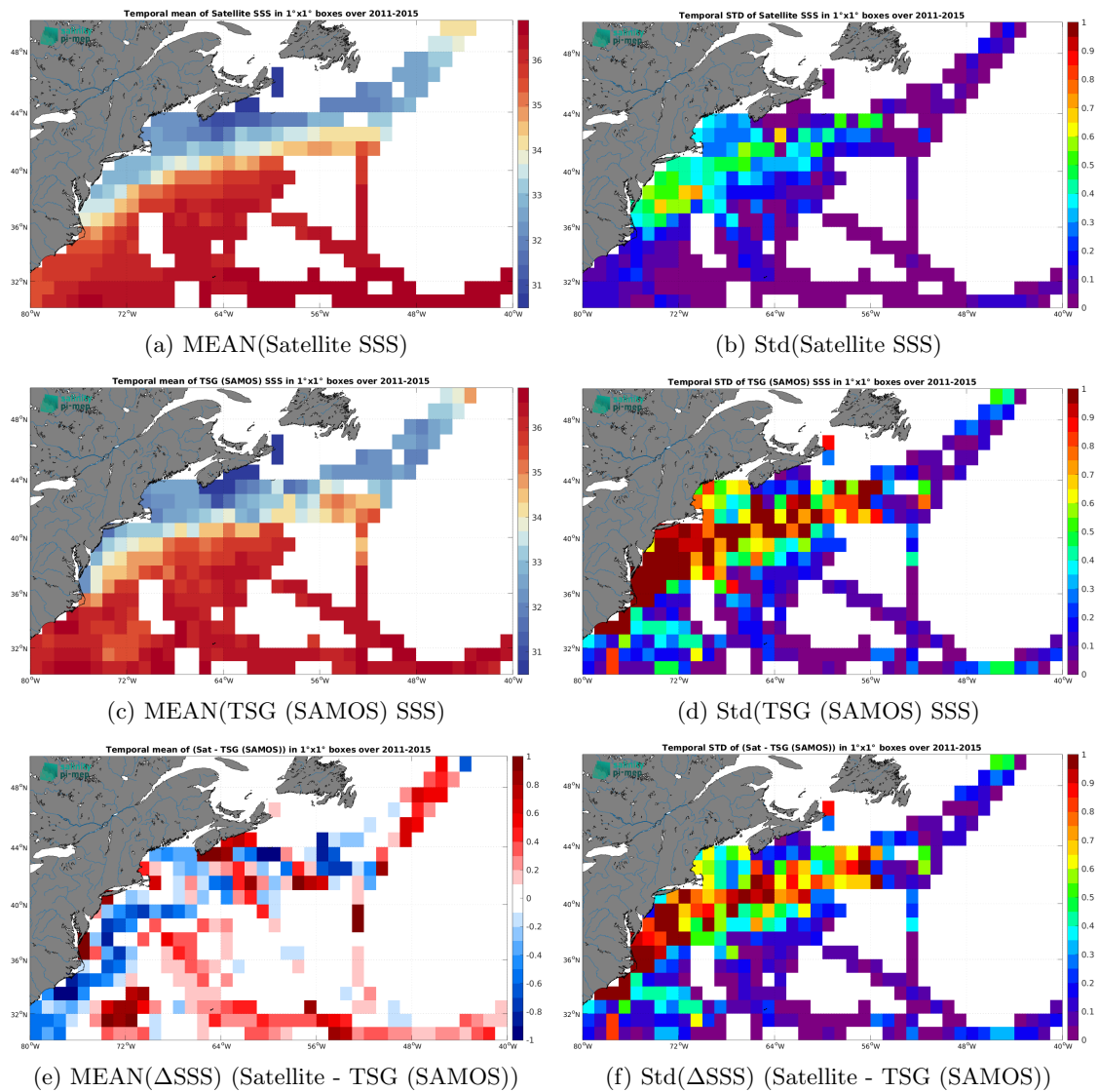
Figure 7: Temporal mean (left) and Std (right) of SSS from Aquarius SSS L4 OI v5 - Monthly (IPRC) (top), TSG (SAMOS) (middle), and of \Delta SSS (Satellite - TSG (SAMOS)). Only match-up pairs are used to generate these maps.
