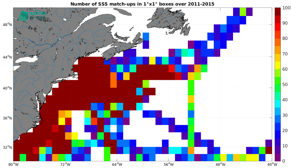
Figure 5: Number of SSS match-ups between TSG (SAMOS) SSS and the Aquarius SSS L4 OI v5 - Monthly (IPRC) SSS product for the Gulf Stream Pi-MEP region over 1^\circ \times 1^\circ boxes and for the full satellite product period.
