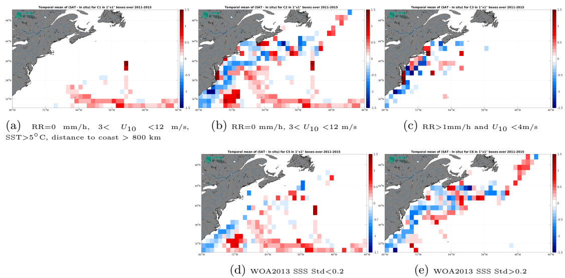
Figure 14: Temporal mean gridded over spatial boxes of size 1^\circ \times 1^\circ of \Delta\text{SSS} (Aquarius SSS L4 OI v5 - Monthly (IPRC) - TSG (SAMOS)) for 5 different subdatasets corresponding to:RR=0 mm/h, 3 < U_{10} < 12 m/s, SST > 5°C, distance to coast > 800 km (a), RR=0 mm/h, 3 < U_{10} < 12 m/s (b), RR > 1mm/h and U_{10} < 4 m/s (c), WOA2013 SSS Std < 0.2 (d), WOA2013 SSS Std > 0.2 (e).
