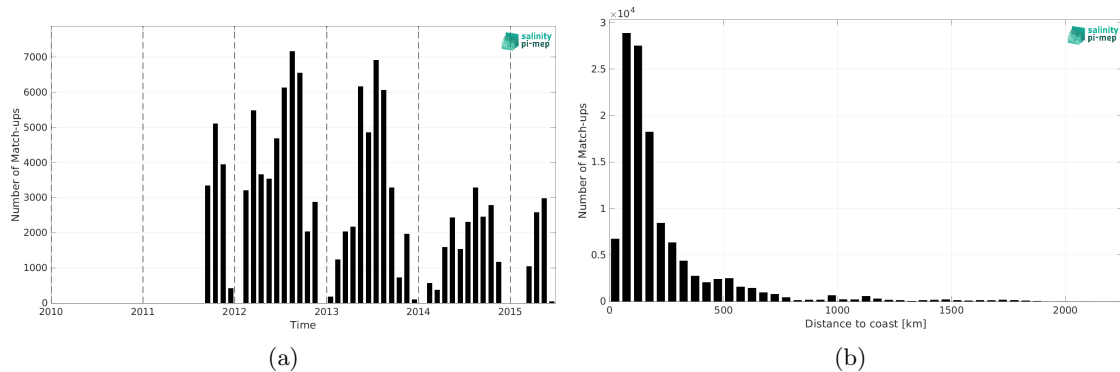
Figure 2: Number of match-ups between TSG (SAMOS) and Aquarius SSS L4 OI v5 - Monthly (IPRC) SSS as a function of time (a) and as function of the distance to coast (b) over the Gulf Stream Pi-MEP region and for the full satellite product period.
