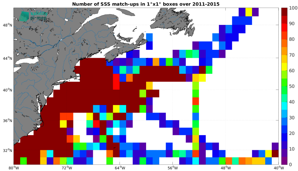
Figure 4: Number of SSS match-ups between TSG (SAMOS) SSS and the Aquarius SSS L4 OI v5 - Monthly (IPRC) SSS product for the Gulf Stream Pi-MEP region over 1^\circ \times 1^\circ boxes and for the full satellite product period.
