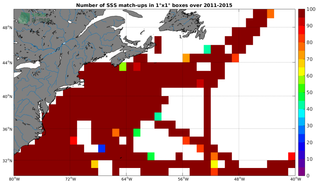
Figure 4: Number of SSS match-ups between TSG-SAMOS SSS and the Aquarius-L4-IPRC-V5-MONTHLY SSS product for the Gulf Stream Pi-MEP region over 1°x1° boxes and for the full satellite product period.
