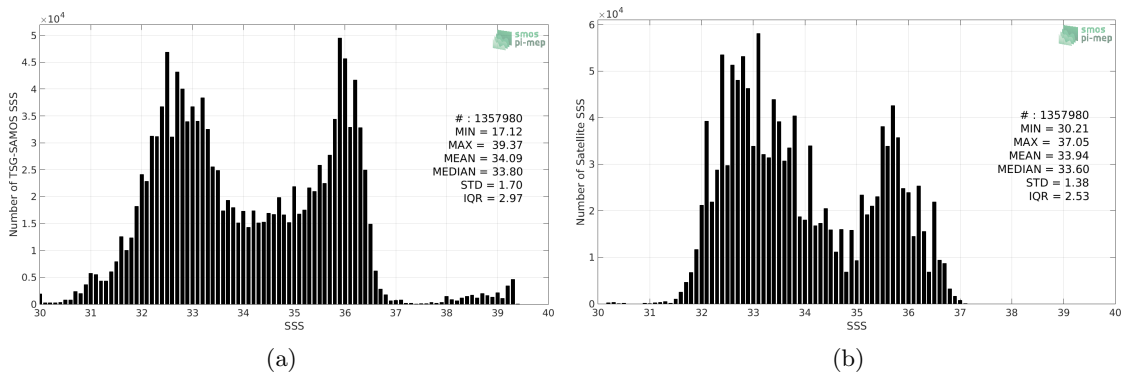
Figure 2: Histograms of SSS from TSG-SAMOS (a) and Aquarius-L4-IPRC-V5-MONTHLY (b) considering all match-up pairs per bins of 0.1 over the Gulf Stream Pi-MEP region and for the full satellite product period.
