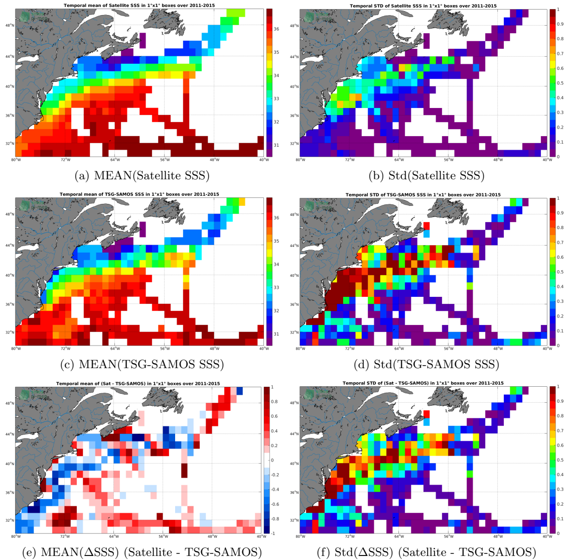
Figure 6: Temporal mean (left) and Std (right) of SSS from Aquarius-L4-IPRC-V5-MONTHLY (top), TSG-SAMOS (middle), and of \Delta SSS (Satellite - TSG-SAMOS). Only match-up pairs are used to generate these maps.
