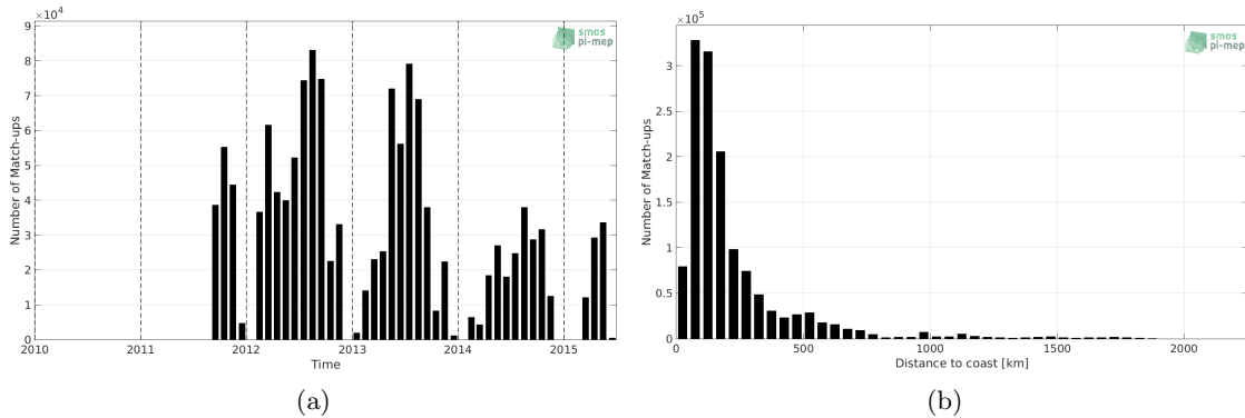
Figure 1: Number of match-ups between TSG-SAMOS and Aquarius-L4-IPRC-V5-MONTHLY SSS as a function of time (a) and as function of the distance to coast (b) over the Gulf Stream Pi-MEP region and for the full satellite product period.
