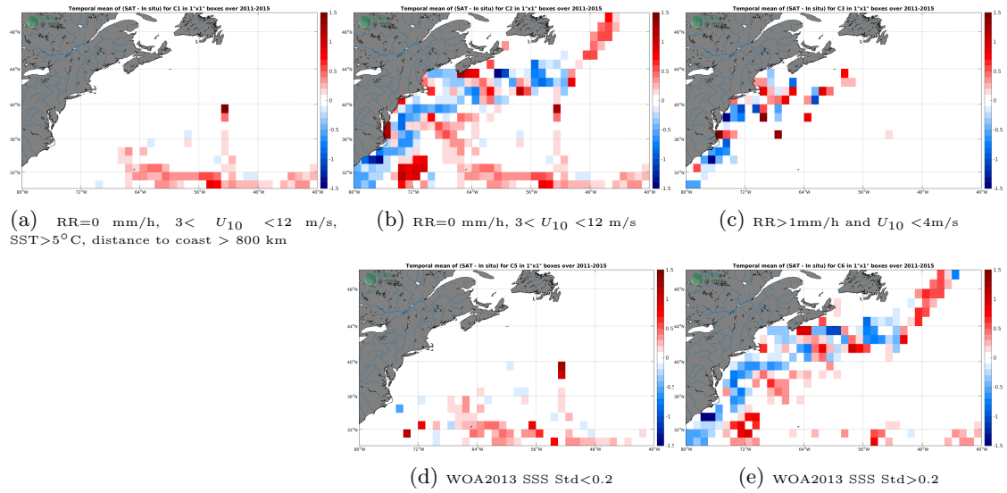
Figure 12: Temporal mean gridded over spatial boxes of size 1^\circ \times 1^\circ of \Delta SSS (Aquarius-L4-IPRC-V5-MONTHLY - TSG-SAMOS) for 5 different subdatasets corresponding to:RR=0 mm/h, 3 < U_{10} < 12 m/s, SST >5^\circ C, distance to coast > 800 km (a), RR=0 mm/h, 3 < U_{10} < 12 m/s (b), RR >1 mm/h and U_{10} < 4 m/s (c), WOA2013 SSS Std <0.2 (d), WOA2013 SSS Std >0.2 (e).
