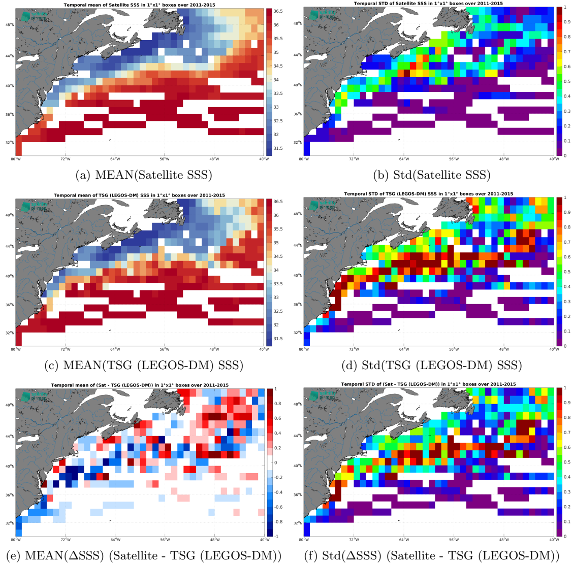
Figure 7: Temporal mean (left) and Std (right) of SSS from Aquarius SSS L4 OI v5 - Monthly (IPRC) (top), TSG (LEGOS-DM) (middle), and of \Delta SSS (Satellite - TSG (LEGOS-DM)). Only match-up pairs are used to generate these maps.
