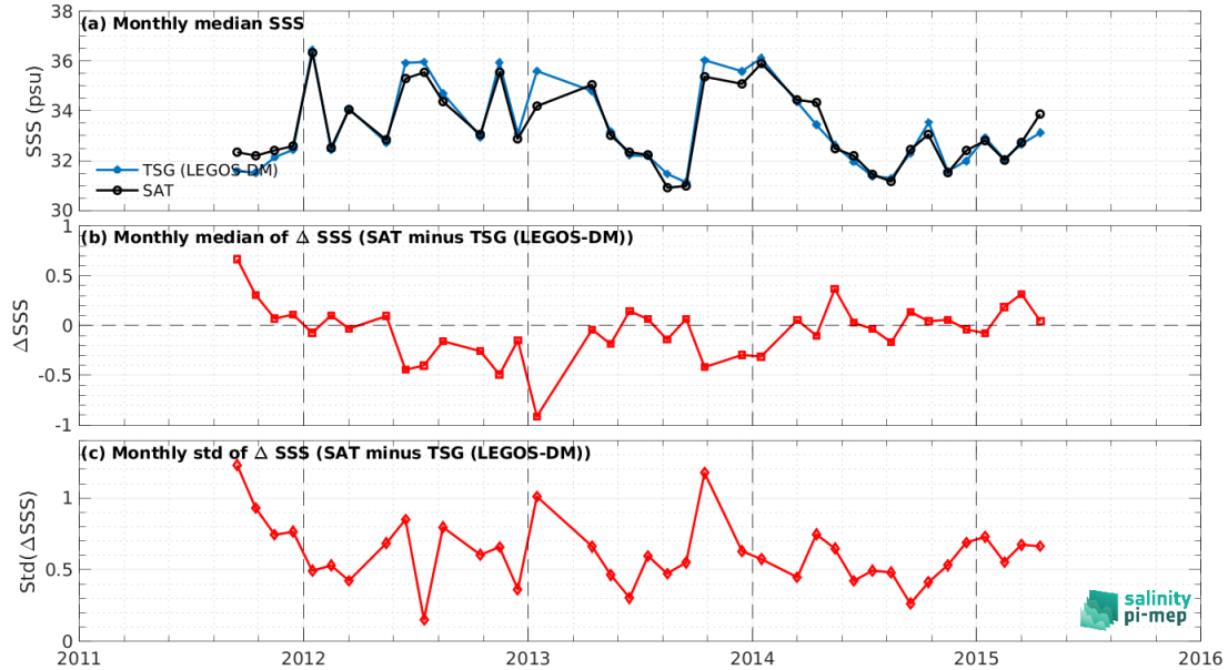
Figure 8: Time series of the monthly median SSS (top), median of \Delta\text{SSS} (Satellite - TSG (LEGOS-DM)) and Std of \Delta\text{SSS} (Satellite - TSG (LEGOS-DM)) over the Gulf Stream Pi-MEP region considering all match-ups collected by the Pi-MEP.
