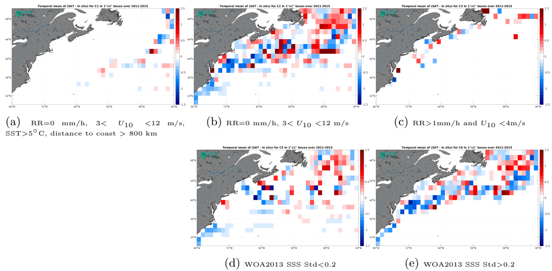
Figure 14: Temporal mean gridded over spatial boxes of size 1^\circ \times 1^\circ of \Delta SSS (Aquarius SSS L4 OI v5 - Monthly (IPRC) - TSG (LEGOS-DM)) for 5 different subdatasets corresponding to:RR=0 mm/h, 3 < U_{10} < 12 m/s, SST > 5°C, distance to coast > 800 km (a), RR=0 mm/h, 3 < U_{10} < 12 m/s (b), RR > 1mm/h and U_{10} < 4 m/s (c), WOA2013 SSS Std < 0.2 (d), WOA2013 SSS Std > 0.2 (e).
