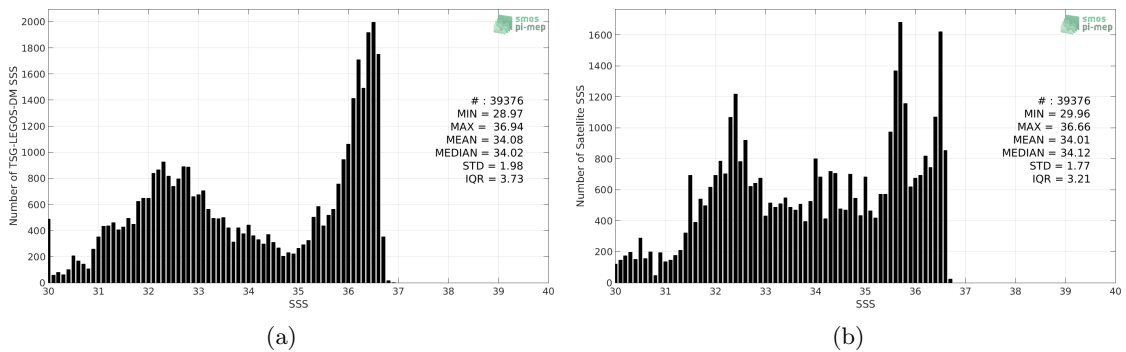
Figure 2: Histograms of SSS from TSG-LEGOS-DM (a) and Aquarius-L4-IPRC-V5-MONTHLY (b) considering all match-up pairs per bins of 0.1 over the Gulf Stream Pi-MEP region and for the full satellite product period.
