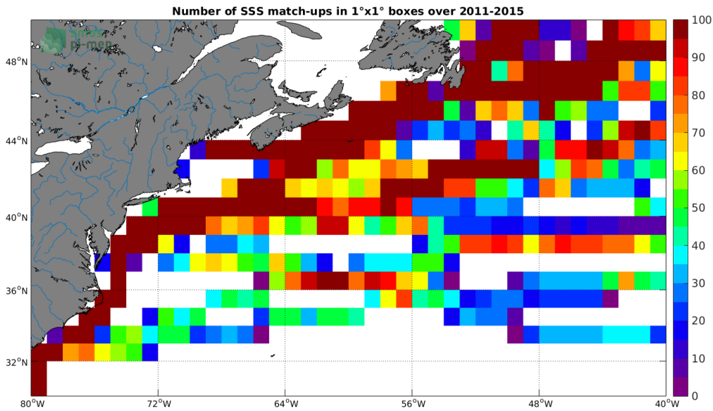
Figure 4: Number of SSS match-ups between TSG-LEGOS-DM SSS and the Aquarius-L4-IPRC-V5-MONTHLY SSS product for the Gulf Stream Pi-MEP region over 1^\circ \times 1^\circ boxes and for the full satellite product period.
