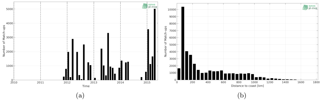
Figure 1: Number of match-ups between TSG-LEGOS-DM and Aquarius-L4-IPRC-V5-MONTHLY SSS as a function of time (a) and as function of the distance to coast (b) over the Gulf Stream Pi-MEP region and for the full satellite product period.
