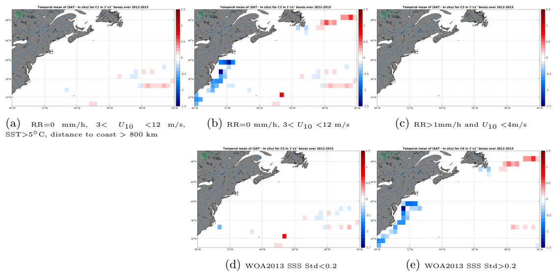
Figure 12: Temporal mean gridded over spatial boxes of size 1°x1° of \Delta SSS (Aquarius SSS L4 OI v5 - Monthly (IPRC) - TSG (GOSUD-Sailing-ship)) for 5 different subdatasets corresponding to: RR=0 mm/h, 3 < U_{10} < 12 m/s, SST > 5°C, distance to coast > 800 km (a), RR=0 mm/h, 3 < U_{10} < 12 m/s (b), RR > 1mm/h and U_{10} < 4 m/s (c), WOA2013 SSS Std < 0.2 (d), WOA2013 SSS Std > 0.2 (e).
