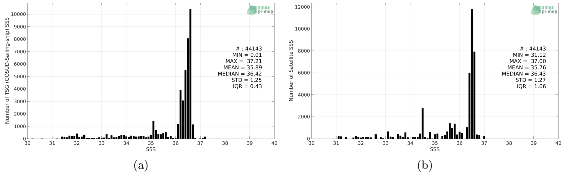
Figure 2: Histograms of SSS from TSG (GOSUD-Sailing-ship) (a) and Aquarius SSS L4 OI v5 - Monthly (IPRC) (b) considering all match-up pairs per bins of 0.1 over the Gulf Stream Pi-MEP region and for the full satellite product period.
