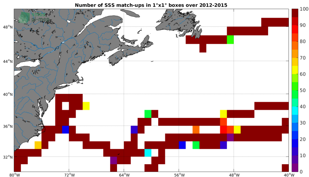
Figure 4: Number of SSS match-ups between TSG-GOSUD-Sailing-ship SSS and the Aquarius-L4-IPRC-V5-MONTHLY SSS product for the Gulf Stream Pi-MEP region over 1^\circ \times 1^\circ boxes and for the full satellite product period.
