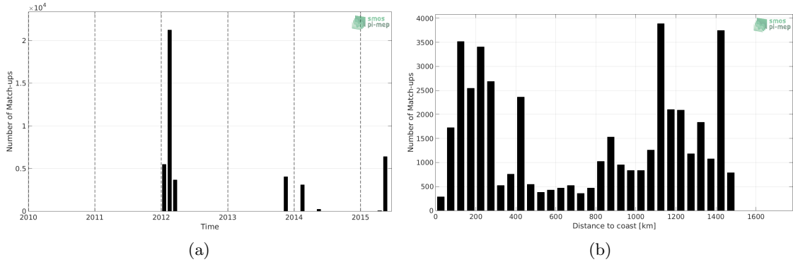
Figure 1: Number of match-ups between TSG-GOSUD-Sailing-ship and Aquarius-L4-IPRC-V5-MONTHLY SSS as a function of time (a) and as function of the distance to coast (b) over the Gulf Stream Pi-MEP region and for the full satellite product period.
