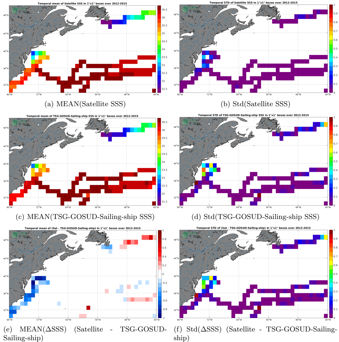
Figure 6: Temporal mean (left) and Std (right) of SSS from Aquarius-L4-IPRC-V5-MONTHLY (top), TSG-GOSUD-Sailing-ship (middle), and of \Delta SSS (Satellite - TSG-GOSUD-Sailing-ship). Only match-up pairs are used to generate these maps.
