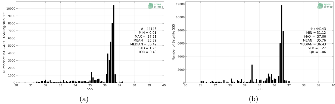
Figure 2: Histograms of SSS from TSG-GOSUD-Sailing-ship (a) and Aquarius-L4-IPRC-V5-MONTHLY (b) considering all match-up pairs per bins of 0.1 over the Gulf Stream Pi-MEP region and for the full satellite product period.
