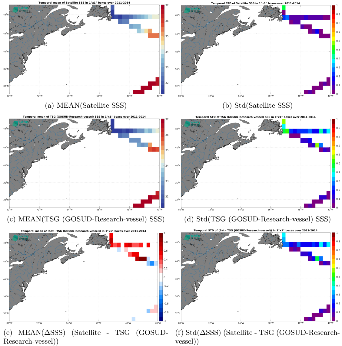
Figure 7: Temporal mean (left) and Std (right) of SSS from Aquarius SSS L4 OI v5 - Monthly (IPRC) (top), TSG (GOSUD-Research-vessel) (middle), and of \Delta SSS (Satellite - TSG (GOSUD-Research-vessel)). Only match-up pairs are used to generate these maps.
