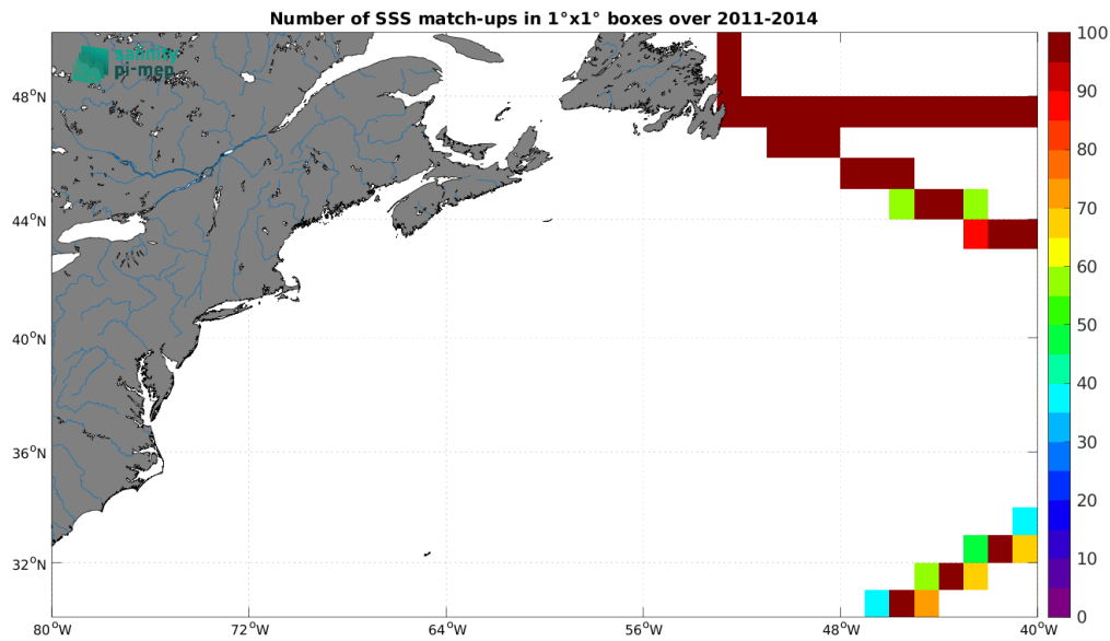
Figure 5: Number of SSS match-ups between TSG (GOSUD-Research-vessel) SSS and the Aquarius SSS L4 OI v5 - Monthly (IPRC) SSS product for the Gulf Stream Pi-MEP region over 1^\circ \times 1^\circ boxes and for the full satellite product period.
