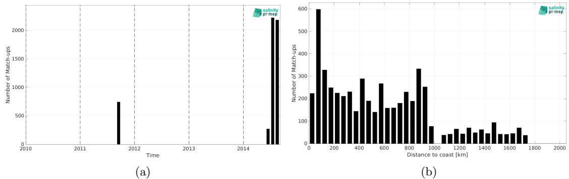
Figure 2: Number of match-ups between TSG (GOSUD-Research-vessel) and Aquarius SSS L4 OI v5 - Monthly (IPRC) SSS as a function of time (a) and as function of the distance to coast (b) over the Gulf Stream Pi-MEP region and for the full satellite product period.
