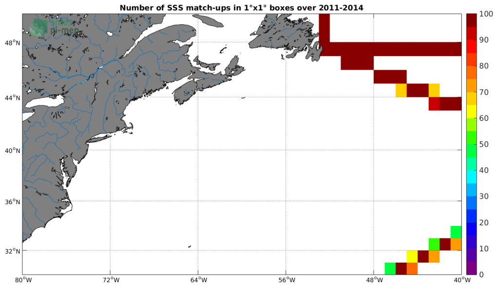
Figure 4: Number of SSS match-ups between TSG-GOSUD-Research-vessel SSS and the Aquarius-L4-IPRC-V5-MONTHLY SSS product for the Gulf Stream Pi-MEP region over 1°x1° boxes and for the full satellite product period.
