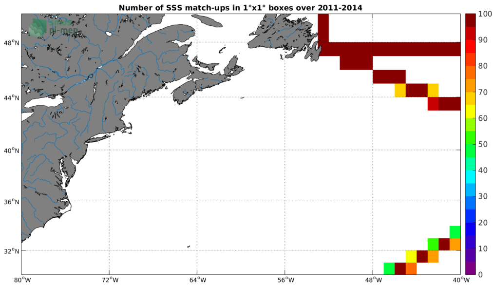
Figure 4: Number of SSS match-ups between TSG-GOSUD-Research-vessel SSS and the Aquarius-L4-IPRC-V5-MONTHLY SSS product for the Gulf Stream Pi-MEP region over 1^\circ \times 1^\circ boxes and for the full satellite product period.
