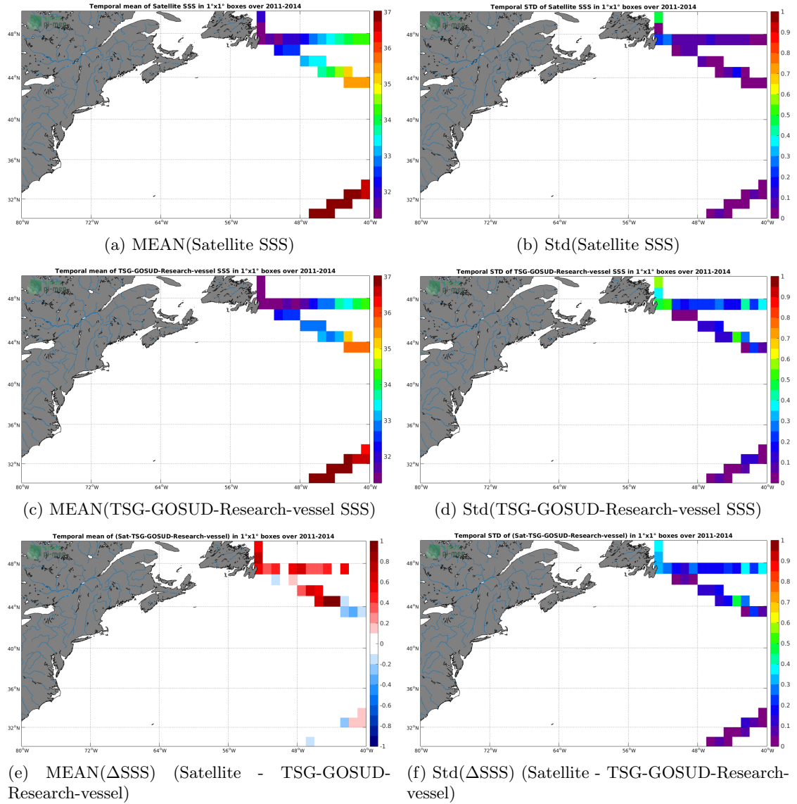
Figure 6: Temporal mean (left) and Std (right) of SSS from Aquarius-L4-IPRC-V5-MONTHLY (top), TSG-GOSUD-Research-vessel (middle), and of \Delta SSS (Satellite - TSG-GOSUD-Research-vessel). Only match-up pairs are used to generate these maps.
