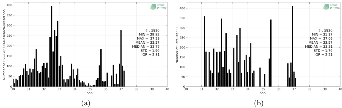
Figure 2: Histograms of SSS from TSG-GOSUD-Research-vessel (a) and Aquarius-L4-IPRC-V5-MONTHLY (b) considering all match-up pairs per bins of 0.1 over the Gulf Stream Pi-MEP region and for the full satellite product period.
