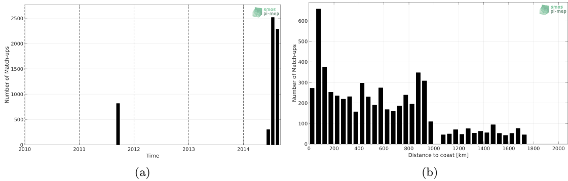
Figure 1: Number of match-ups between TSG-GOSUD-Research-vessel and Aquarius-L4-IPRC-V5-MONTHLY SSS as a function of time (a) and as function of the distance to coast (b) over the Gulf Stream Pi-MEP region and for the full satellite product period.
