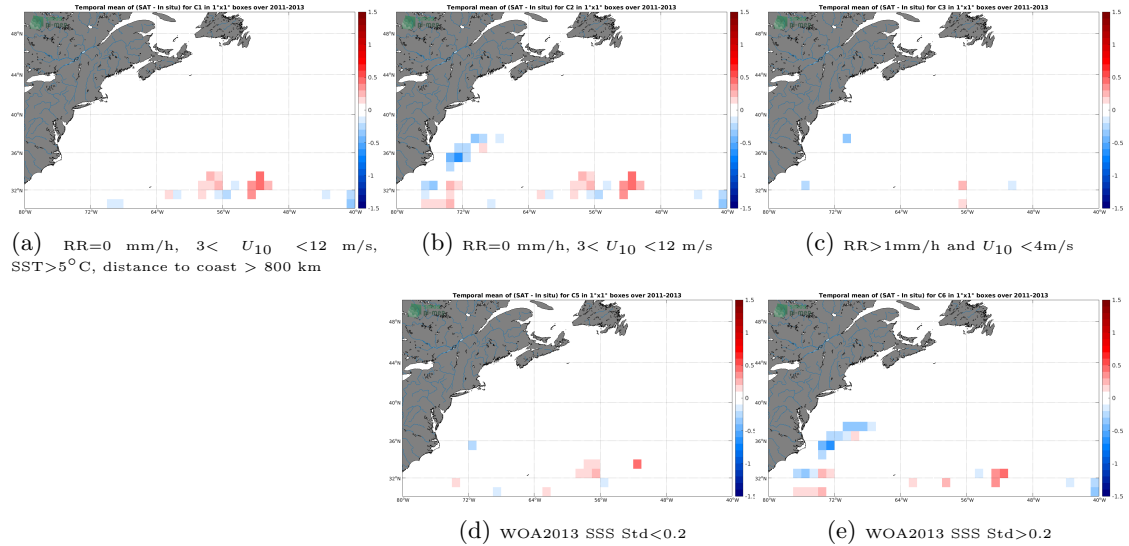
Figure 11: Temporal mean gridded over spatial boxes of size 1^{\circ}\times 1^{\circ} of \Delta\text{SSS} (Aquarius SSS L4 OI v5 - Monthly (IPRC) - Surface drifters) for 5 different subdatasets corresponding to:RR=0 mm/h, 3 < U_{10} < 12 m/s, SST >5^{\circ}\text{C} , distance to coast > 800 km (a), RR=0 mm/h, 3 < U_{10} < 12 m/s (b), RR >1 mm/h and U_{10} < 4 m/s (c), WOA2013 SSS Std <0.2 (d), WOA2013 SSS Std >0.2 (e).
