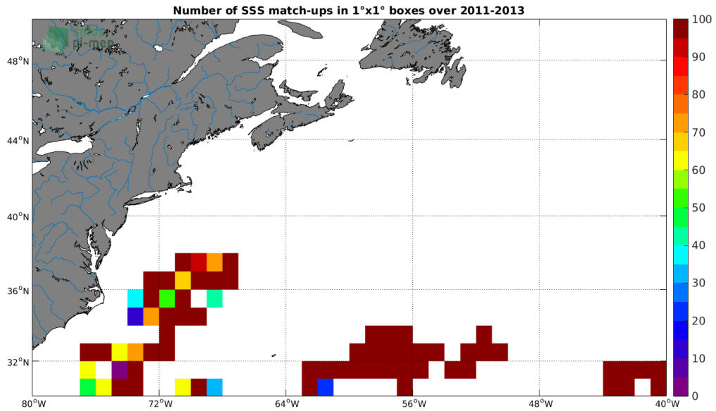
Figure 3: Number of SSS match-ups between Surface drifters SSS and the Aquarius-L4-IPRC-V5-MONTHLY SSS product for the Gulf Stream Pi-MEP region over 1°x1° boxes and for the full satellite product period.
