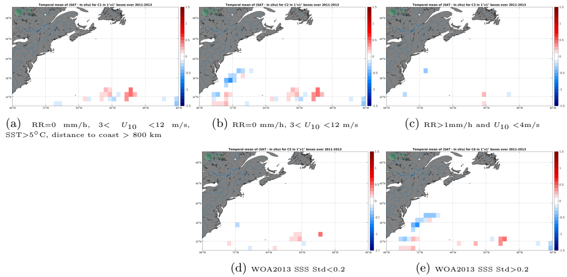
Figure 11: Temporal mean gridded over spatial boxes of size 1^\circ \times 1^\circ of \Delta SSS (Aquarius-L4-IPRC-V5-MONTHLY - Surface drifters) for 5 different subdatasets corresponding to:RR=0 mm/h, 3 < U_{10} < 12 m/s, SST >5^\circ C, distance to coast > 800 km (a), RR=0 mm/h, 3 < U_{10} < 12 m/s (b), RR >1 mm/h and U_{10} < 4 m/s (c), WOA2013 SSS Std <0.2 (d), WOA2013 SSS Std >0.2 (e).
