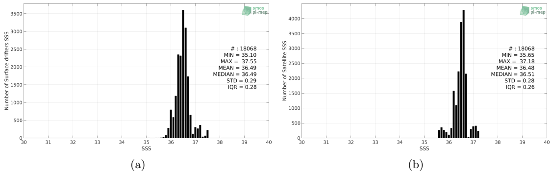
Figure 2: Histograms of SSS from Surface drifters (a) and Aquarius-L4-IPRC-V5-MONTHLY (b) considering all match-up pairs per bins of 0.1 over the Gulf Stream Pi-MEP region and for the full satellite product period.
