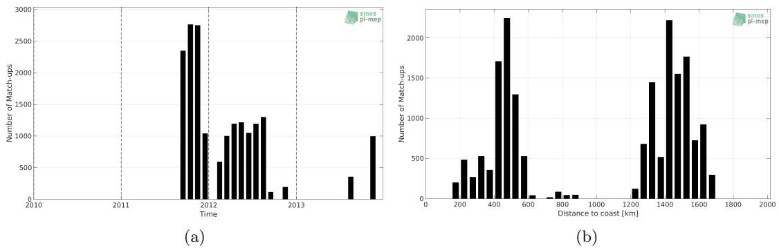
Figure 1: Number of match-ups between Surface drifters and Aquarius-L4-IPRC-V5-MONTHLY SSS as a function of time (a) and as function of the distance to coast (b) over the Gulf Stream Pi-MEP region and for the full satellite product period.
