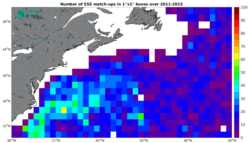
Figure 4: Number of SSS match-ups between Argo SSS and the Aquarius SSS L4 OI v5 - Monthly (IPRC) SSS product for the Gulf Stream Pi-MEP region over 1^{\circ} \times 1^{\circ} boxes and for the full satellite product period.
