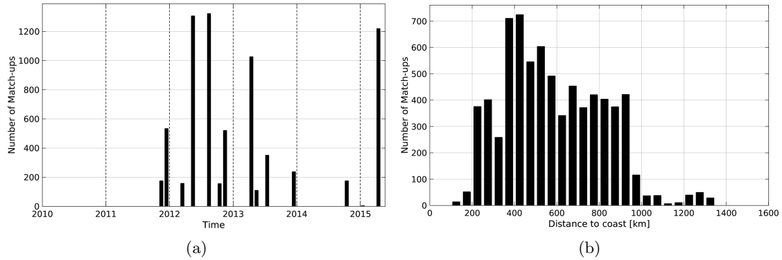
Figure 1: Number of match-ups between TSG-LEGOS-DM and Aquarius-L4-IPRC-V4-WEEKLY SSS as a function of time (a) and as function of the distance to coast (b) over the Gulf Stream Pi-MEP region and for the full satellite product period.
