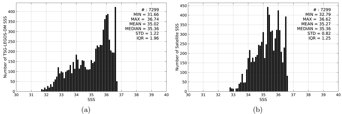
Figure 2: Histograms of SSS from TSG-LEGOS-DM (a) and Aquarius-L4-IPRC-V4-WEEKLY (b) considering all match-up pairs per bins of 0.1 over the Gulf Stream Pi-MEP region and for the full satellite product period.
