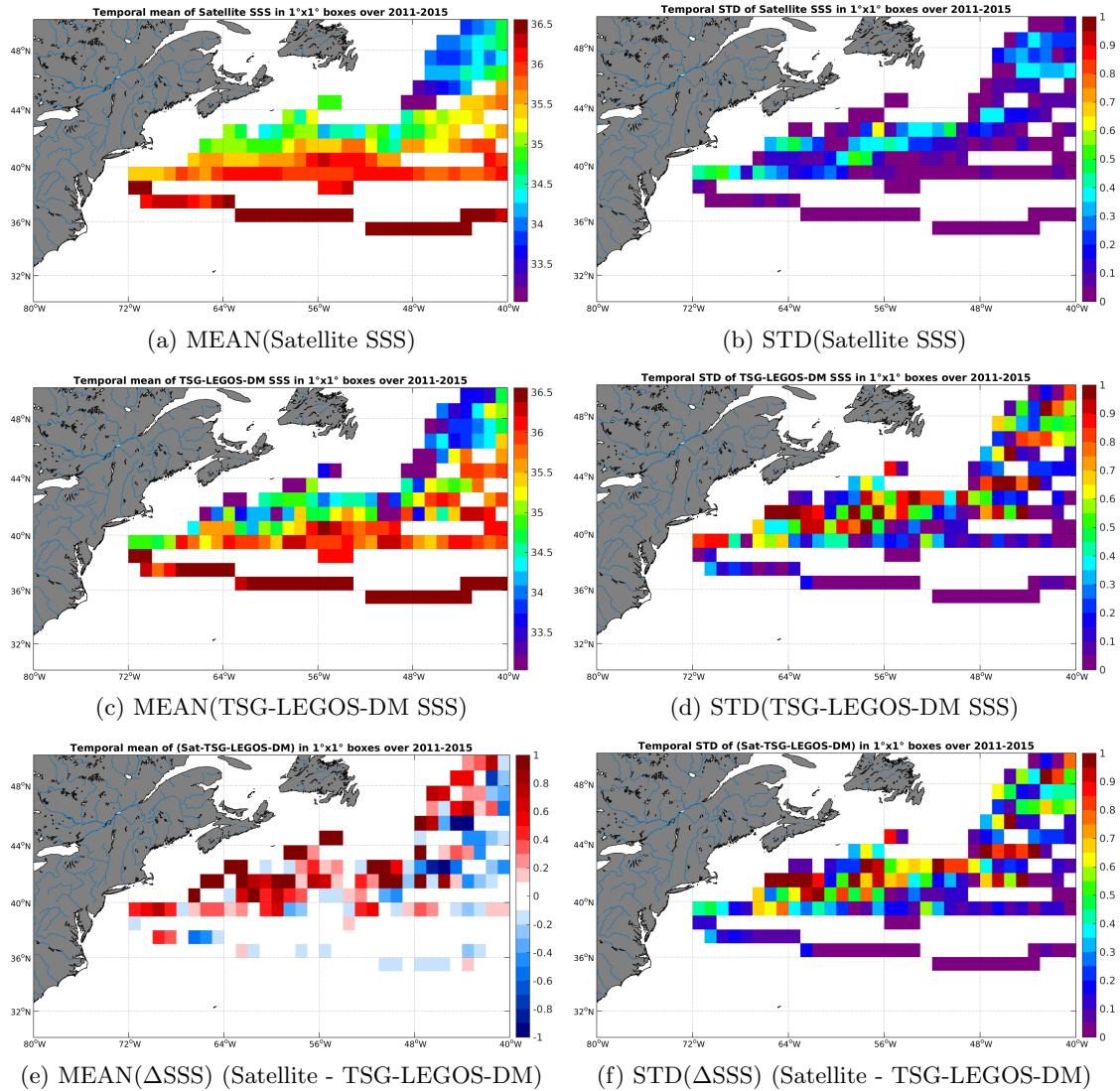
Figure 6: Temporal mean (left) and STD (right) of SSS from Aquarius-L4-IPRC-V4-WEEKLY (top), TSG-LEGOS-DM (middle), and of \Delta SSS (Satellite - TSG-LEGOS-DM). Only match-up pairs are used to generate these maps.
