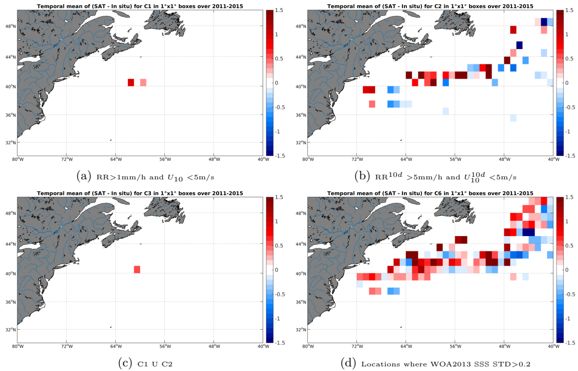
Figure 12: Temporal mean gridded over spatial boxes of size 1^\circ \times 1^\circ of \Delta SSS (Aquarius-L4-IPRC-V4-WEEKLY - TSG-LEGOS-DM) for 4 different subdatasets corresponding to: RR > 1mm/h and U_{10} < 5\text{m/s} (a), RR^{10d} > 5\text{mm/h} and U_{10}^{10d} < 5\text{m/s} (b), C1 U C2 (c), Locations where WOA2013 SSS STD > 0.2 (d).
