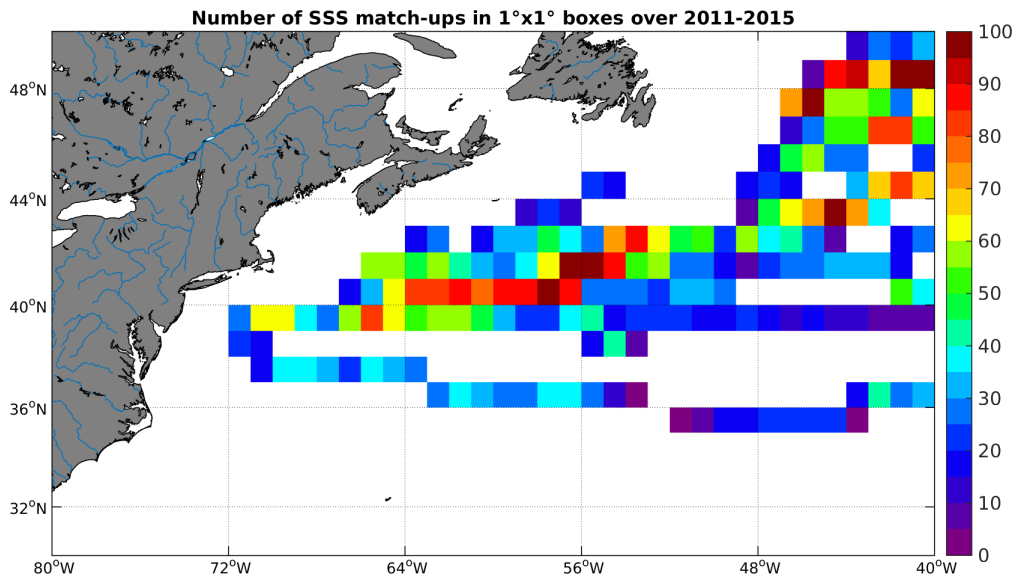
Figure 4: Number of SSS match-ups between TSG-LEGOS-DM SSS and the Aquarius-L4-IPRC-V4-WEEKLY SSS product for the Gulf Stream Pi-MEP region over 1^\circ \times 1^\circ boxes and for the full satellite product period.
