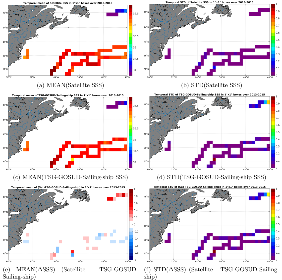
Figure 6: Temporal mean (left) and STD (right) of SSS from Aquarius-L4-IPRC-V4-WEEKLY (top), TSG-GOSUD-Sailing-ship (middle), and of \Delta SSS (Satellite - TSG-GOSUD-Sailing-ship). Only match-up pairs are used to generate these maps.
