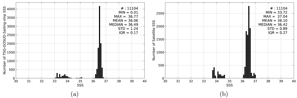
Figure 2: Histograms of SSS from TSG-GOSUD-Sailing-ship (a) and Aquarius-L4-IPRC-V4-WEEKLY (b) considering all match-up pairs per bins of 0.1 over the Gulf Stream Pi-MEP region and for the full satellite product period.
