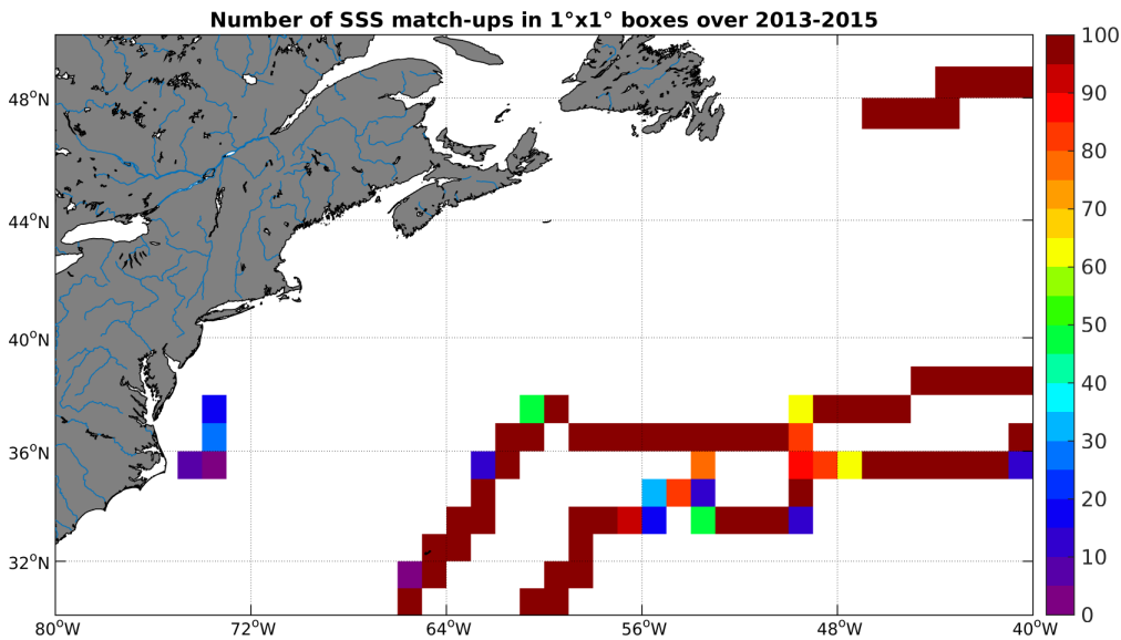
Figure 4: Number of SSS match-ups between TSG-GOSUD-Sailing-ship SSS and the Aquarius-L4-IPRC-V4-WEEKLY SSS product for the Gulf Stream Pi-MEP region over 1^\circ \times 1^\circ boxes and for the full satellite product period.
