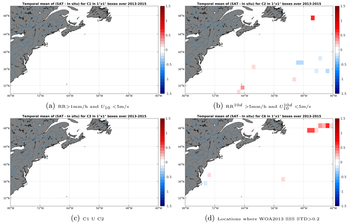
Figure 12: Temporal mean gridded over spatial boxes of size 1^\circ \times 1^\circ of \Delta SSS (Aquarius-L4-IPRC-V4-WEEKLY - TSG-GOSUD-Sailing-ship) for 4 different subdatasets corresponding to: RR > 1\text{mm/h} and U_{10} < 5\text{m/s} (a), RR^{10d} > 5\text{mm/h} and U_{10}^{10d} < 5\text{m/s} (b), C1 U C2 (c), Locations where WOA2013 SSS STD > 0.2 (d).
