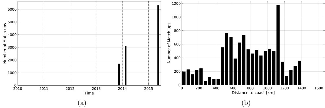
Figure 1: Number of match-ups between TSG-GOSUD-Sailing-ship and Aquarius-L4-IPRC-V4-WEEKLY SSS as a function of time (a) and as function of the distance to coast (b) over the Gulf Stream Pi-MEP region and for the full satellite product period.
