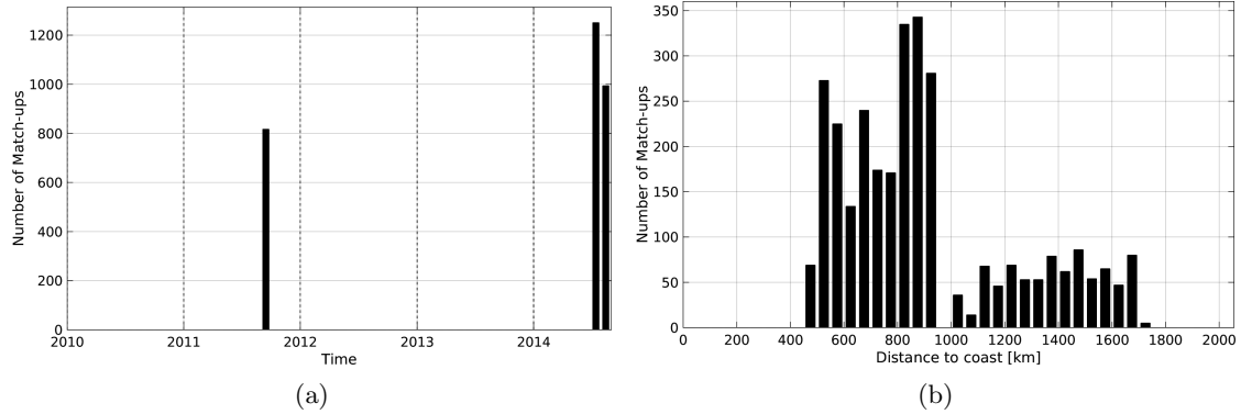
Figure 1: Number of match-ups between TSG-GOSUD-Research-vessel and Aquarius-L4-IPRC-V4-WEEKLY SSS as a function of time (a) and as function of the distance to coast (b) over the Gulf Stream Pi-MEP region and for the full satellite product period.
