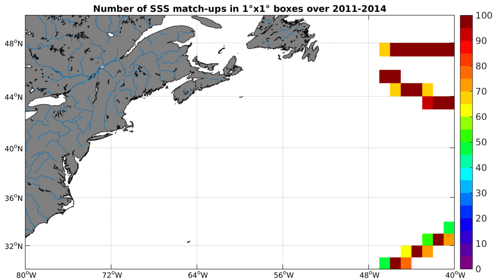
Figure 4: Number of SSS match-ups between TSG-GOSUD-Research-vessel SSS and the Aquarius-L4-IPRC-V4-WEEKLY SSS product for the Gulf Stream Pi-MEP region over 1^\circ \times 1^\circ boxes and for the full satellite product period.
