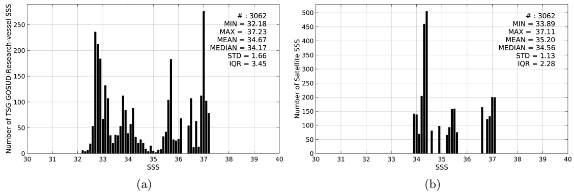
Figure 2: Histograms of SSS from TSG-GOSUD-Research-vessel (a) and Aquarius-L4-IPRC-V4-WEEKLY (b) considering all match-up pairs per bins of 0.1 over the Gulf Stream Pi-MEP region and for the full satellite product period.
