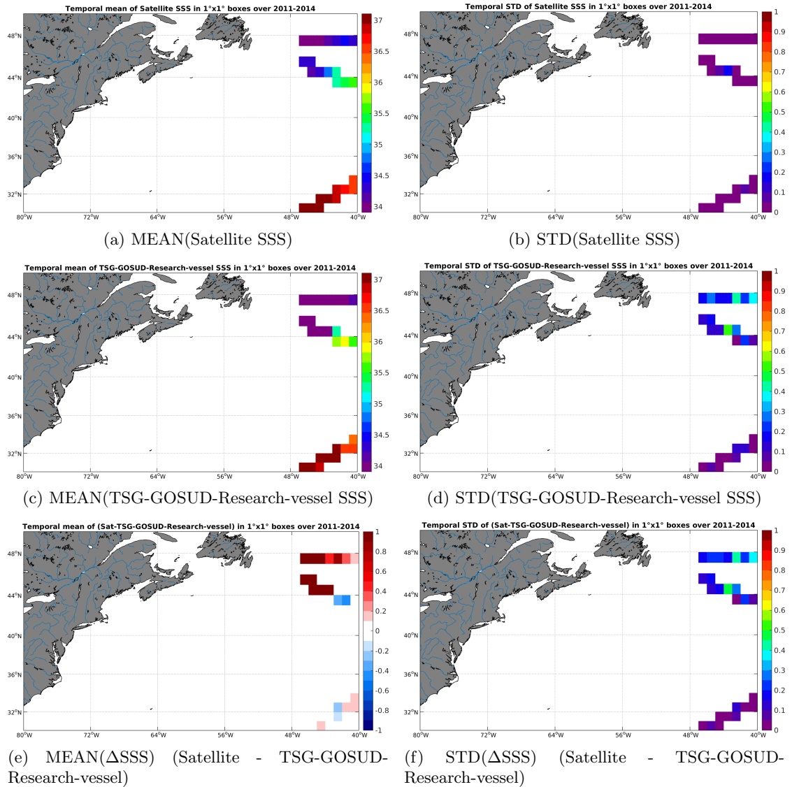
Figure 6: Temporal mean (left) and STD (right) of SSS from Aquarius-L4-IPRC-V4-WEEKLY (top), TSG-GOSUD-Research-vessel (middle), and of \Delta SSS (Satellite - TSG-GOSUD-Research-vessel). Only match-up pairs are used to generate these maps.
