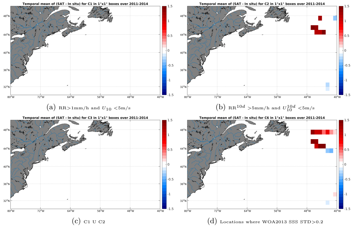
Figure 12: Temporal mean gridded over spatial boxes of size 1°x1° of \Delta SSS (Aquarius-L4-IPRC-V4-WEEKLY - TSG-GOSUD-Research-vessel) for 4 different subdatasets corresponding to: RR > 1mm/h and U_{10} < 5\text{m/s} (a), RR^{10d} > 5\text{mm/h} and U_{10}^{10d} < 5\text{m/s} (b), C1 U C2 (c), Locations where WOA2013 SSS STD > 0.2 (d).
