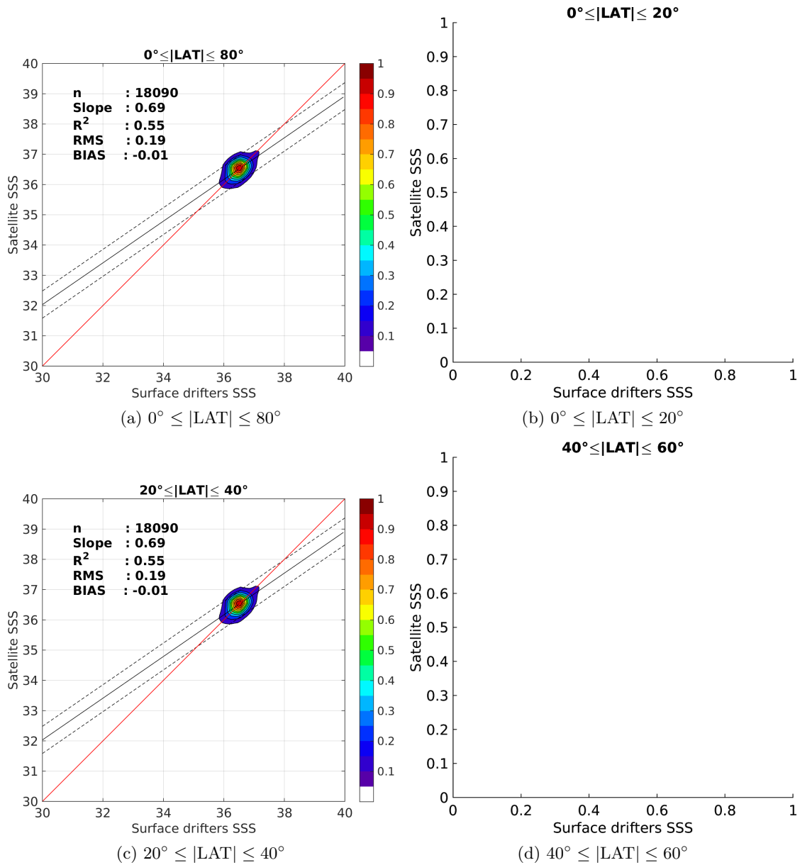
Figure 8: Contour maps of the concentration of Aquarius-L4-IPRC-V4-WEEKLY SSS (y-axis) versus Surface drifters SSS (x-axis) at match-up pairs for different latitude bands. For each plot, the red line shows x=y . The black thin and dashed lines indicate a linear fit through the data cloud and the \pm 95\% confidence levels, respectively. The number match-up pairs n , the slope and R^2 coefficient of the linear fit, the root mean square (RMS) and the mean bias between satellite and in situ data are indicated for each latitude band in each plots.
