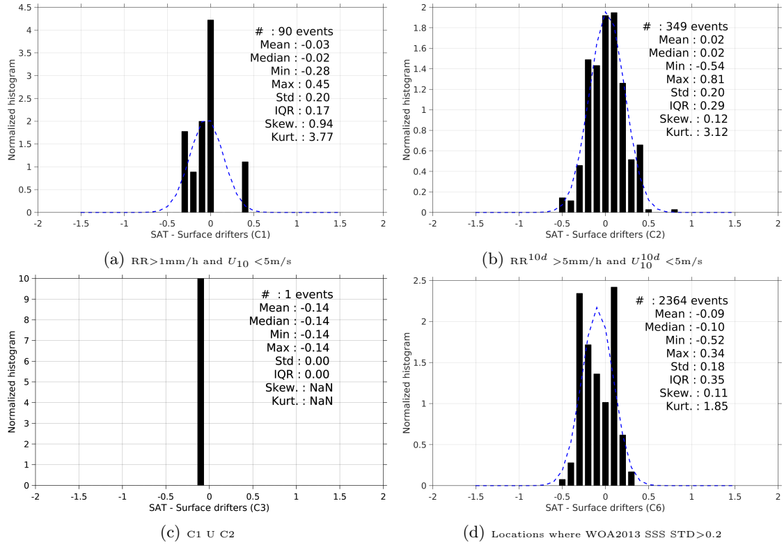
Figure 12: Normalized histogram of \Delta\text{SSS} (Aquarius-L4-IPRC-V4-WEEKLY - Surface drifters) for 6 different subdatasets corresponding to: RR > 1\text{mm/h} and U_{10} < 5\text{m/s} (a), RR^{10d} > 5\text{mm/h} and U_{10}^{10d} < 5\text{m/s} (b), C1 U C2 (c), Locations where WOA2013 SSS STD > 0.2 (d).
