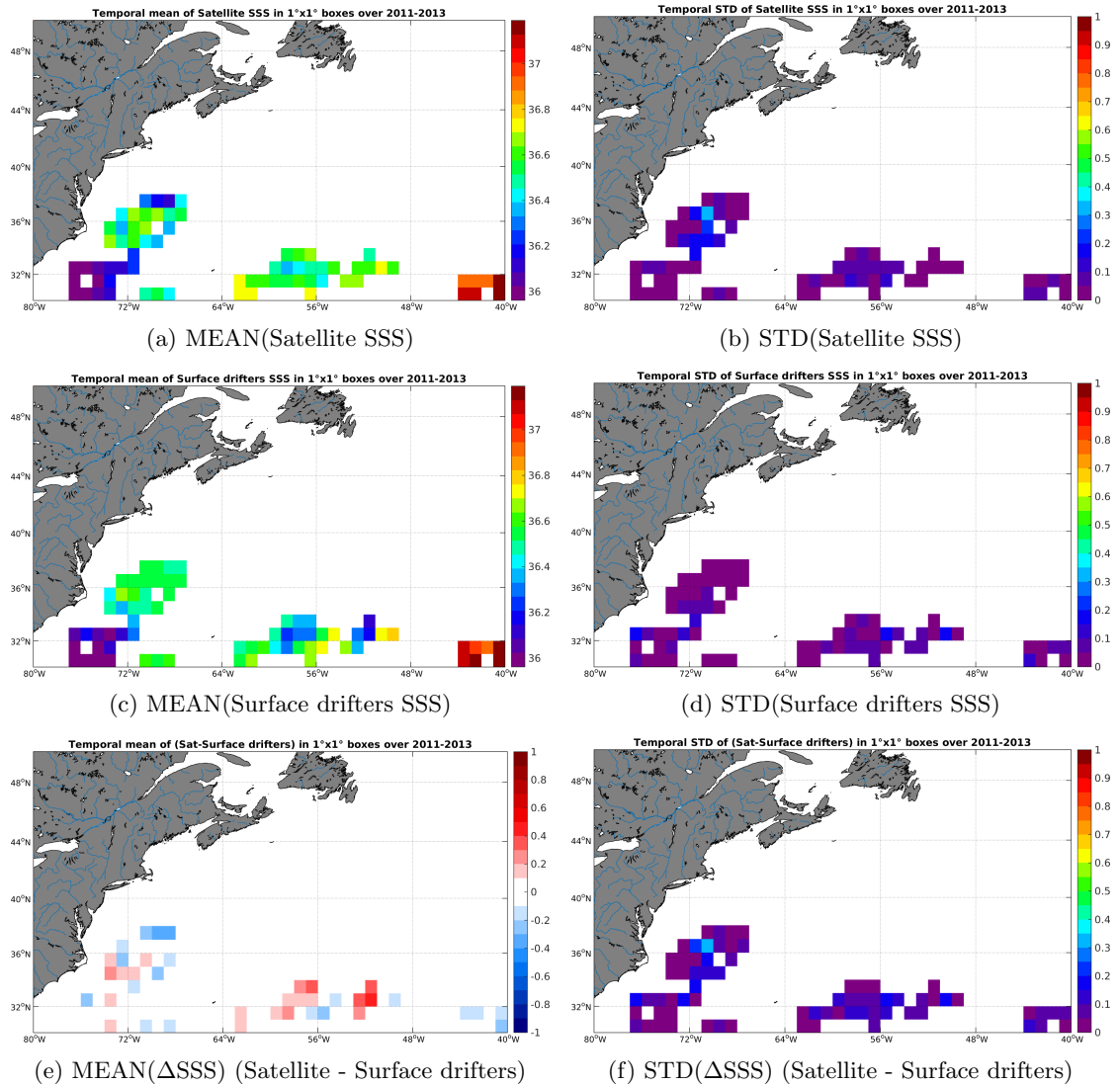
Figure 5: Temporal mean (left) and STD (right) of SSS from Aquarius-L4-IPRC-V4-WEEKLY (top), Surface drifters (middle), and of \Delta SSS (Satellite - Surface drifters). Only match-up pairs are used to generate these maps.
