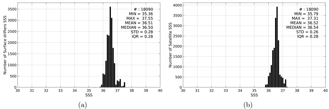
Figure 2: Histograms of SSS from Surface drifters (a) and Aquarius-L4-IPRC-V4-WEEKLY (b) considering all match-up pairs per bins of 0.1 over the Gulf Stream Pi-MEP region and for the full satellite product period.
