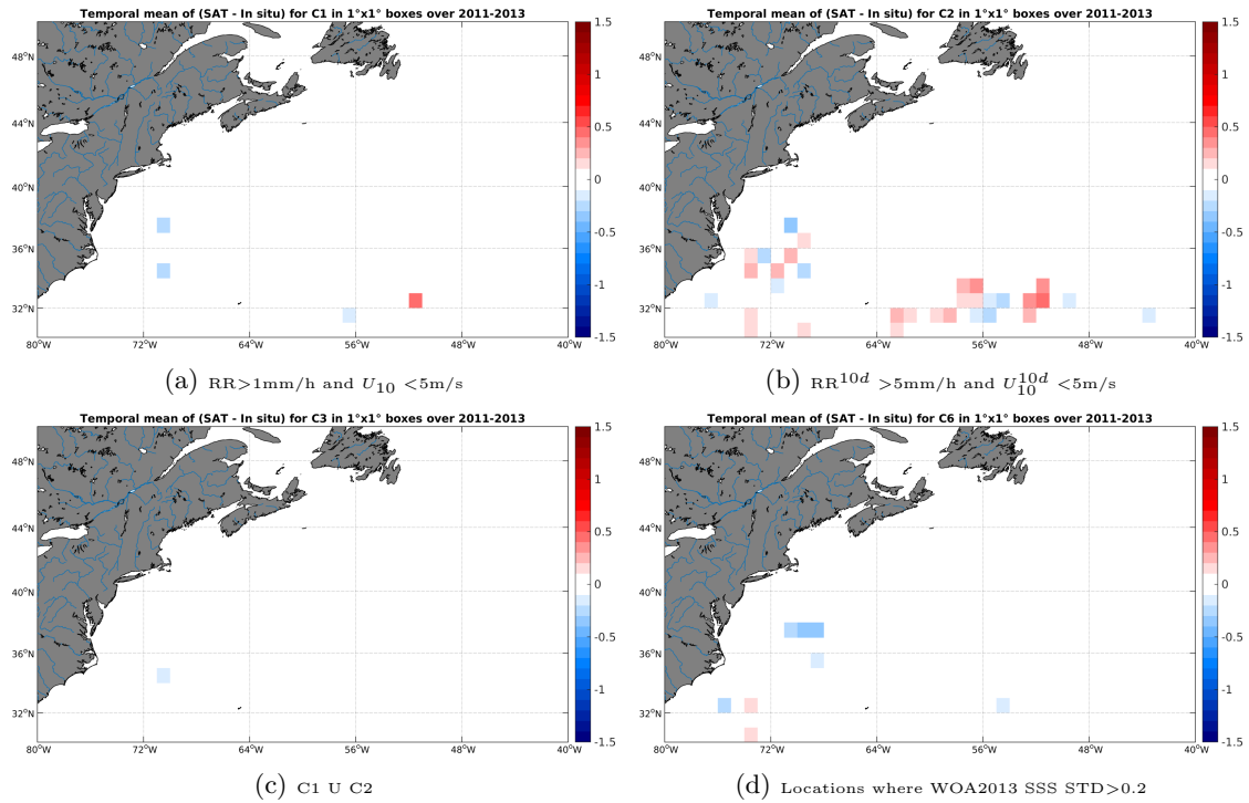
Figure 11: Temporal mean gridded over spatial boxes of size 1^\circ \times 1^\circ of \Delta SSS (Aquarius-L4-IPRC-V4-WEEKLY - Surface drifters) for 4 different subdatasets corresponding to: RR > 1mm/h and U_{10} < 5 m/s (a), RR^{10d} > 5 mm/h and U_{10}^{10d} < 5 m/s (b), C1 U C2 (c), Locations where WOA2013 SSS STD > 0.2 (d).
