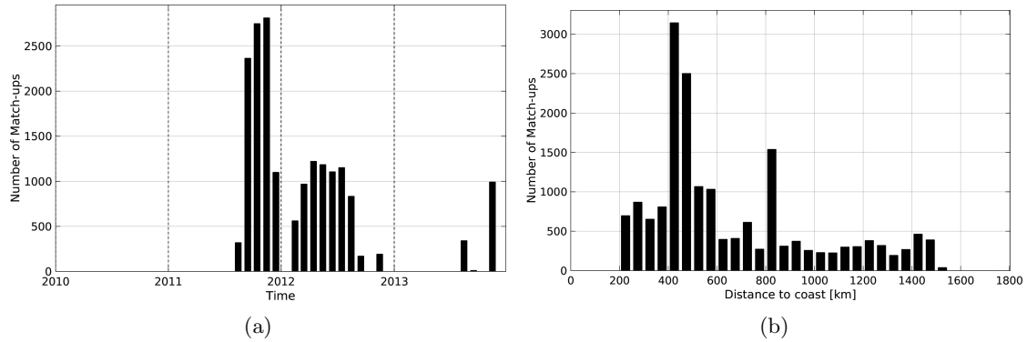
Figure 1: Number of match-ups between Surface drifters and Aquarius-L4-IPRC-V4-WEEKLY SSS as a function of time (a) and as function of the distance to coast (b) over the Gulf Stream Pi-MEP region and for the full satellite product period.
