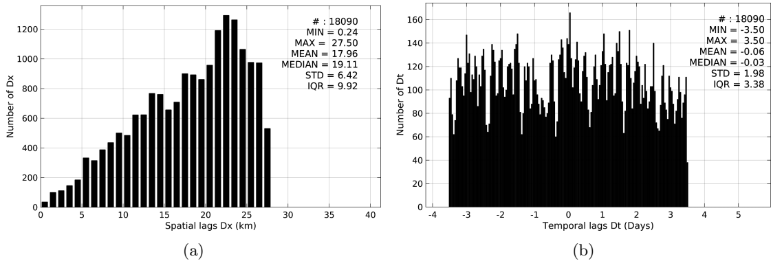
Figure 4: Histograms of the spatial (a) and temporal (b) lags between the time of the Surface drifters measurements and the date of the corresponding Aquarius-L4-IPRC-V4-WEEKLY SSS product.
