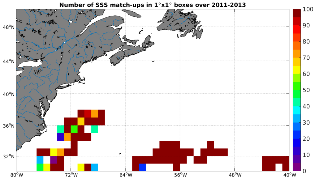
Figure 3: Number of SSS match-ups between Surface drifters SSS and the Aquarius-L4-IPRC-V4-WEEKLY SSS product for the Gulf Stream Pi-MEP region over 1°x1° boxes and for the full satellite product period.
