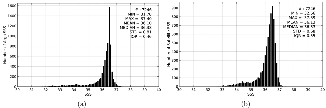
Figure 2: Histograms of SSS from Argo (a) and Aquarius-L4-IPRC-V4-WEEKLY (b) considering all match-up pairs per bins of 0.1 over the Gulf Stream Pi-MEP region and for the full satellite product period.
