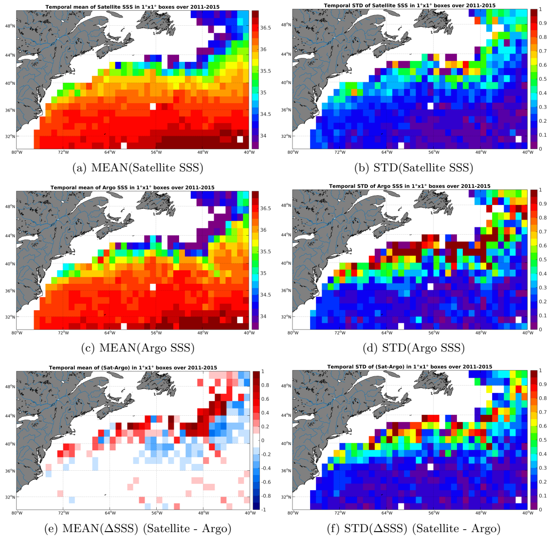
Figure 6: Temporal mean (left) and STD (right) of SSS from Aquarius-L4-IPRC-V4-WEEKLY (top), Argo (middle), and of \Delta SSS (Satellite - Argo). Only match-up pairs are used to generate these maps.
