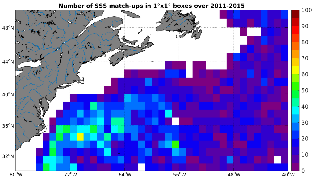
Figure 4: Number of SSS match-ups between Argo SSS and the Aquarius-L4-IPRC-V4-WEEKLY SSS product for the Gulf Stream Pi-MEP region over 1°x1° boxes and for the full satellite product period.
