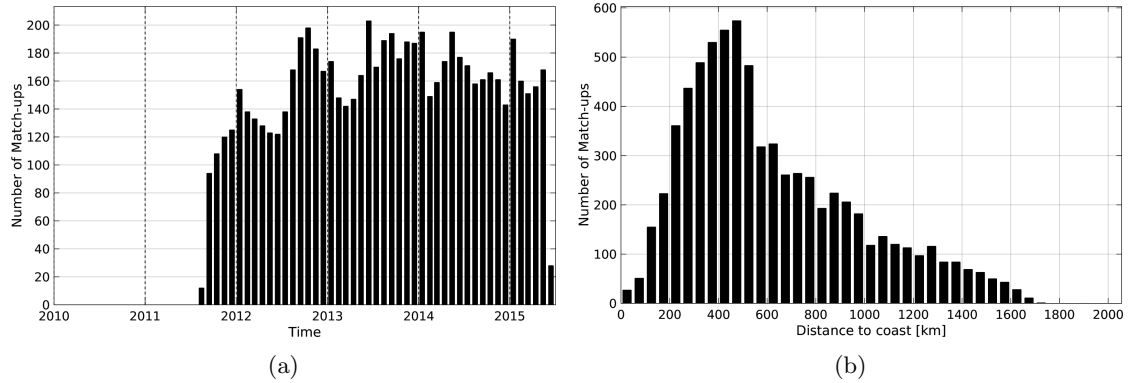
Figure 1: Number of match-ups between Argo and Aquarius-L4-IPRC-V4-WEEKLY SSS as a function of time (a) and as function of the distance to coast (b) over the Gulf Stream Pi-MEP region and for the full satellite product period.
