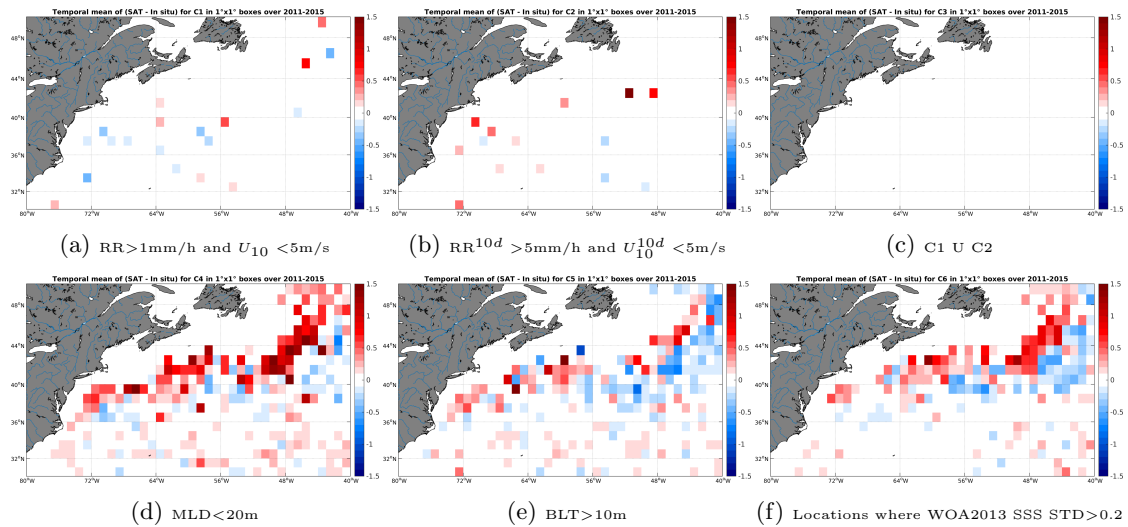
Figure 12: Temporal mean gridded over spatial boxes of size 1^\circ \times 1^\circ of \Delta SSS (Aquarius-L4-IPRC-V4-WEEKLY - Argo) for 6 different subdatasets corresponding to:RR>1mm/h and U_{10} < 5\text{m/s} (a), RR^{10d} > 5\text{mm/h} and U_{10}^{10d} < 5\text{m/s} (b), C1 U C2 (c),MLD<20m (d),BLT>10m (e),Locations where WOA2013 SSS STD>0.2 (f).
