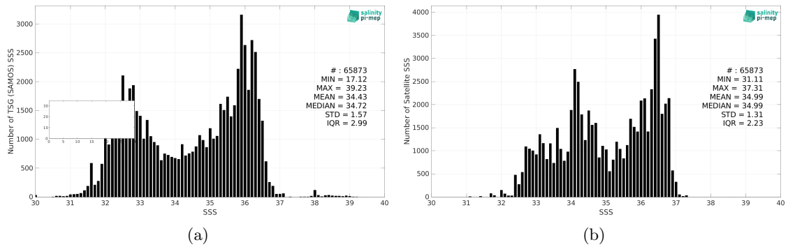
Figure 2: Histograms of SSS from TSG (SAMOS) (a) and Aquarius SSS L3 CAP v5 - 7-Day running (JPL) (b) considering all match-up pairs per bins of 0.1 over the Gulf Stream Pi-MEP region and for the full satellite product period.
