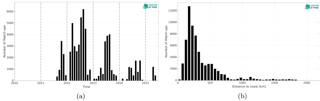
Figure 1: Number of match-ups between TSG (SAMOS) and Aquarius SSS L3 CAP v5 - 7-Day running (JPL) SSS as a function of time (a) and as function of the distance to coast (b) over the Gulf Stream Pi-MEP region and for the full satellite product period.
